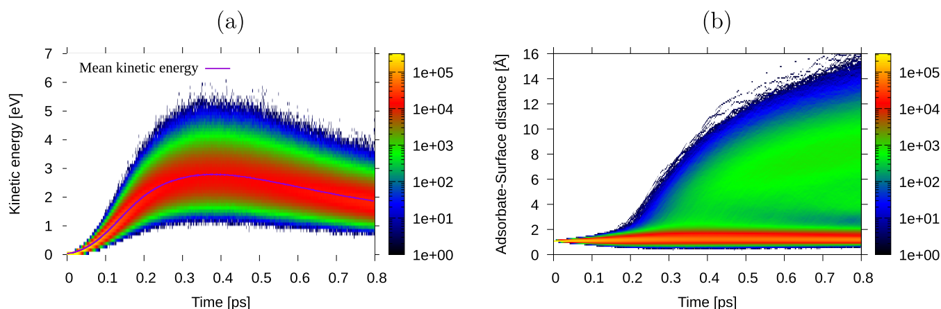
Figure 5. Histograms of the kinetic energy (a) and H-surface distance (b) over 20,000 trajectories with a laser fluence of 60 J/m 2 . Color bar corresponds to the number of H atoms with a given kinetic energy or distance from the surface.
