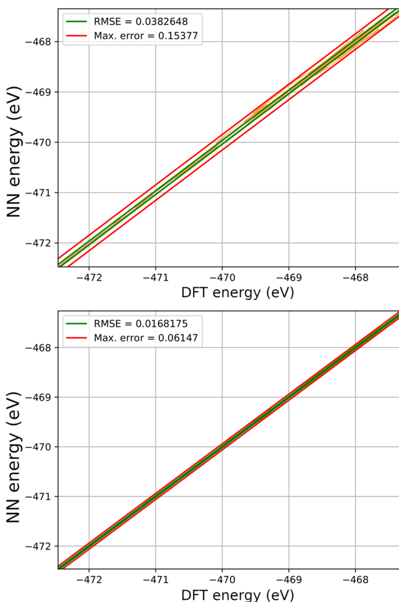
Figure 1. Comparison of DFT energies and neural network (NN) potential. Top panel: NN trained on the initial data set. Bottom panel: NN trained on the final data set. Red (green) lines are offset \pm maximum error (RMSE) from perfect y = x line for which NN would predict exactly the same energy as DFT.
