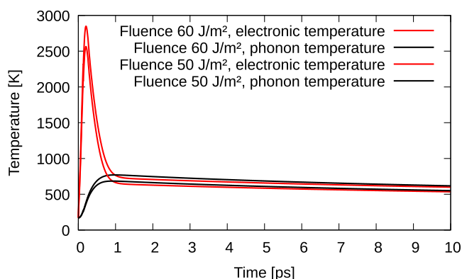
Figure 4. Electronic and phonon temperatures upon laser excitation of the Ru(0001) surface, calculated in the 2TM. Two different Gaussian pulses with FWHM = 130 fs and wavelength = 800 nm but different fluences have been used. Pulse maximum is at t = 0.13 \text{ ps} . The same material properties have been fed into the 2TM as in ref 17, and the same initial temperature (170 K).
