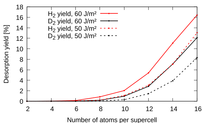
Figure 9. Yield as a function of coverage for (4 \times 4) unit cell with 16 adsorption sites, for \text{H}_2 and \text{D}_2 and two different fluences.
