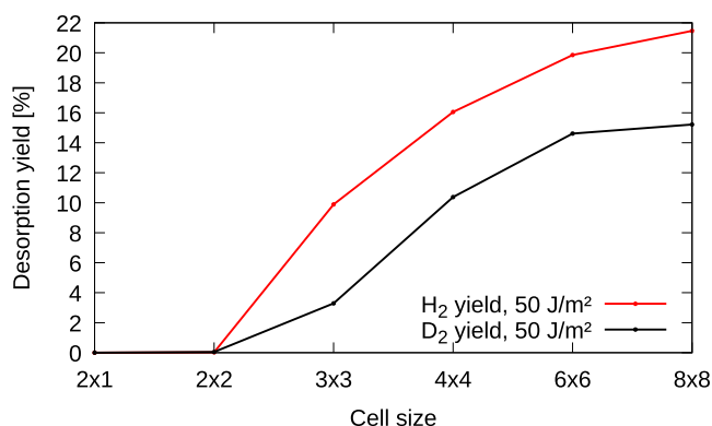
Figure 10. \text{H}_2 and \text{D}_2 desorption yields as a function of cell size, for 1 ML of adsorbates (coverage = 1), and a fluence of 50 \text{ J/m}^2 .
