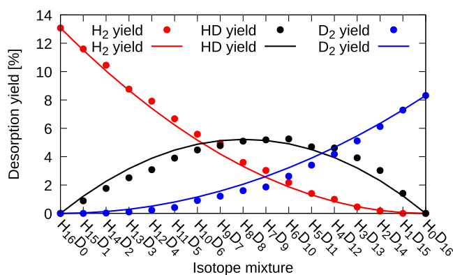
Figure 7. Desorption yield of H 2 , HD, and D 2 for different isotope mixtures for the laser fluence of 50 J/m 2 . Symbols are from the Langevin trajectories, solid lines from idealized second-order rate models (see text and ref 17).
