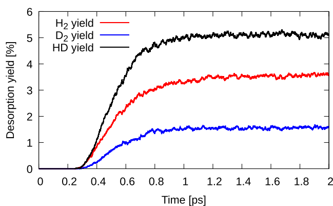
Figure 6. Desorption yield of H 2 , HD, and D 2 for randomly placed H 8 D 8 isotope mixture as a function of integration time for the laser fluence of 50 J/m 2 .
