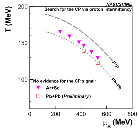
Fig. 21 Diagram of chemical freeze-out temperature and baryon-chemical potential. The dashed line indicates parameters in p+p interactions and the dotted line in the central Pb+Pb collisions; points estimated and extrapolated ( \mu_B for p+p ) based on Ref. [52]. The colored points mark reactions (Ar+Sc and Pb+Pb [53]) in the T - \mu_B phase diagram for which the search for the critical point was conducted, and no evidence for the critical point was found
