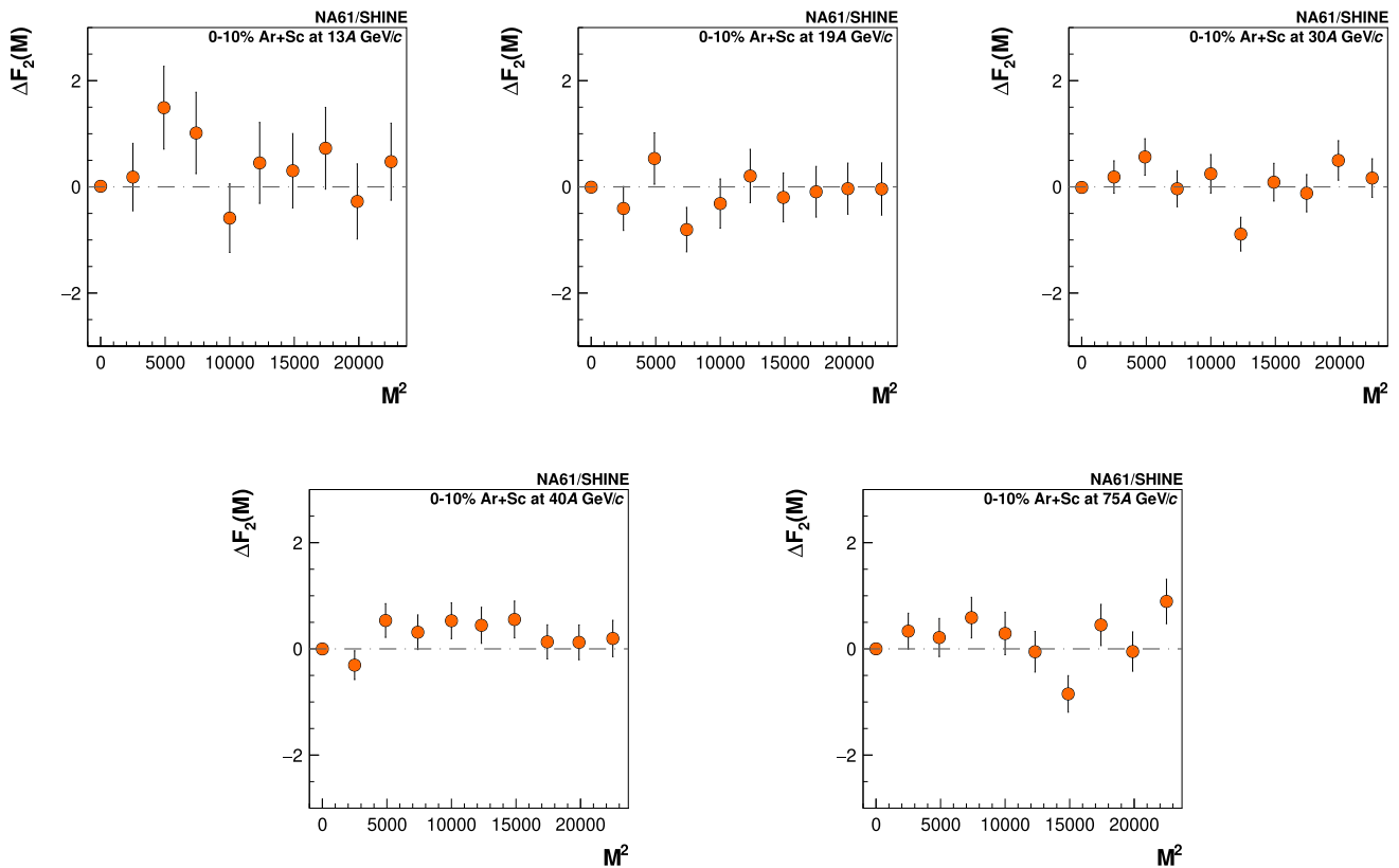
Fig. 12 Results on the dependence of \Delta F_2(M) of proton multiplicity distribution on the number of subdivisions in transverse momentum space M^2 for 1^2 \leq M^2 \leq 150^2 . Results for 0–10% central ^{40}\text{Ar} + ^{45}\text{Sc}
