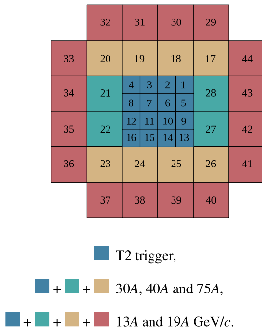
Fig. 3 Event centrality selection using the PSD energy. Modules used in the centrality class determination were chosen based on the anti-correlation between the measured energy and the track multiplicity in a given event. All modules were used for 13A and 19A GeV/c. For 30A, 40A, and 75A GeV/c 28 central modules were chosen. For the T2 trigger, 16 central modules were used
