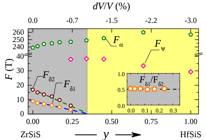
FIG. 2. Phase diagram of QO frequency vs Hf concentration y in Zr_{1-y}Hf_ySiS along the crystallographic [001] direction. Two Lifshitz transitions in the low-frequency spectrum are identified: A new pocket with frequency F_{\psi} emerges at around y = 0.24 , and an electron pocket with frequency F_{\delta 1} ( F_{\delta 2} ) vanishes at y \approx 0.34 (as estimated from linear interpolations - green and blue dashed lines, respectively). Clearly, the low-frequency QOs seen in [001] direction for ZrSiS and HfSiS are topologically not connected. On the other hand the hole-pocket frequency F_{\alpha} increases with y and is continuously connected between y = 0 and y = 1 . The inset shows the ratio of the frequencies F_{\delta 1}/F_{\delta 2} which does not change with y . The dashed lines are guide to the eye.
