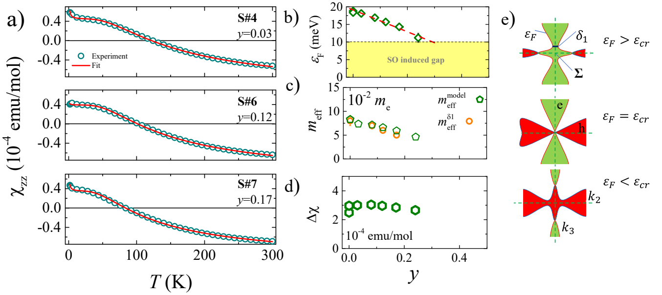
FIG. 3. a) Fit of Eq.(2) to experimental \chi_{zz}(T) for samples y = 0.03, 0.12 and 0.17 including localized paramagnetic impurity contributions responsible for the low- T upturn. The model fairly well captures the experimental data in the whole measured T -range. b) Fermi energy ( E_F ) measured from the nodal-line crossing point as a function of y . Below \approx 10 meV our model breaks down due to the SO-interaction induced gap at the nodal line. c) Effective mass m_{\text{eff}}^{\delta 1} as estimated from QO of the \delta 1 orbital compared with the effective mass m_{\text{eff}}^{\text{model}} as a function of y . d) Almost constant value of \Delta\chi from Eq.(2) as a function of y indicates that the FS around the crossing points is not strongly modified for low levels of y . e) Schematic drawing of the Fermi surface with self-intersecting orbitals near the degeneracy point \Sigma based on the model Eq.(1) (parameters B_1 = -B_2 and \lambda < 0 ). By tuning the Fermi energy the system undergoes a nonstandard Lifshitz transition characterized by a change in the configuration of the e-h pockets and direction of the intersecting orbitals.
