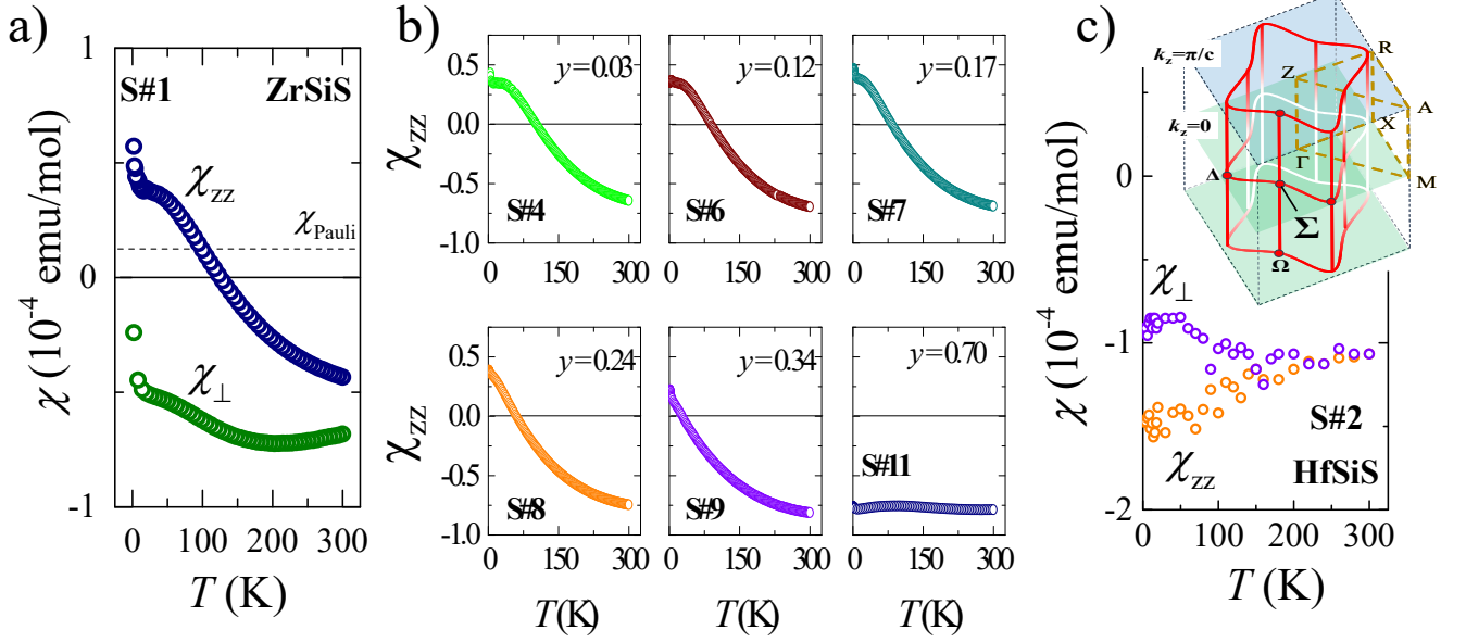
FIG. 1. Temperature ( T ) dependent magnetic susceptibility of \text{Zr}_{1-y}\text{Hf}_y\text{SiS} taken at 1T for various Hf concentrations y . a) Out-of-plane \chi_{zz} , along [001], and in-plane \chi_{\perp} susceptibility of \text{ZrSiS} . \chi_{zz} has a strong anomalous T dependence with unexpected change in the susceptibility from diamagnetic at high T to paramagnetic at low T . By contrast \chi_{\perp} exhibits a weak T dependence with an impurity tail at low T . \chi_{\text{Pauli}} (dashed line) indicates the free-electron Pauli paramagnetic contribution as estimated from the specific heat measurements. b) \chi_{zz} for different y : Upon increasing chemical pressure the sign change in \chi_{zz} shifts toward lower T . For y > 0.24 the low- T saturation of \chi_{zz} vanishes. At high doping y = 0.7 , \chi_{zz} flattens and remains diamagnetic in the whole T range examined. c) \chi_{zz} and \chi_{\perp} for \text{HfSiS} exhibit a conventional, almost isotropic and weak T dependence. (Inset) Schematics of the cage of nodal lines in the 1st Brillouin zone. The intersecting nodal-line of interest \Sigma is located along the \Gamma - M direction.
