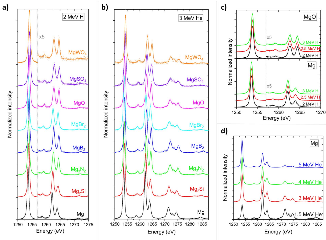
Fig. 3 Fitted K\alpha X-ray emission spectra of Mg and its selected compounds excited by (a) 2 MeV H and (b) 3 MeV He. (c) Fitted K\alpha X-ray emission spectra of Mg and MgO excited by H beam at three different energies: 2, 2.5 and 3 MeV. (d) Fitted K\alpha X-ray emission spectra of Mg excited by He beam at four different energies: 1.5, 3, 4 and 5 MeV. The intensities of spectral regions containing MIS lines in (a) and (c) are multiplied by a factor of 5 for plotting purposes. All spectra are normalized to their maximum intensity.
