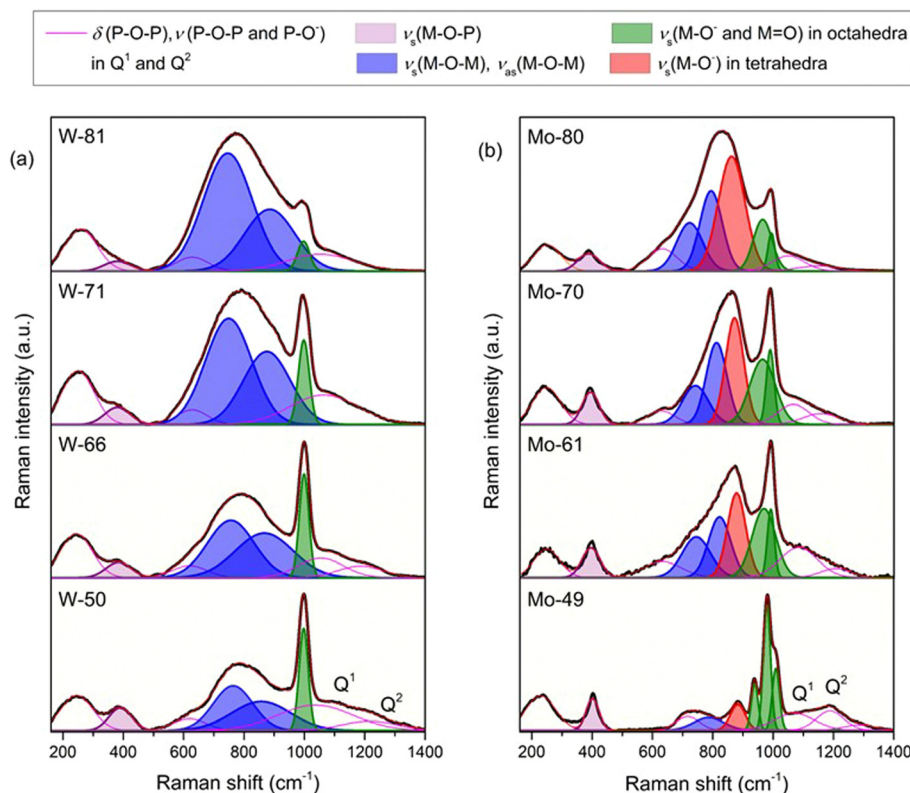
Fig. 1 Raman spectra of glasses from (a) x\text{WO}_3-(100-x)\text{P}_2\text{O}_5 and (b) x\text{MoO}_3-(100-x)\text{P}_2\text{O}_5 , x = 49-81 mol%, series. The Raman spectra of W-61 and Mo-57 are similar to those of W-66 and Mo-61, respectively; hence, they are not shown.
