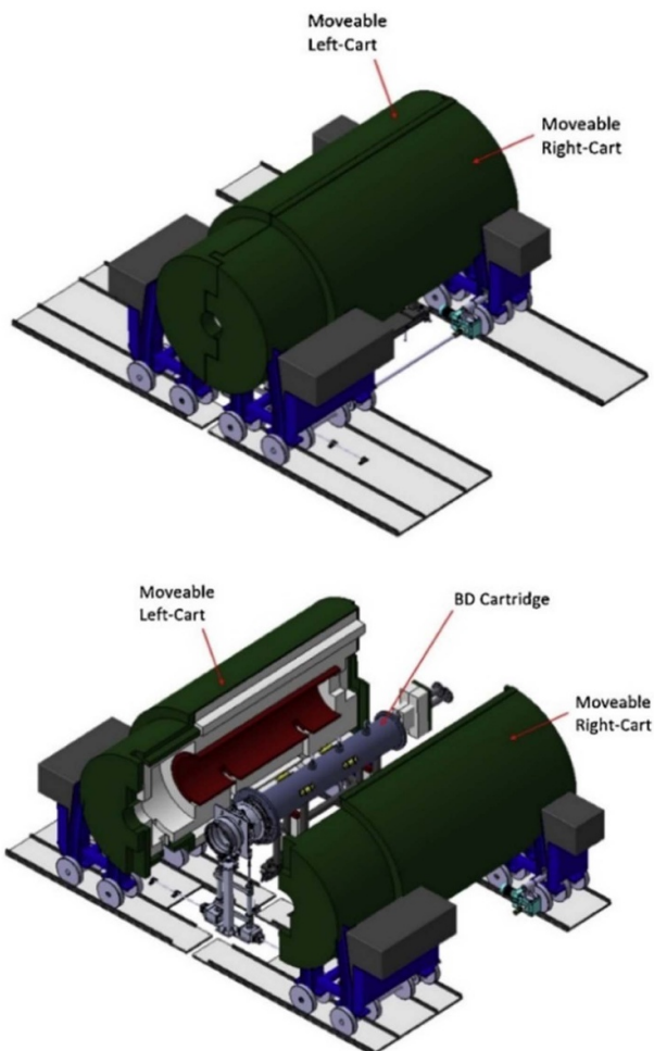
Figure 16. BD module structure. Reprinted from [13], Copyright (2020), with permission from Elsevier.
