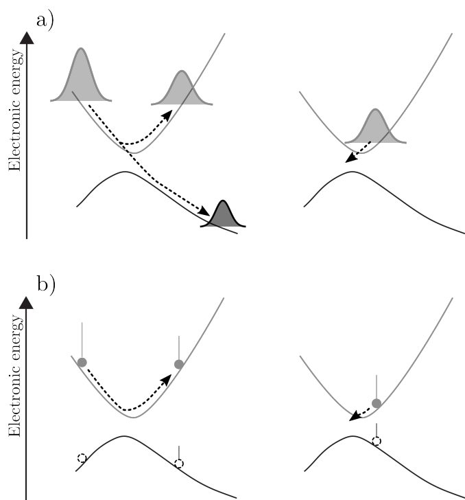
Figure 6. Schematic representation of a first branching of a nuclear wavepacket following a nonadiabatic region (left), followed by a second crossing event (right) in (a) quantum dynamics and (b) TSH. The right panel highlights the overcoherence issue of TSH in its original flavour. In panel (b), the trajectory that drives the TSH dynamics is given as a filled circle (the scenario here is that the driving trajectory remains in the upper electronic state). The dashed circle indicates a 'ghost' trajectory that follows the driving trajectory and is meant to highlight the dynamics of the electronic coefficients. The magnitude of the electronic coefficient in each electronic state is symbolized by the vertical bar on top of the circles: long bar for the upper electronic state at the beginning of the dynamics (the electronic coefficient is set to 1 for this state, 0 for the other), and smaller bars after the first crossing as electronic amplitude was shared between both electronic states due to nonadiabatic couplings.
