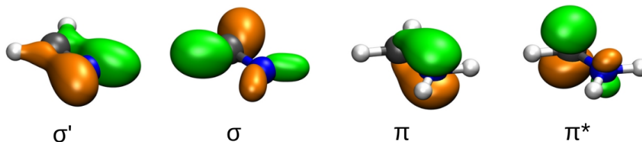
Figure 10. Excitation energies (in eV) of the two lowest singlet excited electronic states of protonated formalimine. Active space orbitals used in the multiconfigurational calculations are listed. Computational details follow those reported in Ref. 115.
