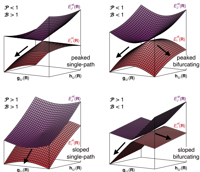
Figure 5. Schematic representation of the adiabatic PESs in the branching space of four two-state CXs characterised by different local topographies: (top left) peaked and single-path ( \delta_{gh} = 0.0949 , \Delta_{gh} = 0.5320 , s_x = 0.9550 , s_y = 0.0000 ); (top right) peaked and bifurcating ( \delta_{gh} = 0.1249 , \Delta_{gh} = 0.3402 , s_x = 0.0000 , s_y = 0.7133 ); (bottom left) sloped and single-path ( \delta_{gh} = 0.1326 , \Delta_{gh} = 0.2680 , s_x = 0.0000 , s_y = 2.1588 ); and (bottom right) sloped and bifurcating ( \delta_{gh} = 0.1399 , \Delta_{gh} = 0.8753 , s_x = 0.0000 , s_y = 0.4553 ). The numerical CX branching space topography parameters used to generate the plots in this figure were taken from Ref. [69]. We note that, here, in Fig. 5, and in Fig. 4, we use the (raw) \mathbf{g}_j(\mathbf{R}) and \mathbf{h}_j(\mathbf{R}) vector notation instead of the x and y (orthonormalized) scalar quantities for schematic simplicity.
