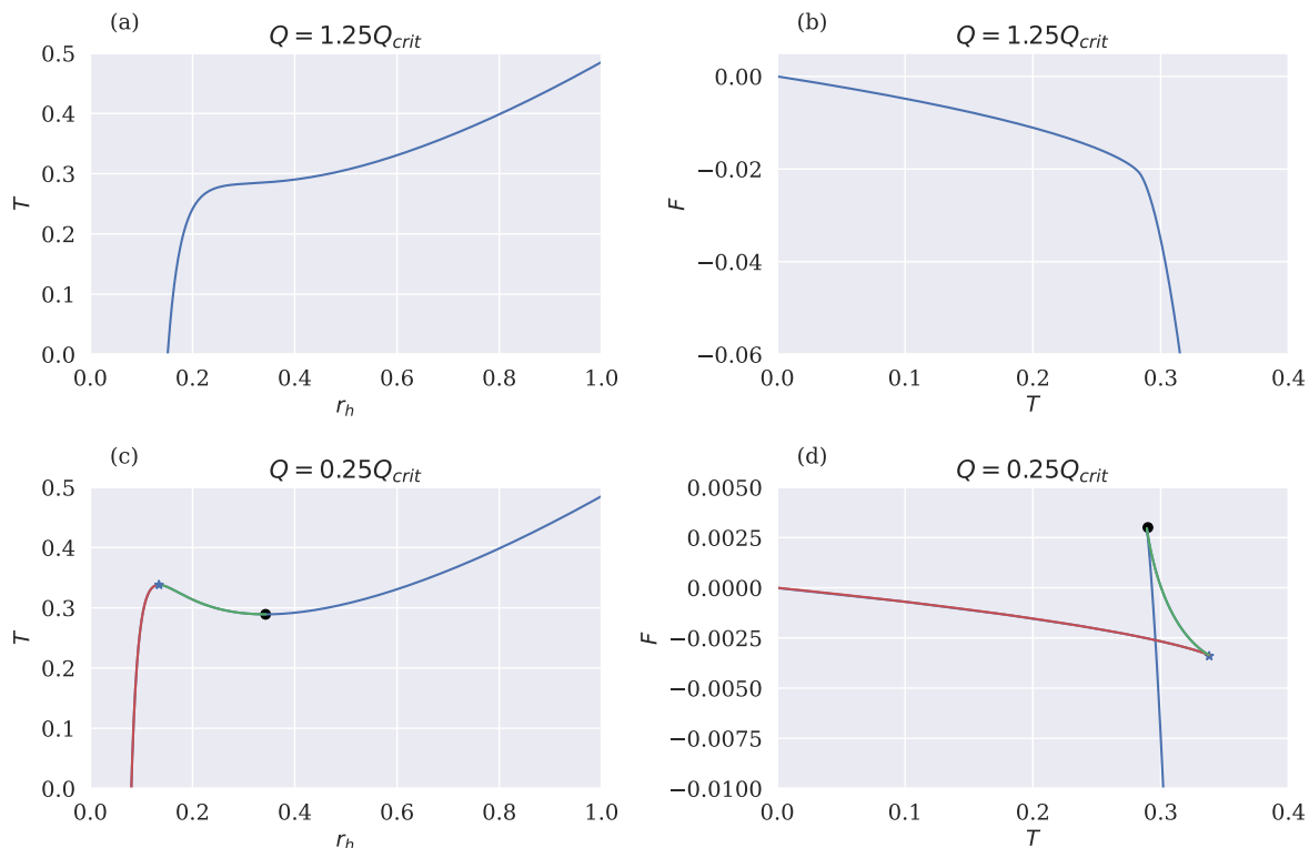
Figure 1. Hawking temperature vs. horizon radius, and free energy vs. Hawking temperature are depicted for two distinct charge regimes: Q = 1.25Q_{crit} > Q_{crit} (top row) and Q = 0.25Q_{crit} < Q_{crit} (bottom row). The figures are generated with fixed spacetime parameters, including (\theta = 0, k = r_F = Z_0 = \Phi_0 = 1, d = 3, \Omega_{kd} = 16\pi G, z = 3/2) . The qualitative behavior of these figures remain same for all allowed values of \theta and z .
