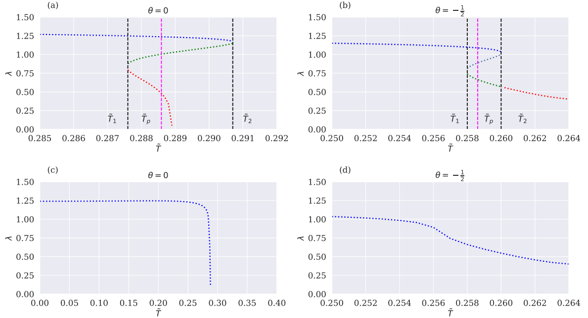
Figure 9. Lyapunov exponents for massless particles plotted against the Hawking temperature for two distinct charge regimes: Q = 0.8Q_{\text{crit}} < Q_{\text{crit}} (top row) and Q = 1.1Q_{\text{crit}} > Q_{\text{crit}} (bottom row). The left panel corresponds to the Lifshitz case with \theta = 0 , while the right panel represents the HSV case with \theta = -1/2 . The fixed spacetime parameters include ( k = r_F = Z_0 = \Phi_0 = 1 , d = 3 , \Omega_{kd} = 16\pi G , z = 3/2 ). The phase transition from Small Black Hole to Large Black Hole occurs at \tilde{T} = \tilde{T}_p .
