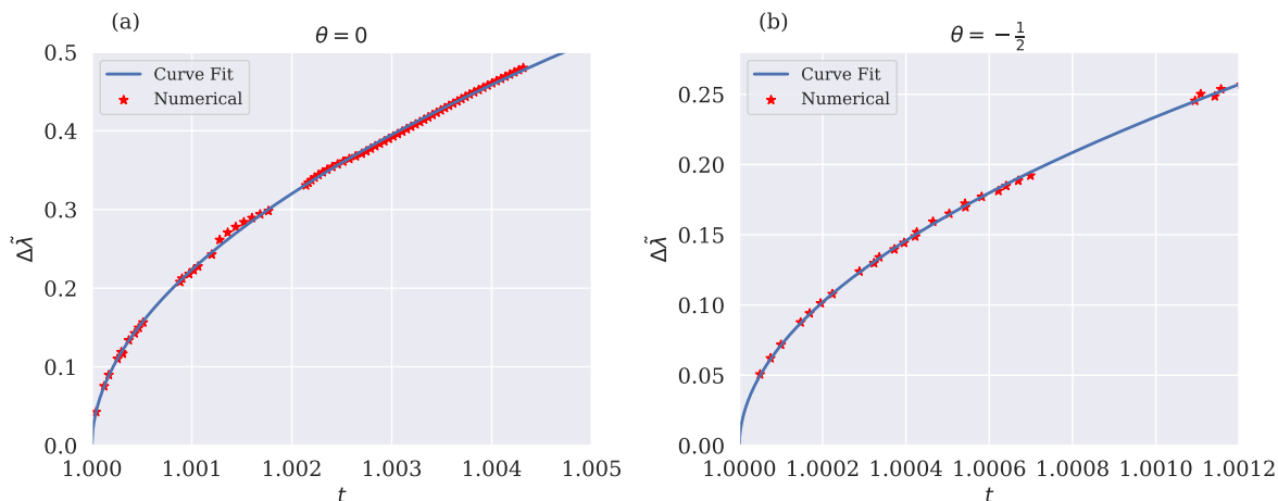
Figure 6. \Delta\tilde{\lambda} vs t plot for massive particles. Left: Lifshitz case, \theta = 0 . Right: HSV case, \theta = -1/2 . The red stars represent data points obtained from numerical calculations, and the blue solid line represents the fitted curve.
