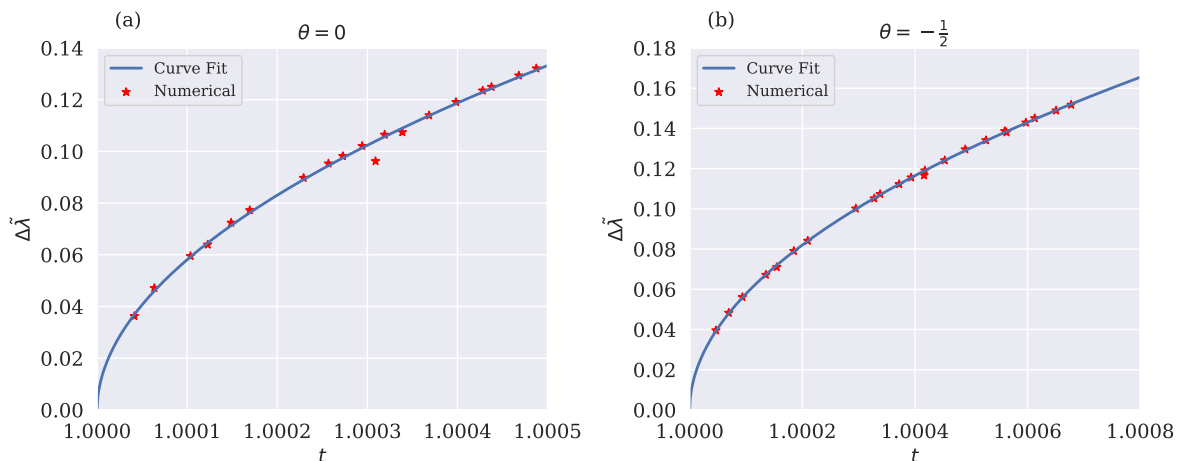
Figure 10. \Delta\tilde{\lambda} vs t plot for massless particles. Left: Lifshitz case, \theta = 0 . Right: HSV case, \theta = -1/2 . The red stars represent data points obtained from numerical calculations, and the blue solid line represents the fitted curve.
