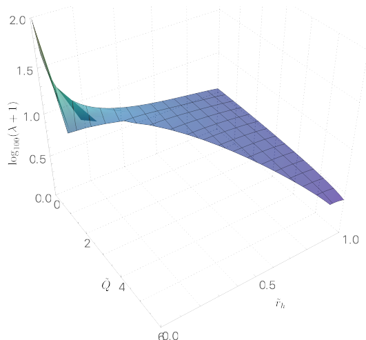
Figure 3. Three-dimensional plot illustrating \log_{100}(\lambda + 1) as a function of \tilde{Q} and \tilde{r}_h for massive particles in the Lifshitz case ( \theta = 0 ). The spacetime parameters are fixed with k = r_F = Z_0 = \Phi_0 = 1 , d = 3 , \Omega_{kd} = 16\pi G , and z = 3/2 . The exclusion of the no black hole region is enforced based on the positivity of the Hawking temperature, ensuring extremal black hole conditions.
