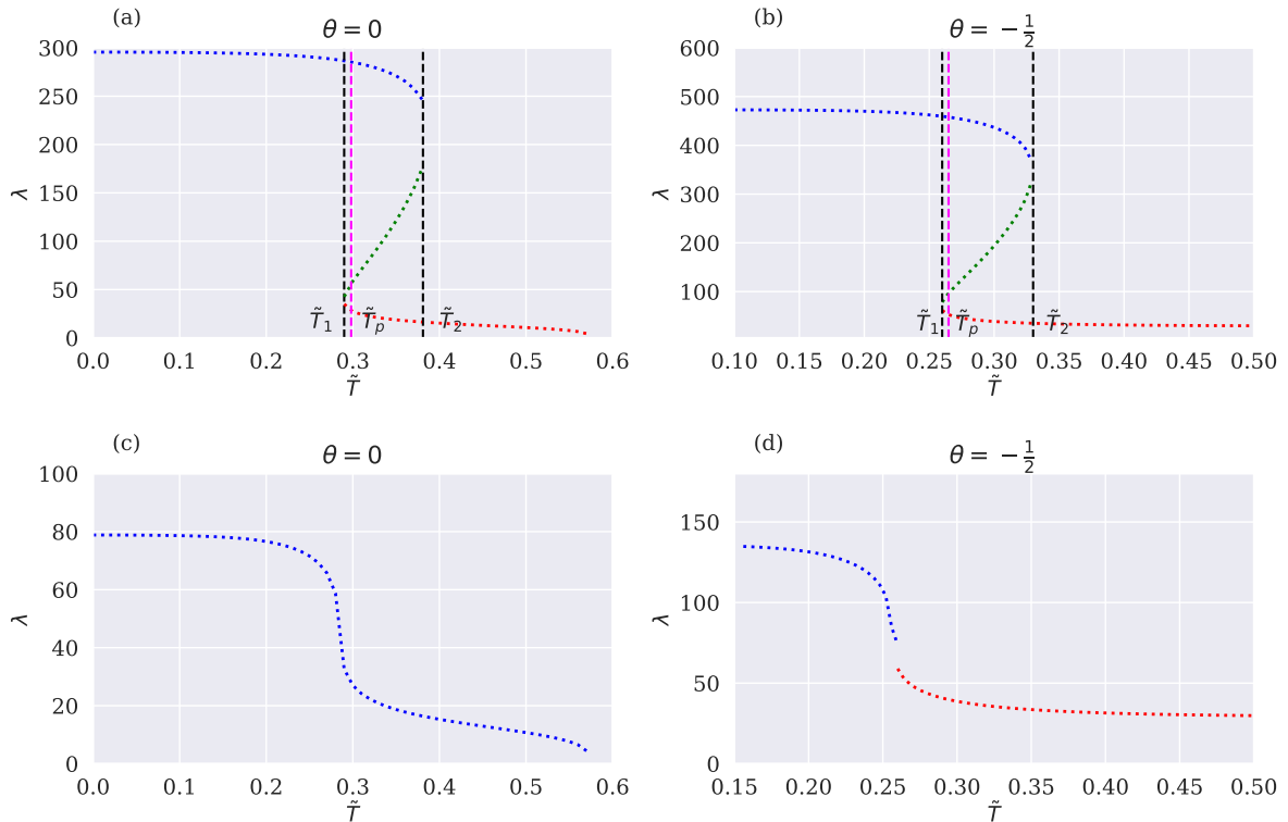
Figure 5. Lyapunov exponents for massive particles plotted against the Hawking temperature for two distinct charge regimes: Q = 0.1Q_{\text{crit}} < Q_{\text{crit}} (top row) and Q = 1.1Q_{\text{crit}} > Q_{\text{crit}} (bottom row). The left panel corresponds to the Lifshitz case with \theta = 0 , while the right panel represents the HSV case with \theta = -1/2 . The fixed spacetime parameters include (k = r_F = Z_0 = \Phi_0 = 1, d = 3, \Omega_{kd} = 16\pi G, z = 3/2) . The phase transition from Small Black Hole to Large Black Hole occurs at \tilde{T} = \tilde{T}_p . In all cases, \lambda initiates from a finite value at \tilde{T} = 0 and reaches zero after a certain temperature, though this is not displayed in every plot for the sake of a clear presentation. The plots are obtained numerically, and any discontinuity near the joining points is a result of numerical instability and limitations in the number of iterations to access those points. Otherwise, the connecting plots are continuous.
