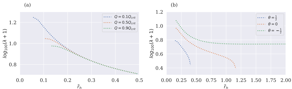
Figure 4. The cross-section \log_{100}(\lambda + 1) - \tilde{r}_h derived from the 3D plot with fixed Q values. Left: illustrating the impact of charge Q on \lambda while maintaining other spacetime parameters constant ( k = r_F = Z_0 = \Phi_0 = 1 , d = 3 , \Omega_{kd} = 16\pi G , z = 3/2 ) in the Lifshitz case ( \theta = 0 ). The selected Q variation is Q = (0.1Q_{\text{crit}}, 0.5Q_{\text{crit}}, 0.9Q_{\text{crit}}) . The qualitative behavior holds for all admissible z and \theta values. Right: demonstrating the influence of HSV parameter \theta on \lambda while keeping other spacetime parameters fixed ( k = r_F = Z_0 = \Phi_0 = 1 , d = 3 , \Omega_{kd} = 16\pi G , z = 3/2 , Q = 0.9Q_{\text{crit}} ). The chosen \theta variation is \theta = (-1/2, 0, 1/2) . The qualitative trends remain consistent across different \theta values.
