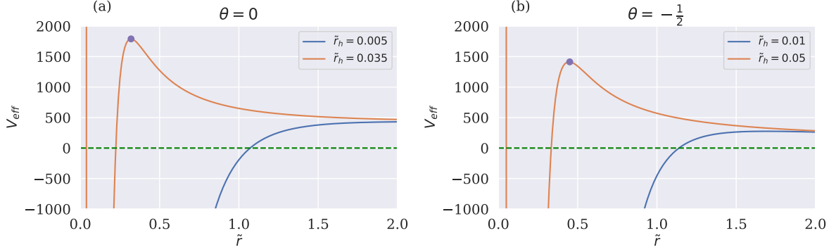
Figure 2. The effective potential V_{\text{eff}} governing the motion of massive particles in HSV spacetime is depicted. Left: Lifshitz case \theta = 0 . Right: HSV case \theta = -1/2 . In both instances, the spacetime parameters are set to k = r_F = Z_0 = \Phi_0 = 1 , with d = 3 , \Omega_{kd} = 16\pi G , z = 3/2 and \tilde{Q} = 0.01 . Without loss of generality, particle properties are chosen as E_n = 1 and L = 20l . The blue dot on the plot corresponds to an unstable circular orbit. Notably, the presence of an unstable circular orbit is dependent on the size of the black hole. For black holes with substantial sizes, there is no maximum in V_{\text{eff}} , indicating the absence of an unstable circular orbit.
