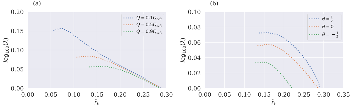
Figure 8. The cross-section of \log_{100}(\lambda) - \tilde{r}_h derived from the 3D plot with fixed Q values for massless particles. Left: illustrating the impact of charge Q on \lambda while maintaining other spacetime parameters constant ( k = r_F = Z_0 = \Phi_0 = 1 , d = 3 , \Omega_{kd} = 16\pi G , z = 3/2 ) in the Lifshitz case ( \theta = 0 ). The selected Q variation is Q = (0.1Q_{\text{crit}}, 0.5Q_{\text{crit}}, 0.9Q_{\text{crit}}) . The qualitative behavior holds for all admissible z and \theta values. Right: demonstrating the influence of the HSV parameter \theta on \lambda while keeping other spacetime parameters fixed ( k = r_F = Z_0 = \Phi_0 = 1 , d = 3 , \Omega_{kd} = 16\pi G , z = 3/2 , Q = 0.9Q_{\text{crit}} ). The chosen \theta variation is \theta = (-1/2, 0, 1/2) . The qualitative trends remain consistent across different \theta values. Notice that the trend is reversed in the right panel compared to the massive case (see figure 4).
