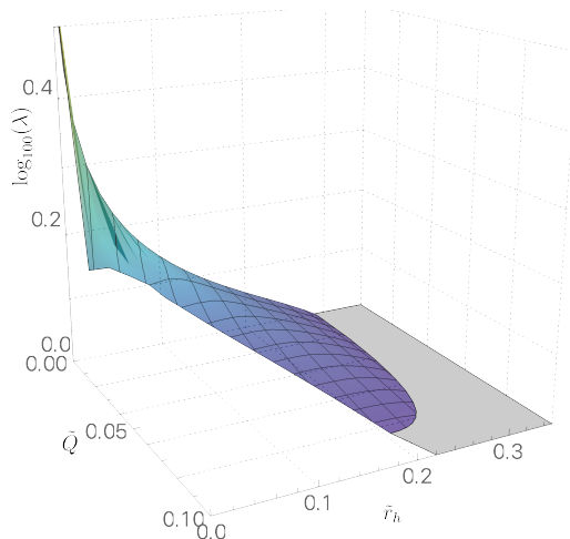
Figure 7. Three-dimensional plot depicting \log_{100}(\lambda) as a function of \tilde{Q} and \tilde{r}_h for massless particles in the Lifshitz case ( \theta = 0 ). The spacetime parameters are fixed with k = r_F = Z_0 = \Phi_0 = 1 , d = 3 , \Omega_{kd} = 16\pi G , and z = 3/2 . The exclusion of the no black hole region is enforced based on the positivity of the Hawking temperature, ensuring extremal black hole conditions. Notably, unlike AdS spacetime, the unstable null geodesics cease to exist beyond a certain r_h value. The Lyapunov exponent crosses zero in the \{\tilde{Q}, r_h\} plane in the \lambda = 0 line and continues further, taking negative values for larger r_h values. However, since we do not consider negative \lambda values in our study, we truncate that portion.
