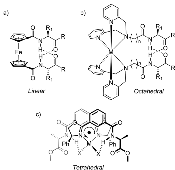
Fig. 11 Induction of chirality in: (a) dipeptidic ferrocene compounds, 21 (b) octahedral metal complexes of peptidic tridentate ligands 56 and (c) tetrahedral metal complexes of monodentate 2-aryloxazoline ligands presented herein.
