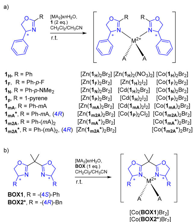
Scheme 1 Reaction conditions: [MA 2 ], M = Zn 2+ , Cd 2+ or Co 2+ , A = Br - , I - or NO 3 - ; CH 2 Cl 2 , r.t. The chirality at position 4 of the oxazoline ring is ( S ) in all cases except for ligands denoted with an asterisk (*), which contain ( 4R ) chirality, additionally marked by "( 4R )" in the scheme. All amino acid moieties are L-alanine methyl ester moieties meta substituted on the 2-phenyl group ( mA ).
