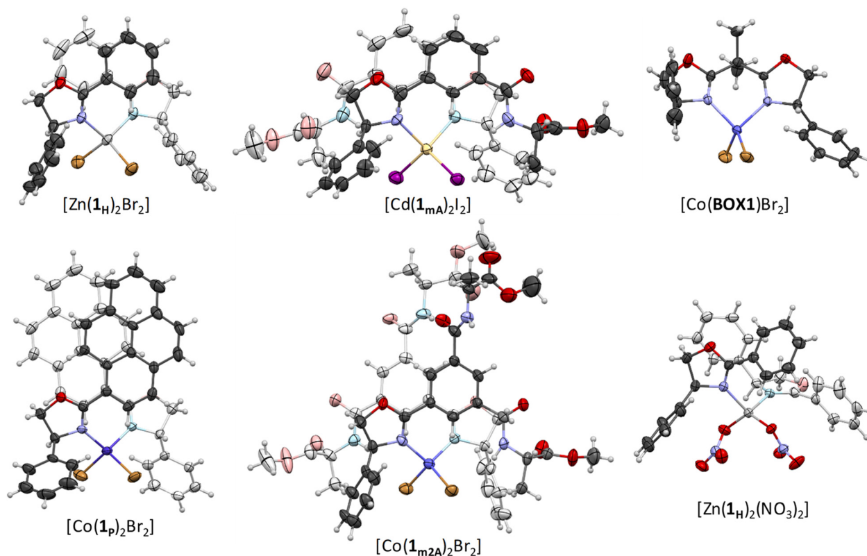
Fig. 4 ORTEP-III drawings 53 of complexes [\text{Zn}(\mathbf{1}_H)_2\text{Br}_2] , [\text{Cd}(\mathbf{1}_{mA})_2\text{I}_2] , [\text{Co}(\mathbf{BOX1})\text{Br}_2] , [\text{Co}(\mathbf{1}_P)_2\text{Br}_2] , [\text{Co}(\mathbf{1}_{m2A})_2\text{Br}_2] and [\text{Zn}(\mathbf{1}_H)_2(\text{NO}_3)_2] with 30% ellipsoid probability level for SCXRD-determined structures.
