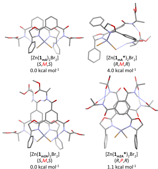
Fig. 9 Calculated structures of the most stable conformers of zinc bromide complexes with ligands 1_{m_A} , 1_{m_A^*} , 1_{m_{2A}} and 1_{m_{2A}^*} . Relative Gibbs energies ( \Delta G ) denoted below structures are calculated for diastereomeric pairs 1_{m_A} and 1_{m_A^*} , as well as 1_{m_{2A}} and 1_{m_{2A}^*} , respectively. All hydrogen atoms, except for those interacting via hydrogen bonding, were removed for clarity. Hydrogen bonds are highlighted by blue, dashed lines.
