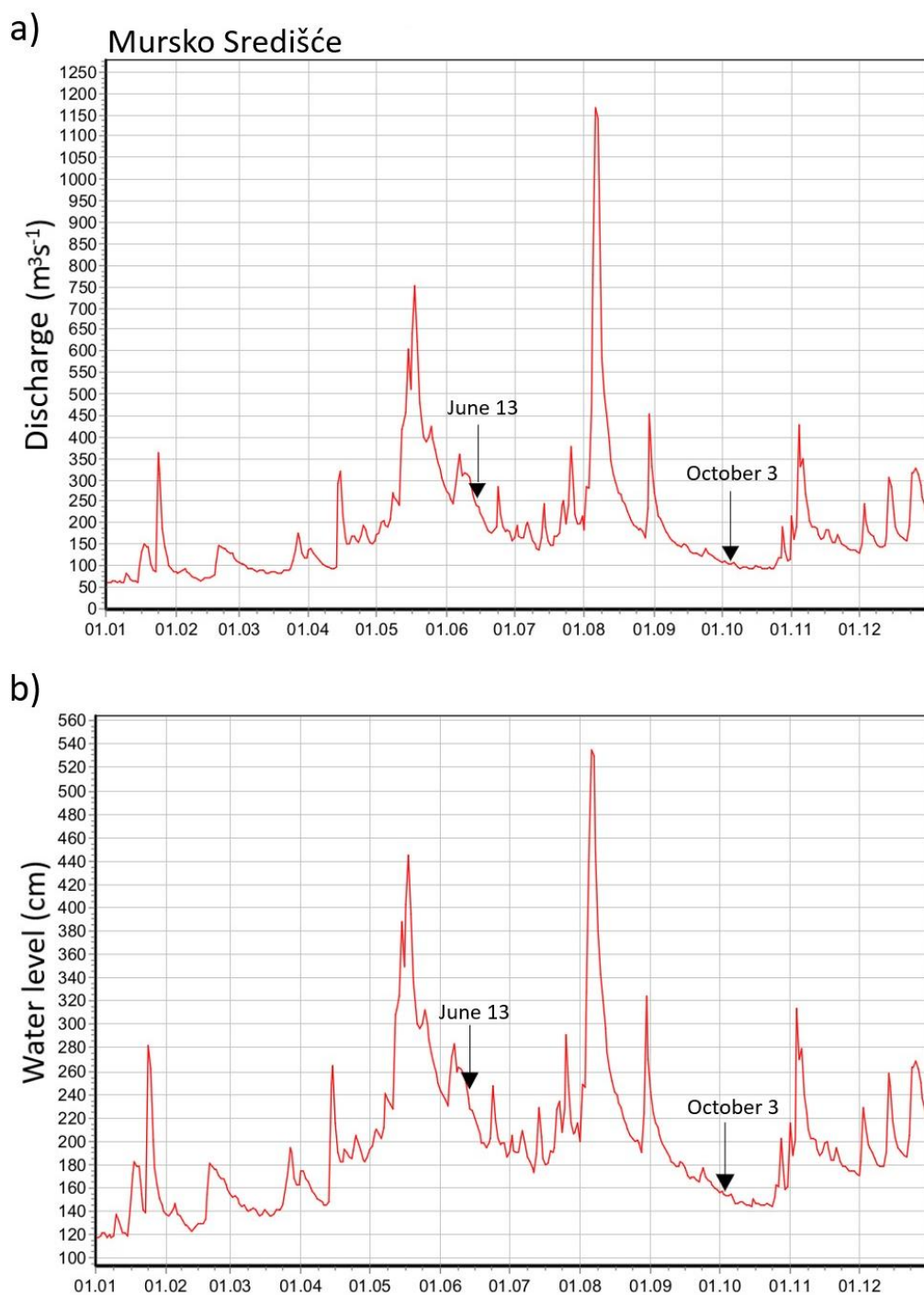
Figure ESM.4. Daily hydrological data for the Mursko Središće site at the Mura River: a) discharges; and b) water levels. The data refer to year 2023, and are provided by the Croatian Meteorological and Hydrological Service. The arrows in the graph indicate the initial times of water sampling in each sampling campaign, whereas the numbers on the x-axes represent the dates within the year 2023.
