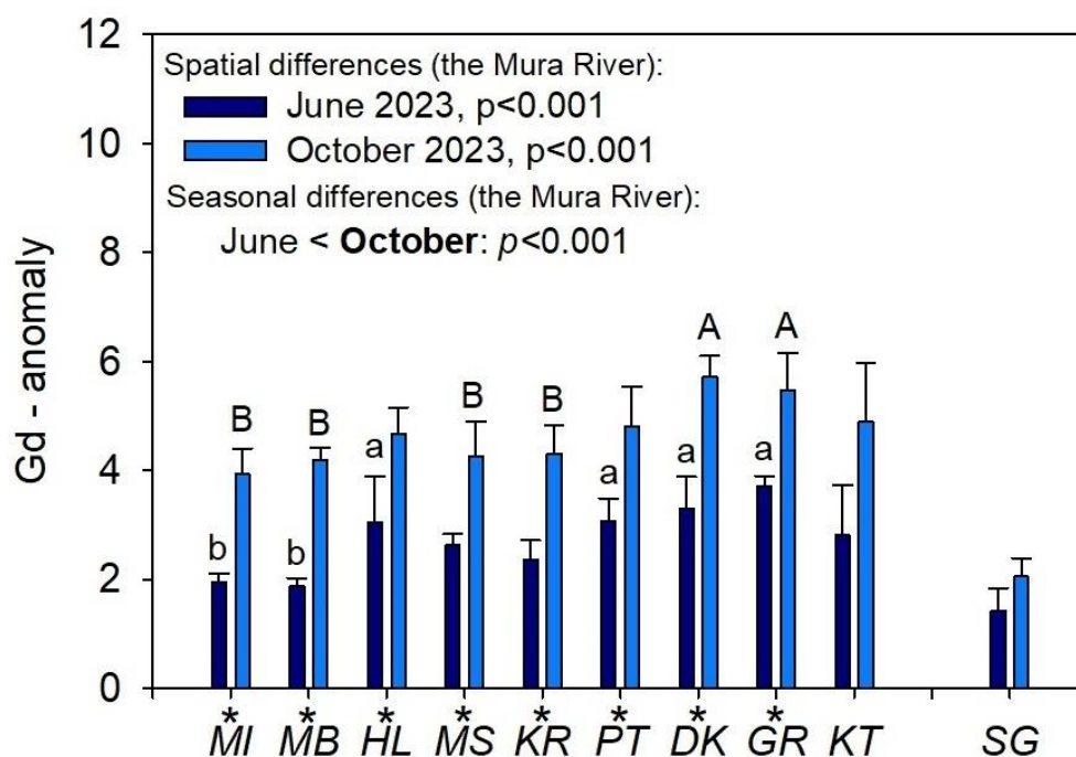
Figure 6. The Gd-anomalies calculated for June and October 2023 at nine sampling sites along the section of the Mura River flowing through Croatia (MI – the initial, most upstream location in Croatia; MB – location near bridge, in the municipality of Sveti Martin na Muri; HL – Hlapičina; MS – Mursko Središće; KR – Križovec; PT – Podturen; DK – Dekanovec; GR – Goričan; KT – Kotoriba), and at the stream Gradišćak (SG). The results and statistical comparisons were presented as in the Fig. 3.
