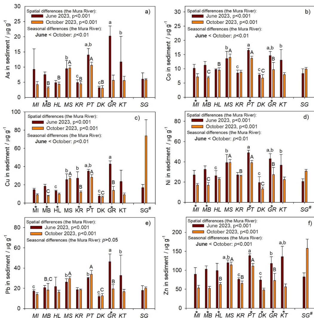
Figure 8. The concentrations of metals in sediments, As (a), Co (b), Cu (c), Ni (d), Pb (e), and Zn (f), measured in June and October 2023 at nine sampling sites along the section of the Mura River flowing through Croatia (MI – the initial, most upstream location in Croatia; MB – location near bridge, in the municipality of Sveti Martin na Muri; HL – Hlapičina; MS – Mursko Središće; KR – Križovec; PT – Podturen; DK – Dekanovec; GR – Goričan; KT – Kotoriba), and in the stream Gradišćak (SG). The results and statistical comparisons were presented as in the Fig. 3.
