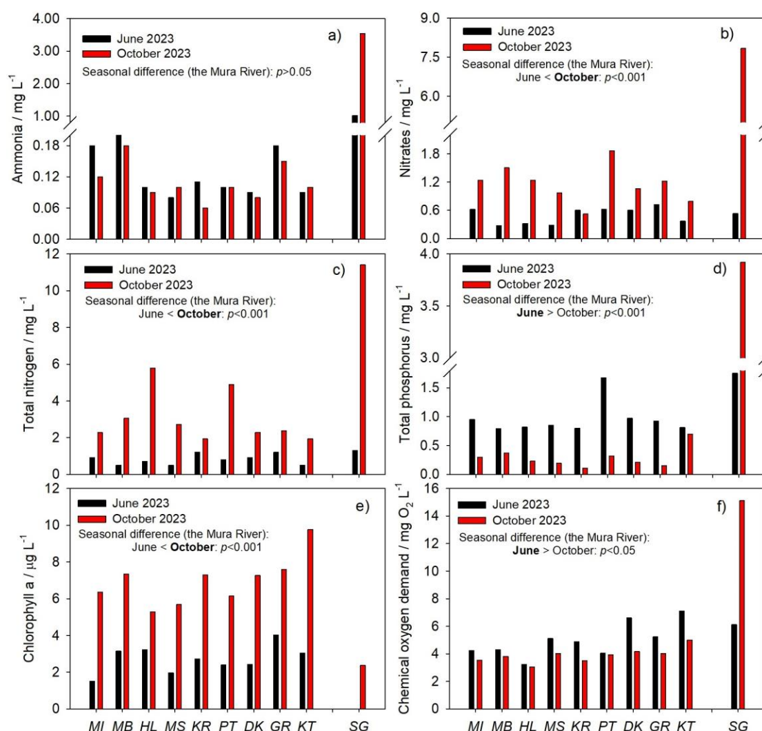
Figure 2. The values of nutrients (ammonia (a), nitrates (b), total nitrogen (c) and total phosphorus (d)), chlorophyll a (e), and chemical oxygen demand (f), measured in June and October 2023 at nine sampling sites along the section of the Mura River flowing through Croatia (MI – the initial, most upstream location in Croatia; MB – location near bridge, in the municipality of Sveti Martin na Muri; HL – Hlapičina; MS – Mursko Središće; KR – Križovec; PT – Podturen; DK – Dekanovec; GR – Goričan; KT – Kotoriba), and in the stream Gradišćak (SG). The results were presented as vertical bars ( n=1 ). Statistical comparison was made between two samplings (for all nine Mura-sites together), with the p -values stated within the figure.
