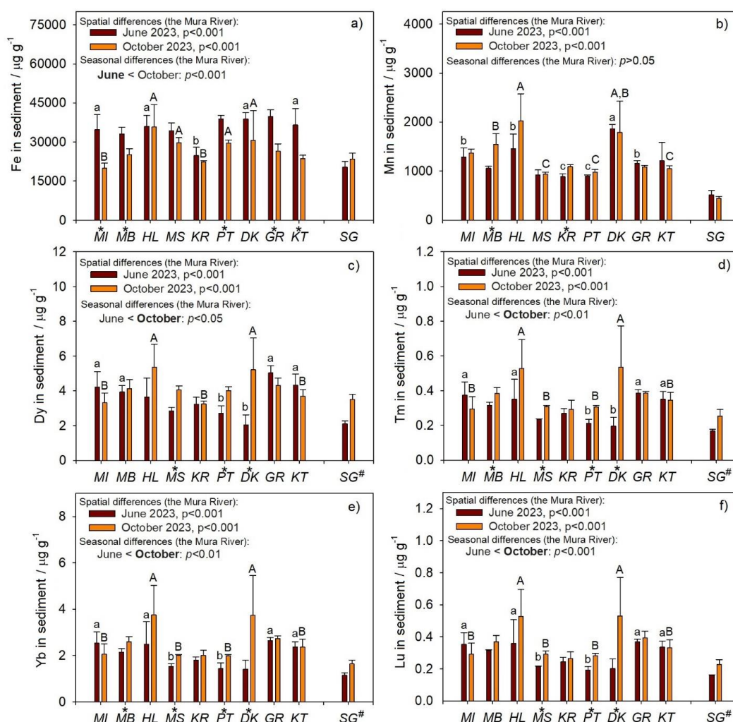
Figure 9. The concentrations of metals in sediments, Fe (a), Mn (b), Dy (c), Tm (d), Yb (e), and Lu (f), measured in June and October 2023 at nine sampling sites along the section of the Mura River flowing through Croatia (MI – the initial, most upstream location in Croatia; MB – location near bridge, in the municipality of Sveti Martin na Muri; HL – Hlapičina; MS – Mursko Središće; KR – Križovec; PT – Podturen; DK – Dekanovec; GR – Goričan; KT – Kotoriba), and in the stream Gradišćak (SG). The results and statistical comparisons were presented as in the Fig. 3.
