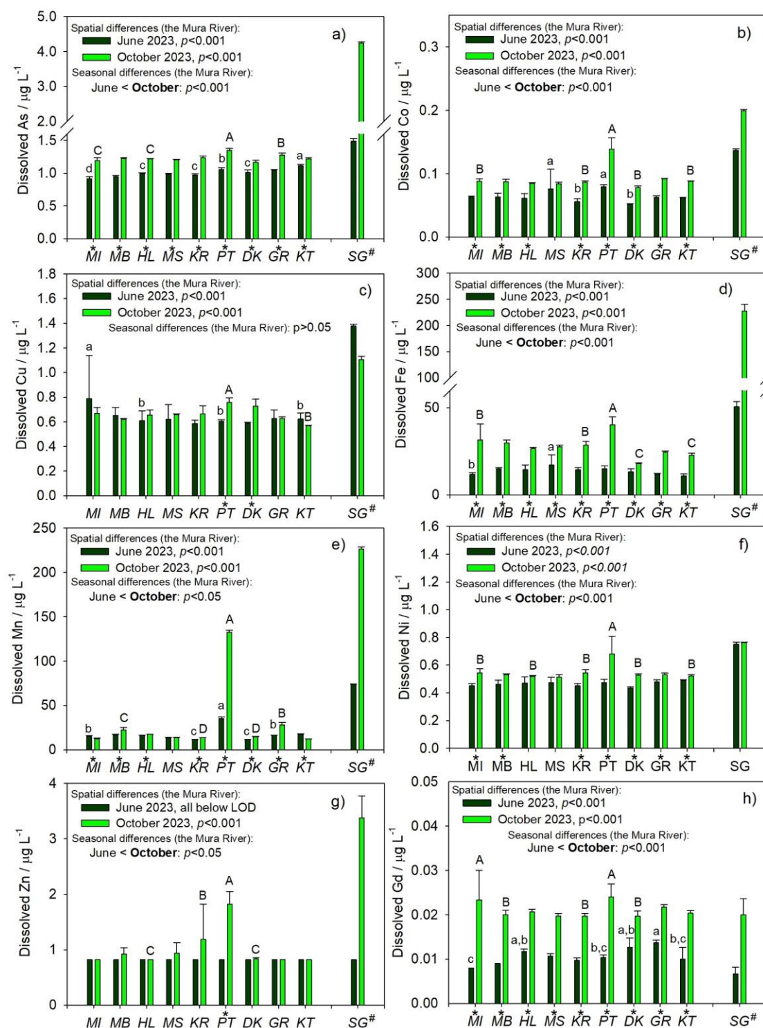
Figure 4. The concentrations of dissolved metals/metalloids (As (a), Co (b), Cu (c), Fe (d), Mn (e), Ni (f), Zn (g), and Gd (h)) measured in June and October 2023 at nine sampling sites along the section of the Mura River flowing through Croatia (MI – the initial, most upstream location in Croatia; MB – location near bridge, in the municipality of Sveti Martin na Muri; HL – Hlapičina; MS – Mursko Središće; KR – Križovec; PT – Podturen; DK – Dekanovec; GR – Goričan; KT – Kotoriba), and in the stream Gradišćak (SG). The results and statistical comparisons were presented as in the Fig. 3.
