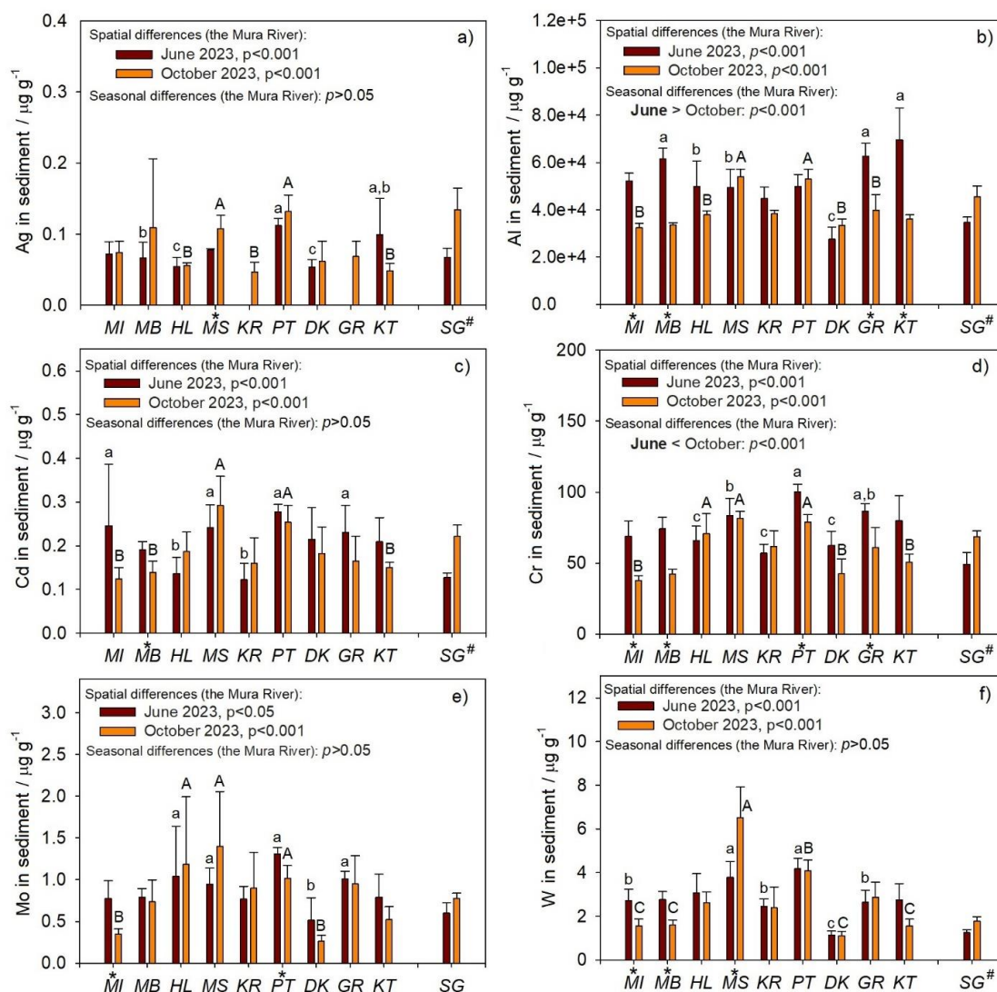
Figure 7. The concentrations of metals in sediments, Ag (a), Al (b), Cd (c), Cr (d), Mo (e), and W (f), measured in June and October 2023 at nine sampling sites along the section of the Mura River flowing through Croatia (MI – the initial, most upstream location in Croatia; MB – location near bridge, in the municipality of Sveti Martin na Muri; HL – Hlapičina; MS – Mursko Središće; KR – Križovec; PT – Podturen; DK – Dekanovec; GR – Goričan; KT – Kotoriba), and in the stream Gradišćak (SG). The results and statistical comparisons were presented as in the Fig. 3.
