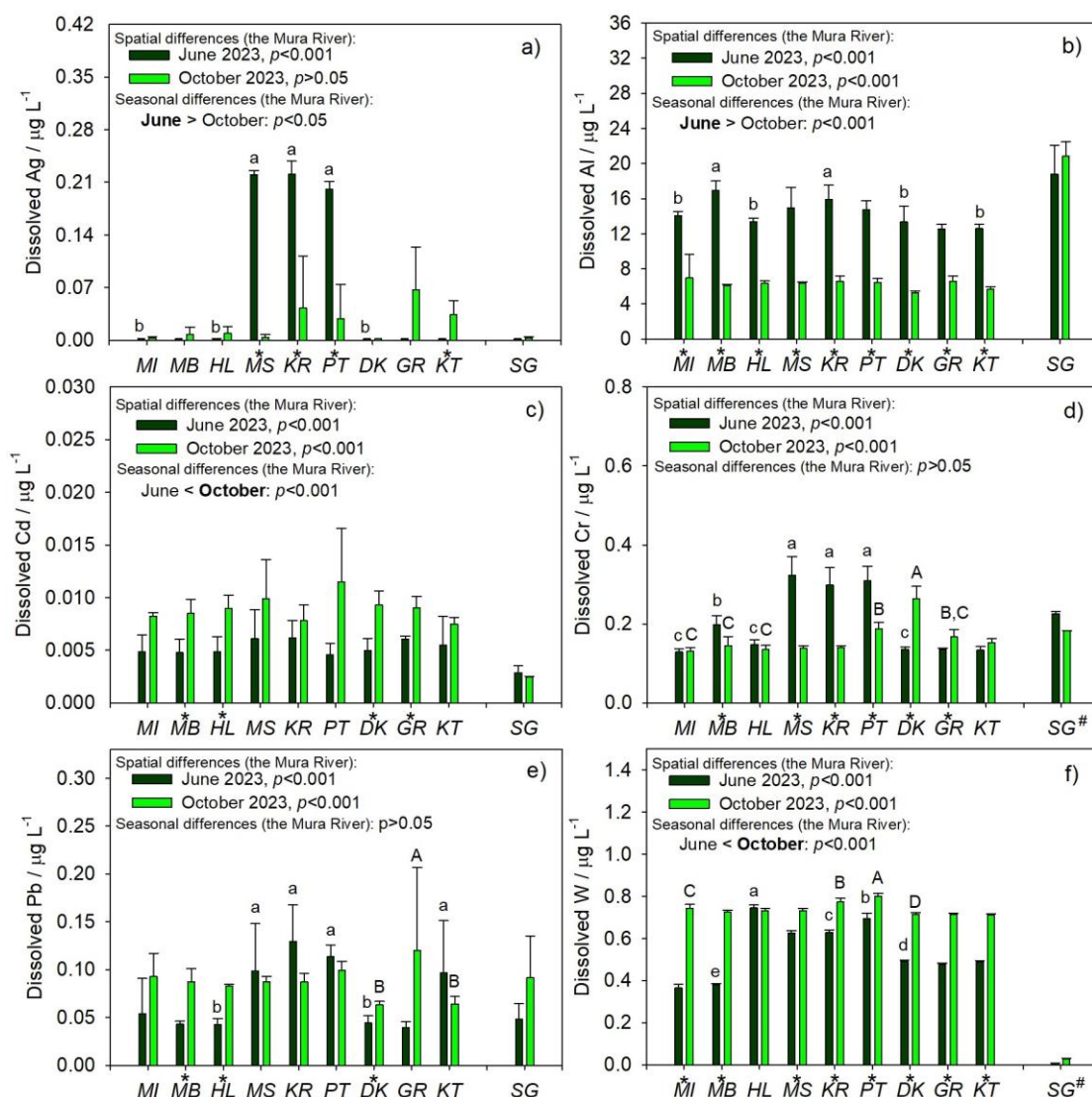
Figure 3. The concentrations of dissolved metals (Ag (a), Al (b), Cd (c), Cr (d), Pb (e), and W (f)) measured in June and October 2023 at nine sampling sites along the section of the Mura River flowing through Croatia (MI – the initial location in Croatia; MB –Sveti Martin na Muri; HL – Hlapičina; MS – Mursko Središće; KR – Križovec; PT – Podturen; DK – Dekanovec; GR – Goričan; KT – Kotoriba), and in the stream Gradišćak (SG). The results were presented as vertical bars (mean) with assigned standard deviations ( n=3 ). Statistical comparisons were made among nine Mura-sampling sites for each sampling, and between two samplings (for all Mura-sites together), with the p -values stated within the figure (SG was excluded from these comparisons). The selected post-hoc comparisons between sites were performed (taking in consideration the number of degrees of freedom); statistically significant differences ( p < 0.05 ) between sites were designated with different letters (lower case for June sampling, and upper case for October sampling). Statistically significant differences ( p < 0.05 ) between two seasons at each site were designated with asterisks (*).
