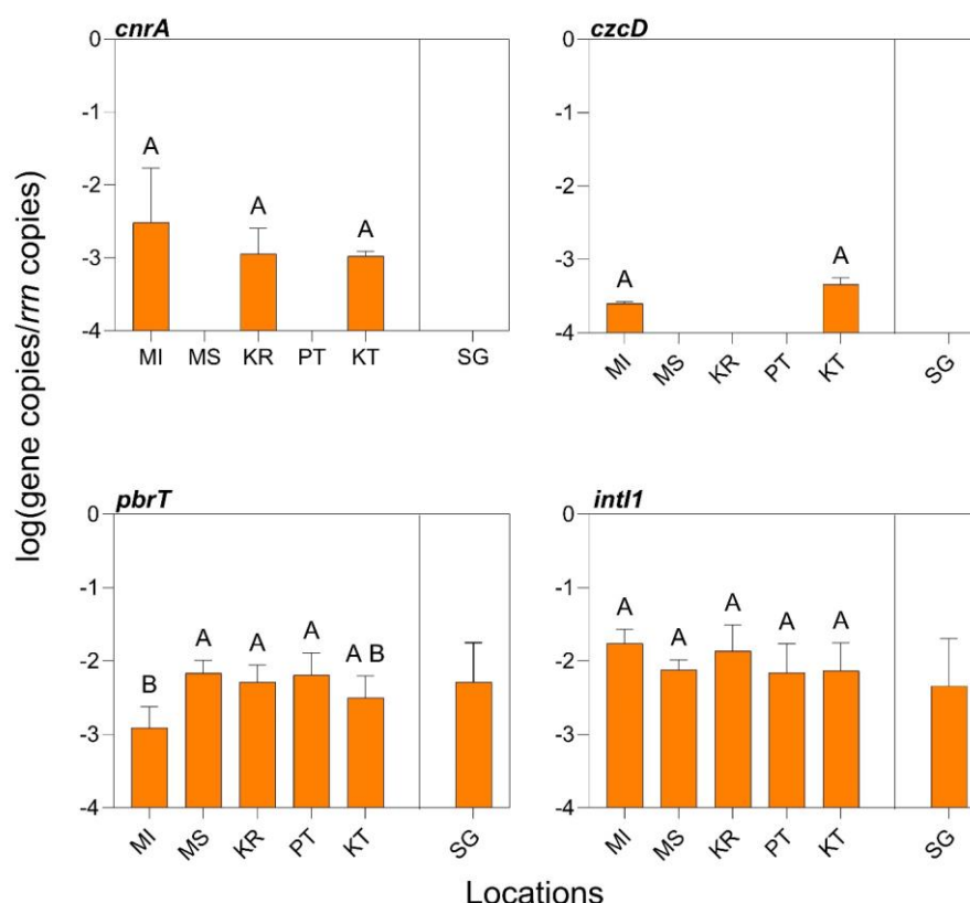
Figure 10. Relative abundance of metal resistance genes ( cnrA , czcD , and pbrT ) and class 1 integron-integrase ( intl1 ) in sediments from five Mura River locations (MI – the initial, most upstream location in Croatia; MS – Mursko Središće; KR – Križovec; PT – Podturen; KT – Kotoriba) and stream Gradišćak (SG). Each value represents the mean \pm standard deviation of three replicates. Different letters indicate significant differences between locations ( p < 0.05 ; comparison was made among five Mura River locations).
