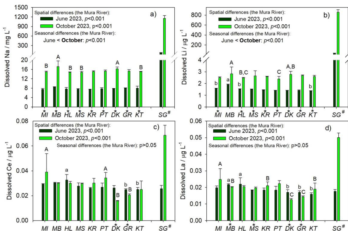
Figure 5. The concentrations of dissolved metals (Na (a), Li (b), Ce (c), and La (d)) measured in June and October 2023 at nine sampling sites along the section of the Mura River flowing through Croatia (MI – the initial, most upstream location in Croatia; MB – location near bridge, in the municipality of Sveti Martin na Muri; HL – Hlapičina; MS – Mursko Središće; KR – Križovec; PT – Podturen; DK – Dekanovec; GR – Goričan; KT – Kotoriba), and in the stream Gradišćak (SG). The results and statistical comparisons were presented as in the Fig. 3.
