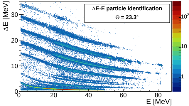
Fig. 1. Typical example of the particle identification spectrum obtained with the silicon strip detector telescopes for one pixel at the polar angle of 23.3^\circ .
