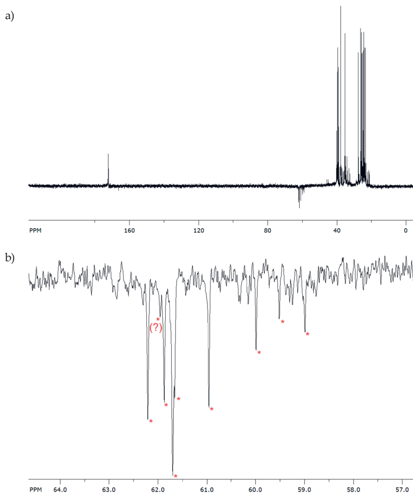
Fig. 3. a) APT- 13 C NMR spectra of the quenched and washed reaction; b) eight different signals in the negative region from 57–64 ppm correspond to eight different products.
