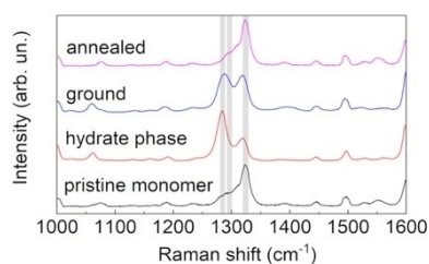
Figure 3. Normalized Raman spectra of pristine monomer, powder ground for 40 min in the mortar and powder ground and annealed at 60 ^{\circ}\text{C} for 2 h in air.
