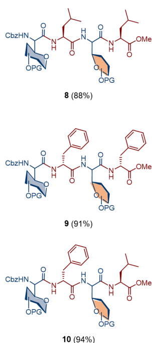
Scheme 4. Hetero-valent tetrapeptides
