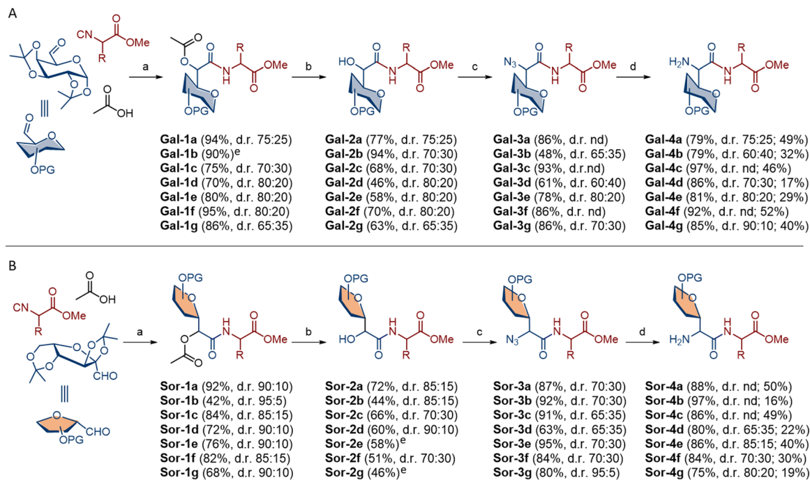
Scheme 2 Synthesis of homo- and heterochiral dipeptides containing C-glycosyl \alpha -amino acids derived from D-galactose (A) and L-sorbose (B). Reagent and conditions: (a) 0.1 mmol of all components in DCM, at RT, overnight; (b) NaOH (5 eq.) in MeOH (0.1 M), RT, 5 h; then K_2CO_3 (1.5 eq.) and MeI (3 eq.) in DMF (0.2 M) at 75 °C, overnight; (c) pyridine (10 eq.) and Tf_2O (3 eq.) in DCM (0.04 M) at -20 °C, 3 h; then NaN_3 (5 eq.) in DMF (0.2 M) at -20 °C, 24 h; (d) NaBH_4 (1.5 eq.) and NiCl_2 \cdot xH_2O (0.01 eq.) in DCM–EtOH (1:5, v/v, 0.02 M), at RT, 12 h; (e) main diastereoisomer was isolated by column chromatography; nd – not determined. Overall yields of Gal-4 and Sor-4 are also given (second number in parenthesis).
