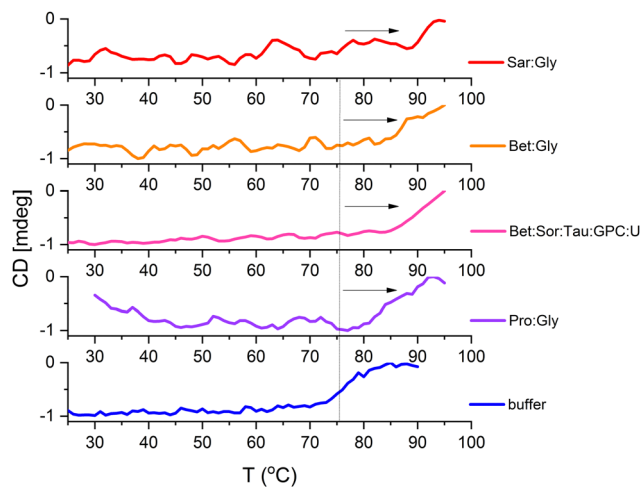
Fig. 3 Thermal CD scans of lysozyme in 50 mM potassium phosphate buffer (pH 6.4) and DESs containing 40% of water, w/w ( c_{\text{Lys}} = 0.3\text{--}0.4 \text{ mg ml}^{-1} ; \lambda = 227 \pm 5 \text{ nm} ): ellipticity change is a consequence of secondary structure change.
