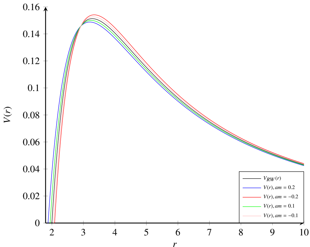
FIG. 2: Plot of the potential for R = 2 ( M = 1 ) and \ell = 2 , but only around the peak.
