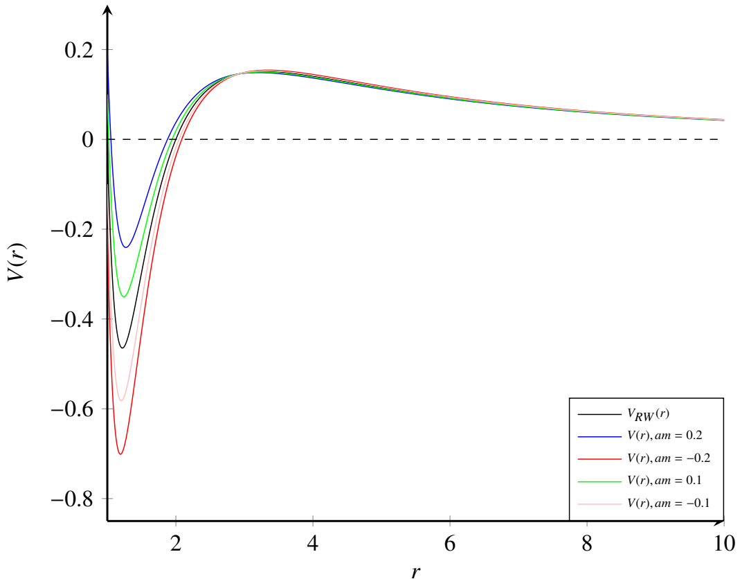
FIG. 1: The figure is drawn for R = 2 ( M = 1 ) and \ell = 2 for a wider range of r and V(r) . Around the peak and further away from the horizon, the behaviour appears to be very similar to the commutative case.
