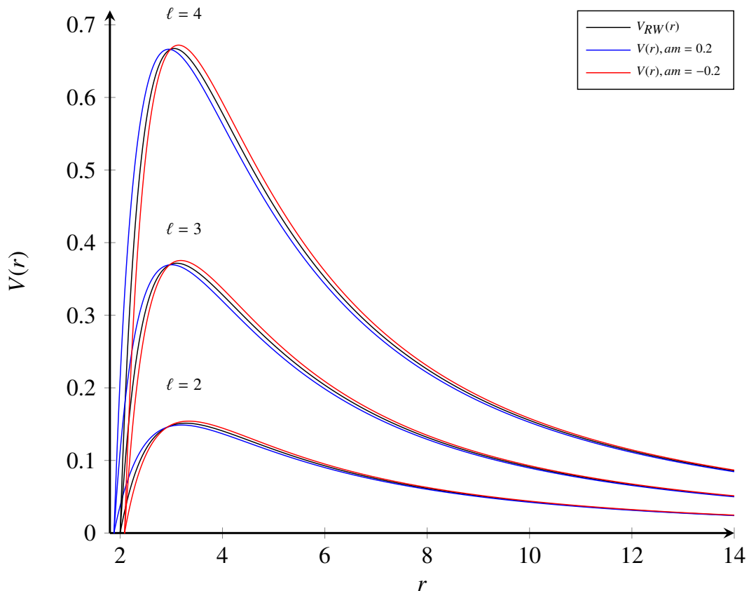
FIG. 3: Plot of the potential for R = 2 ( M = 1 ) and \ell = 2, 3, 4 .
