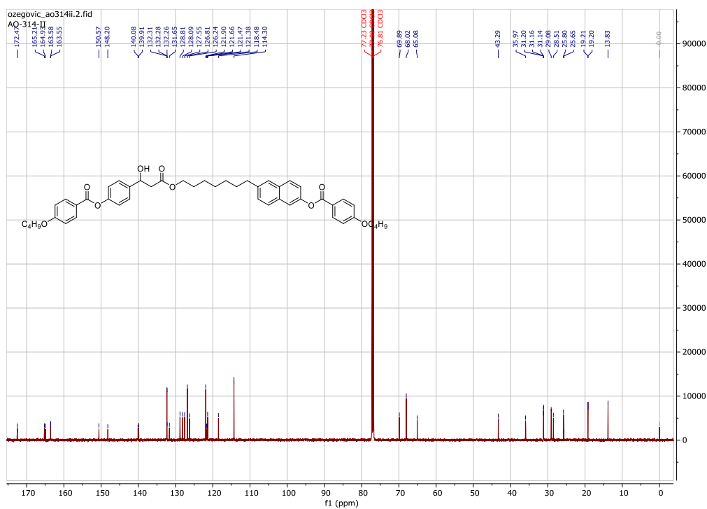
D1.14. ^{13}\text{C} NMR spektar spoja BB-7-NB, (S)-BB-7-NB
