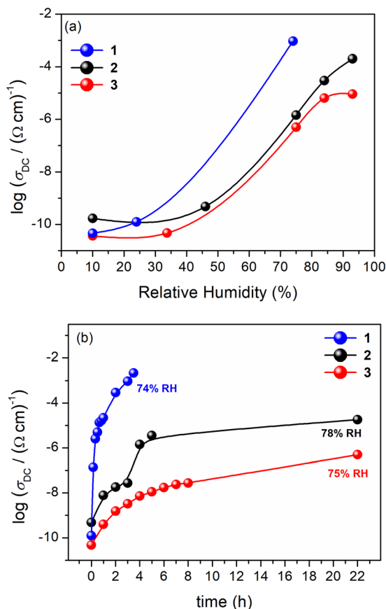
Fig. 7 (a) The proton conductivity as a function of relative humidity (RH) at room temperature for compounds 1–3; (b) time-dependent conductivity tests for compounds 1–3 at \approx 75\% RH.
