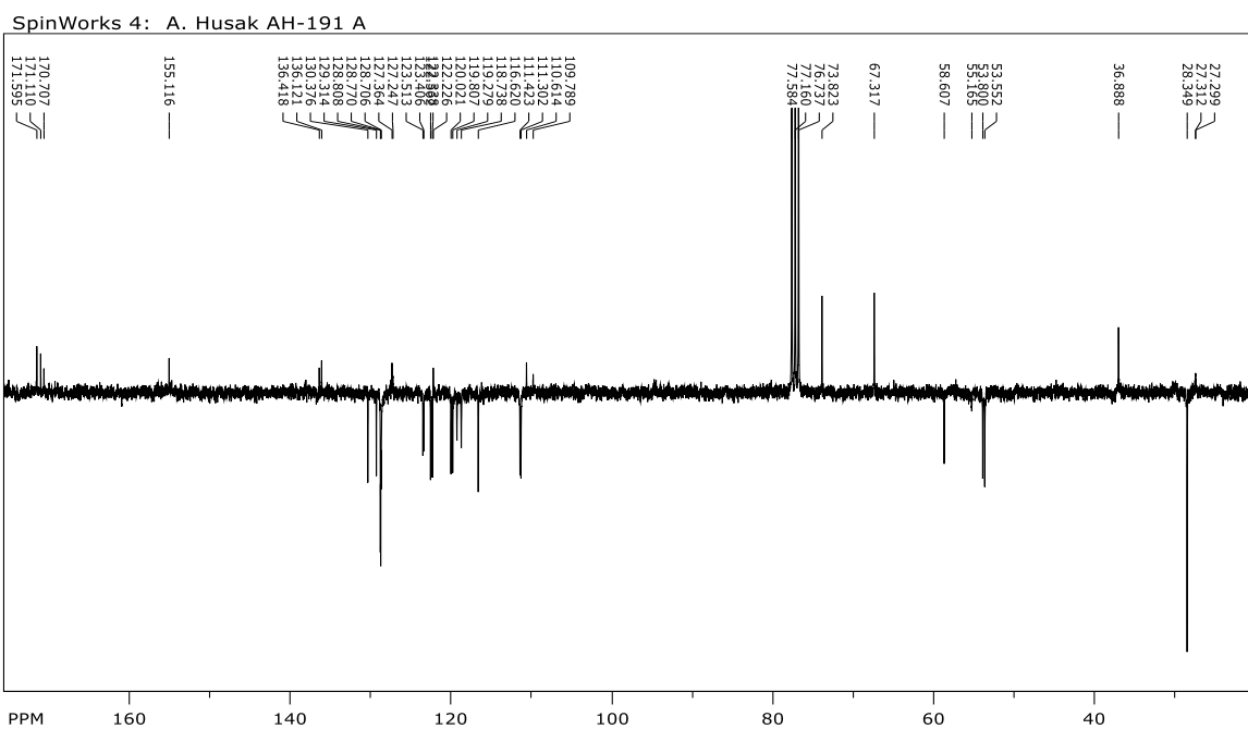
Prilog 59. ^{13}\text{C} NMR ( \text{CDCl}_3 , 75 MHz) spektr Boc-Trp-Trp-Tyr[ \text{CH}_2\text{OCH}_3 ]-OBn ( 37 )
