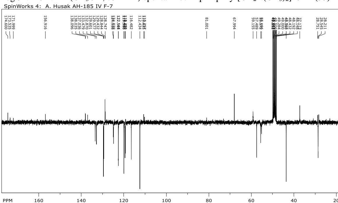
Prilog 51. ^{13}\text{C} NMR ( \text{CD}_3\text{OD} , 75 MHz) spektar Boc-Trp-Trp-Tyr[ \text{CH}_2\text{N}(\text{CH}_3)_2 ]-OBn ( 33 )
