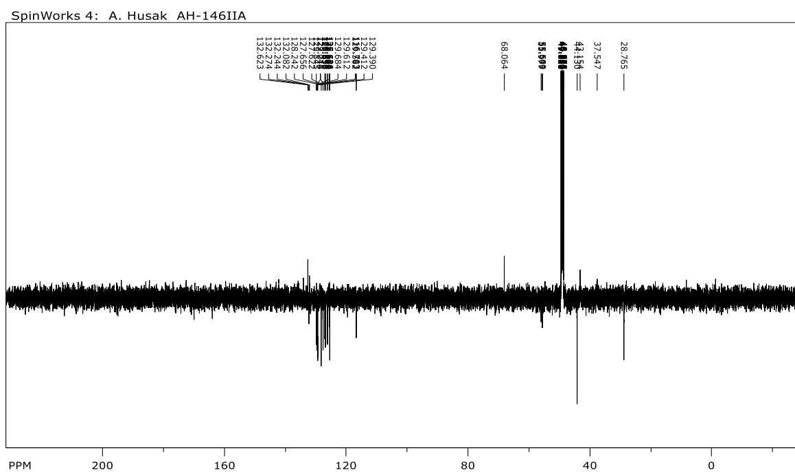
Prilog 68. ^{13}\text{C} NMR ( \text{CD}_3\text{OD} , 75 MHz, APT) spektr Boc-Pyr-Tyr[ \text{CH}_2\text{N}(\text{CH}_3)_2 ]-OBn ( 42 )
