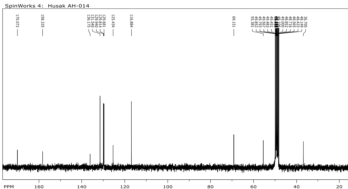
Prilog 18. 13 C NMR (CD 3 OD, 75 MHz) spektar TFA×H-Tyr-OBn ( 10 )
