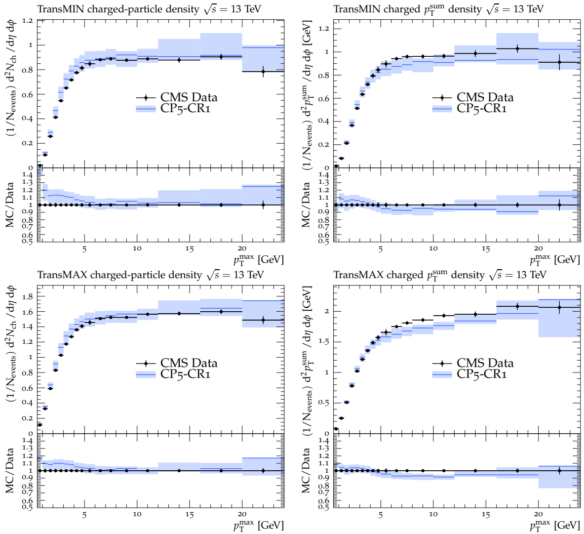
Figure B.3: The charged-particle (left) and p_T^{\text{sum}} densities (right) in the transMIN (upper) and transMAX (lower) regions as functions of the p_T of the leading charged particle, p_T^{\text{max}} , measured by the CMS experiment at \sqrt{s} = 13 TeV [17]. The predictions of the tunes CP5-CR1 are compared with data. The coloured band represents the tune uncertainties.
