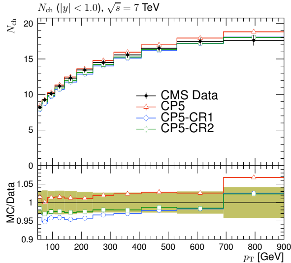
Figure 16: Average charged-hadron multiplicity, as a function of the jet p_T , for jets with rapidity |y| < 1 , measured by the CMS experiment at \sqrt{s} = 7 TeV [27]. The predictions of the CP5 and CP5-CR tunes are compared with data. The coloured band and error bars on the data points represent the total experimental uncertainty in the data.
