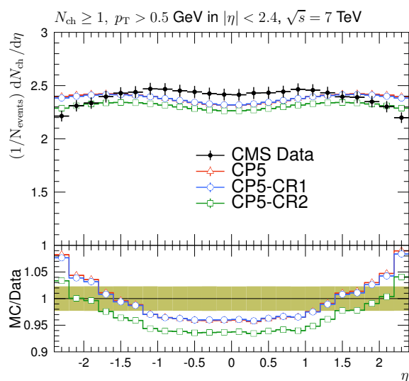
Figure 10: The pseudorapidity of charged particles, dN_{\text{ch}}/d\eta , with at least one charged particle in |\eta| < 2.4 , measured by the CMS experiment at \sqrt{s} = 7 \text{ TeV} [31]. The predictions of the CP5 and CP5-CR tunes are compared with data. The coloured band and error bars on the data points represent the total experimental uncertainty in the data.
