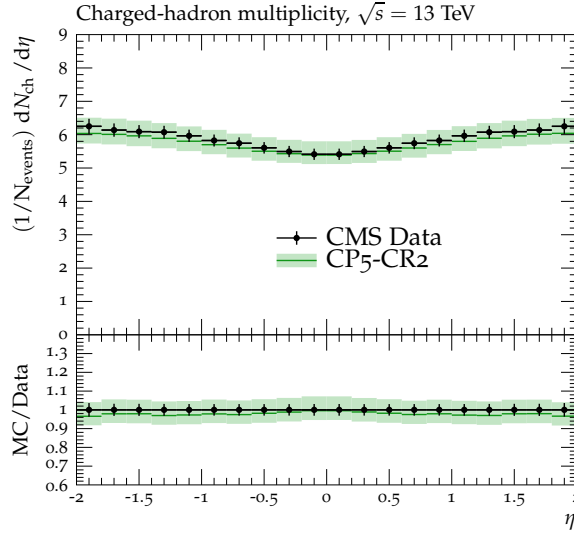
Figure B.4: The pseudorapidity of charged hadrons, dN_{\text{ch}}/d\eta , measured by the CMS experiment at \sqrt{s} = 13 TeV [22]. The prediction of the CP5-CR2 tune is compared with data. The coloured band represents the tune uncertainties.
