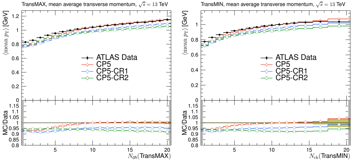
Figure 7: The mean charged-particle average transverse momentum as functions of charged-particle multiplicity in the transMAX (left) and transMIN (right) regions, measured by the ATLAS experiment at \sqrt{s} = 13 TeV [18]. The predictions of the CP5 and CP5-CR tunes are compared with data. The coloured band and error bars on the data points represent the total experimental uncertainty in the data.
