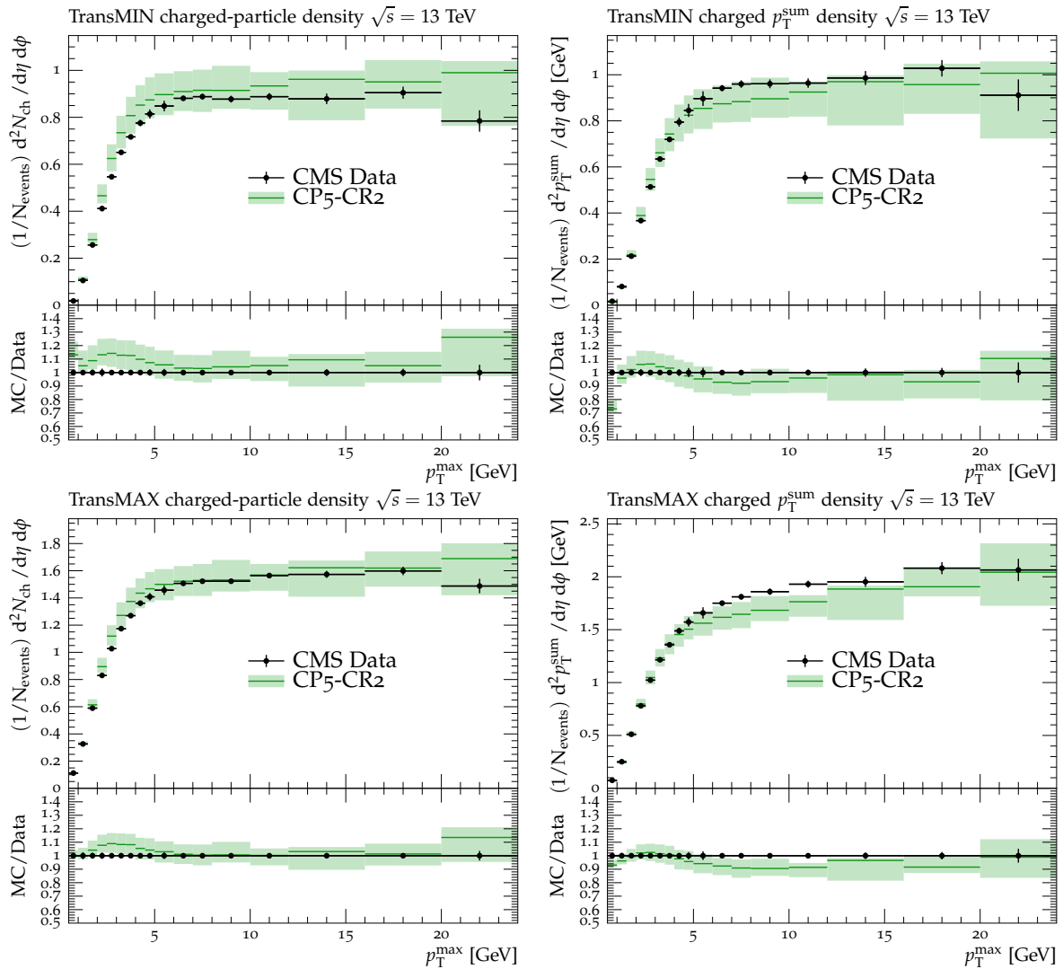
Figure B.5: The charged-particle (left) and p_T^{\text{sum}} densities (right) in the transMIN (upper) and transMAX (lower) regions as functions of the p_T of the leading charged particle, p_T^{\text{max}} , measured by the CMS experiment at \sqrt{s} = 13 TeV [17]. The predictions of the tunes CP5-CR2 are compared with data. The coloured band represents the tune uncertainties.
