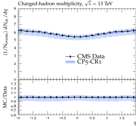
Figure B.2: The pseudorapidity of charged hadrons, dN_{\text{ch}}/d\eta , measured by the CMS experiment at \sqrt{s} = 13 TeV [22]. The prediction of the CP5-CR1 tune is compared with data. The coloured band represents the tune uncertainties.
