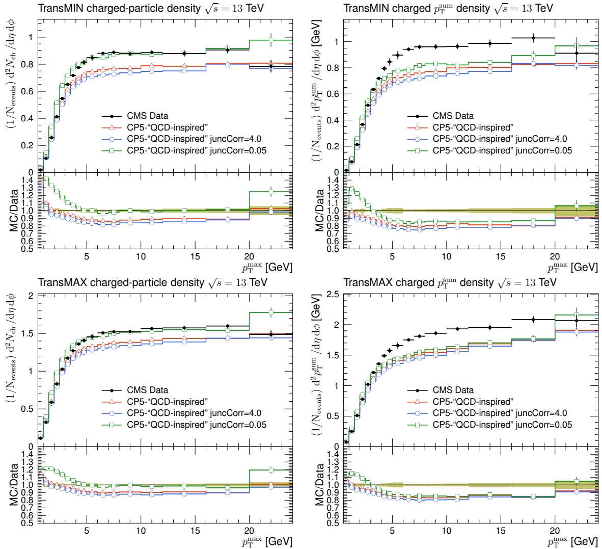
Figure C.2: The charged-particle (left) and p_T^{\text{sum}} densities (right) in the transMIN (upper) and transMAX (lower) regions as functions of the p_T of the leading charged particle, p_T^{\text{max}} , measured by the CMS experiment at \sqrt{s} = 13 TeV [17]. The red line shows the prediction of CP5-“QCD-inspired,” where the default value of the ColourReconnection:junctionCorrection parameter is 1.2. The predictions shown with the blue and green lines use 4.0 and 0.05 for the ColourReconnection:junctionCorrection parameter, respectively. These comparisons demonstrate the sensitivity of the ColourReconnection:junctionCorrection parameter to these observables.
