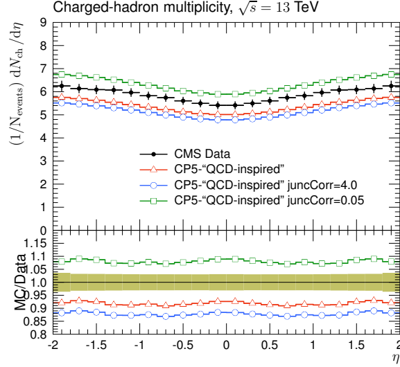
Figure C.1: The pseudorapidity of charged hadrons, dN_{\text{ch}}/d\eta , measured in |\eta| < 2 by the CMS experiment at \sqrt{s} = 13 TeV [23]. The red line shows the prediction of CP5-"QCD-inspired," where the default value of the ColourReconnection:junctionCorrection parameter is 1.2. The predictions shown with the blue and green lines use 4.0 and 0.05 for the ColourReconnection:junctionCorrection parameter, respectively. These comparisons demonstrate the sensitivity of the ColourReconnection:junctionCorrection parameter to this observable.
