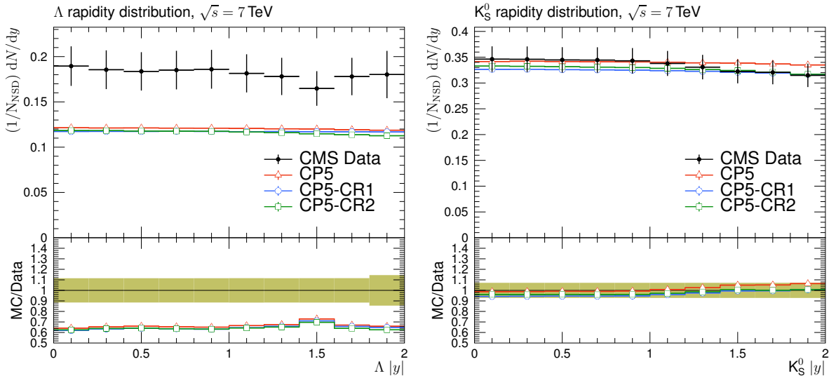
Figure 14: The strange particle production, \Lambda baryons (left) and K_S^0 mesons (right), as a function of rapidity, measured by the CMS experiment at \sqrt{s} = 7 TeV [16]. The predictions of the CP5 and CP5-CR tunes are compared with data. The coloured band and error bars on the data points represent the total experimental uncertainty in the data.
