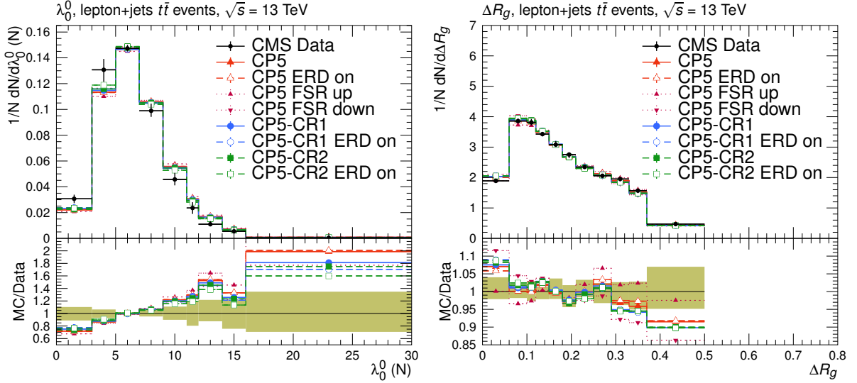
Figure 19: Distributions of the particle multiplicity in gluon jets (left) and the angle \Delta R_g between two groomed subjects in inclusive jets (right) measured by the CMS experiment in t\bar{t} events at \sqrt{s} = 13 TeV [53]. The coloured band and error bars on the data points represent the total experimental uncertainty in the data.
