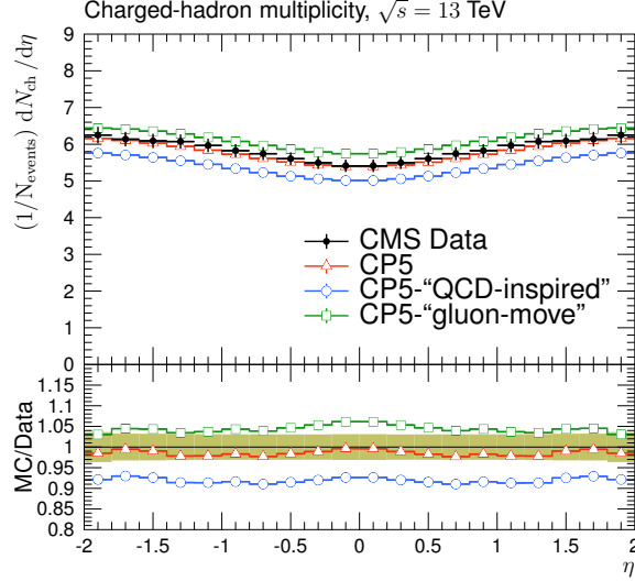
Figure 4: The pseudorapidity of charged hadrons, dN_{\text{ch}}/d\eta , measured in |\eta| < 2 by the CMS experiment at \sqrt{s} = 13 TeV [23]. The predictions of the tunes CP5, CP5-“QCD-inspired”, and CP5-“gluon-move” using their default parameter settings in Refs. [9, 14], are compared with data. The coloured band and error bars on the data points represent the total experimental uncertainty in the data where model uncertainty is also included. The comparisons show that the models need to be retuned in order to have a better agreement with the data.
