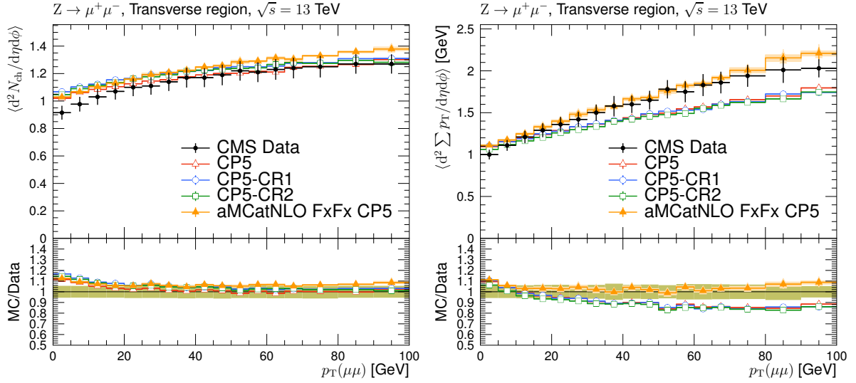
Figure 18: Number of charged particles and p_T flow in the transverse region of DY events, measured by the CMS experiment at \sqrt{s} = 13 TeV in bins of Z boson p_T [44]. The plots show the predictions of PYTHIA 8 with the CP5 and CP5-CR tunes, as well as MADGRAPH5_aMC@NLO with the CP5 tune compared with data. The coloured band and error bars on the data points represent the total experimental uncertainty in the data.
