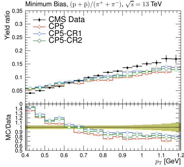
Figure 15: Ratios of particle yields, p/\pi , as a function of transverse momentum in minimum-bias events, measured by the CMS experiment at \sqrt{s} = 13 TeV [39]. The predictions of the CP5 and CP5-CR tunes are compared with CMS data. The coloured band and error bars on the data points represent the total experimental uncertainty in the data.
