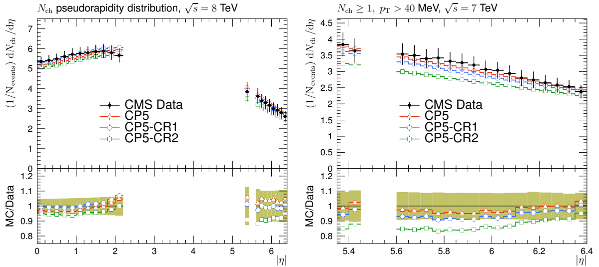
Figure 13: The pseudorapidity of charged particles, dN_{\text{ch}}/d\eta , measured by the CMS and TOTEM collaborations at \sqrt{s} = 8 TeV [32] (left) and measured by the TOTEM collaboration at \sqrt{s} = 7 TeV [33] (right). The predictions of the CP5 and CP5-CR tunes are compared with data. The coloured band and error bars on the data points represent the total experimental uncertainty in the data. For the CMS-TOTEM measurement, at least one charged particle with p_T > 0 is required in 5.3 < \eta < 6.5 or -6.5 < \eta < -5.3 . For the TOTEM measurement, at least one charged particle with p_T > 40 MeV is required in 5.3 < |\eta| < 6.4 .
