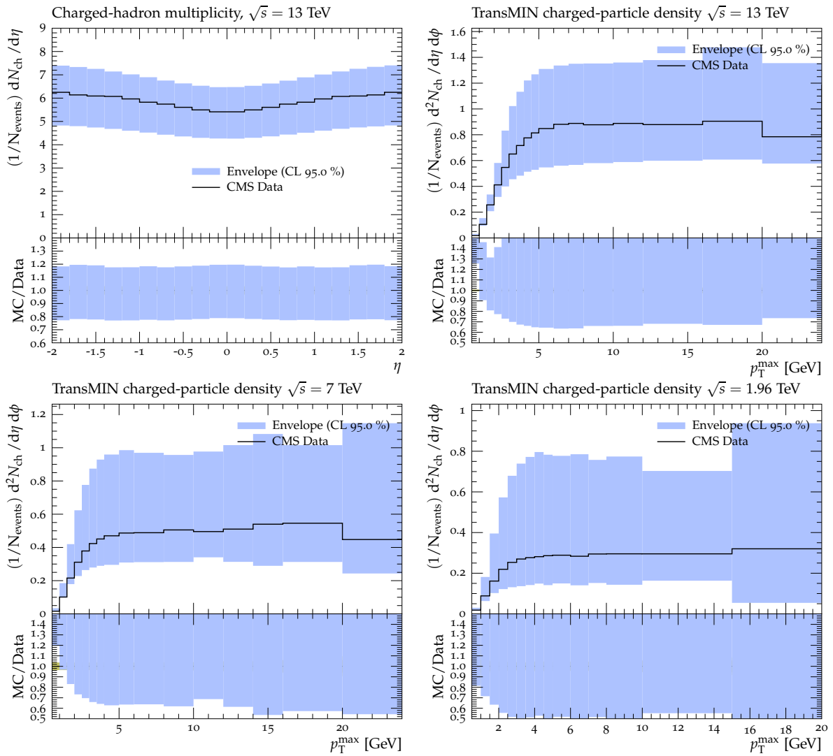
Figure B.1: Sample histograms showing the range of variation available on the observable histograms are given for CP5-CR1.
