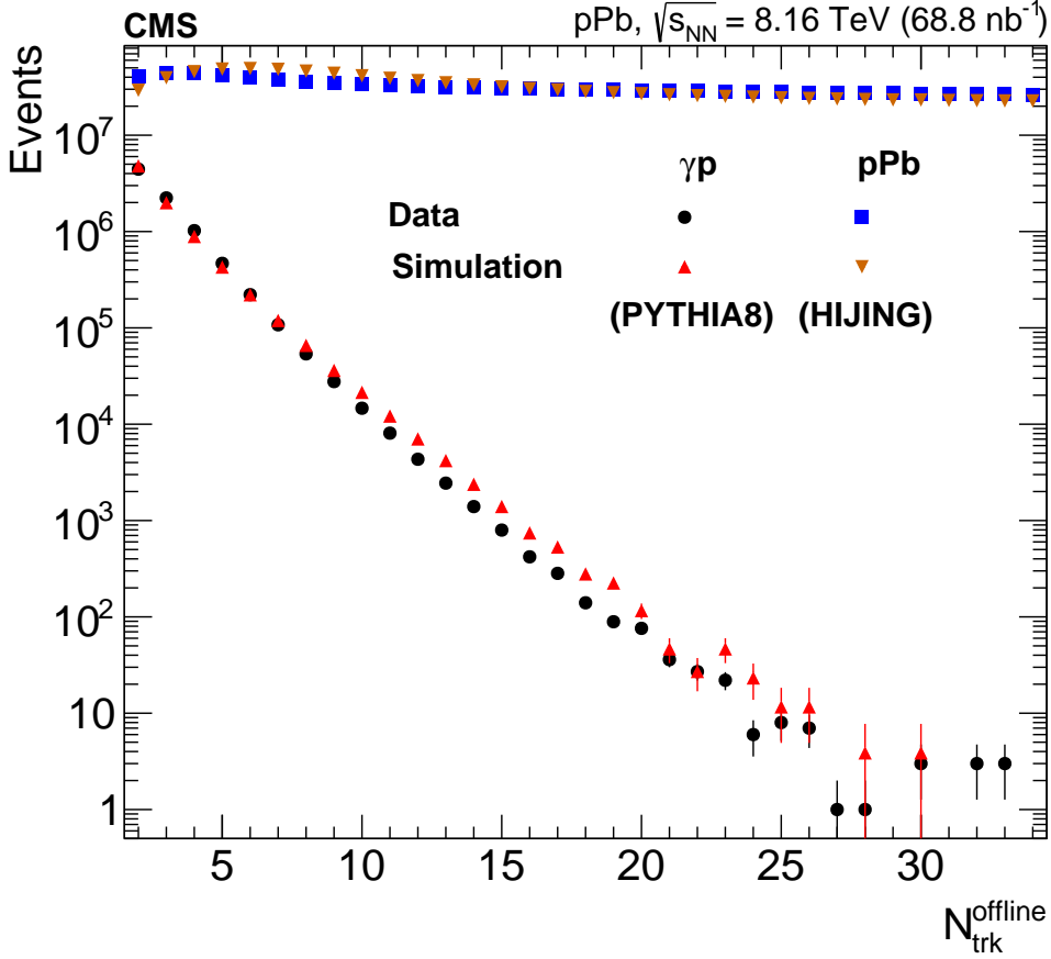
Figure 1: The N_{\text{trk}}^{\text{offline}} spectra for \gamma p and MB samples. The simulated \gamma p distribution has been normalized to the same event yield as the \gamma p -enhanced data sample.
