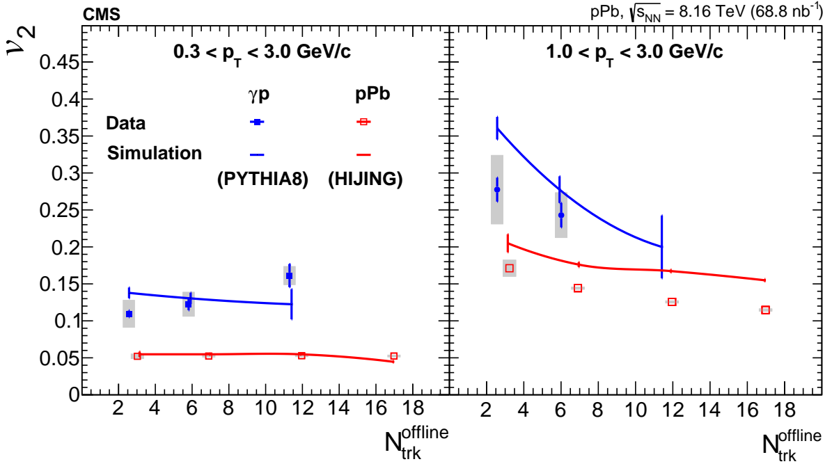
Figure 4: Single-particle azimuthal anisotropy v_2 versus N_{\text{trk}}^{\text{offline}} for \gamma p -enhanced and pPb samples in two p_T regions. Systematic uncertainties are shown by the shaded bars in the two panels. Predictions from the PYTHIA8 and HIJING generators are shown for the \gamma p and MB pPb samples respectively. For the \gamma p events, same N_{\text{trk}}^{\text{offline}} bin arrangement as in Figure 3 is kept while for pPb the bins [2, 5) , [5, 10) , [10, 15) and [15, 20) are used.
