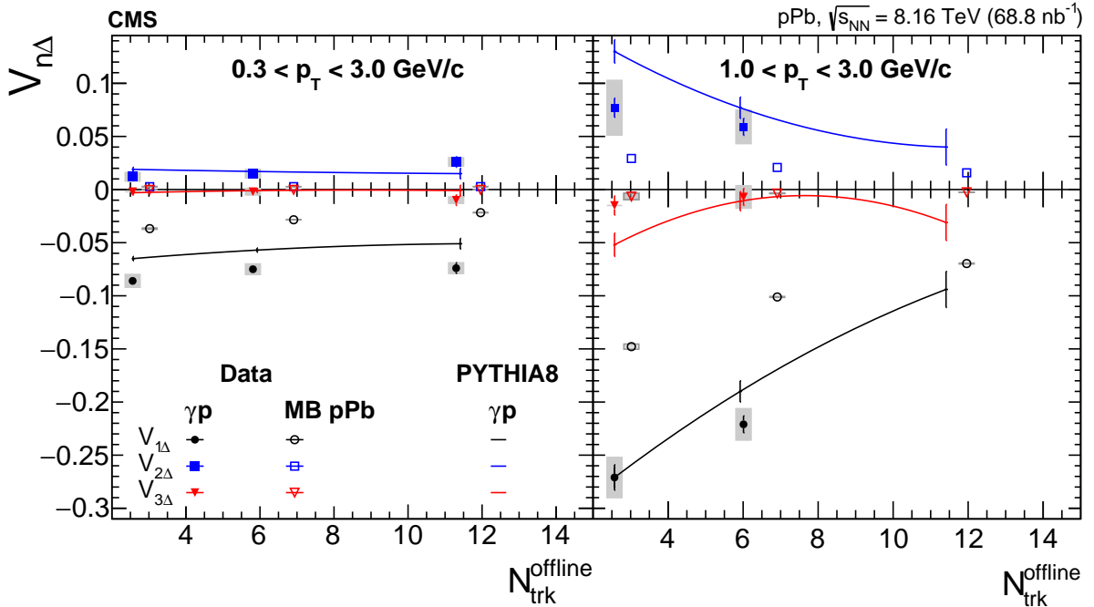
Figure 3: Dependence of V_{n\Delta} on N_{\text{trk}}^{\text{offline}} for \gamma p and MB events for two different p_T ranges. Systematic uncertainties are shown by the shaded bars in the two panels. The 2 \leq N_{\text{trk}}^{\text{offline}} < 5 , 5 \leq N_{\text{trk}}^{\text{offline}} < 10 , 10 \leq N_{\text{trk}}^{\text{offline}} < 35 are used for the lower p_T range and 2 \leq N_{\text{trk}}^{\text{offline}} < 5 and 5 \leq N_{\text{trk}}^{\text{offline}} < 35 for the higher range. The points are placed at the mean value of the corresponding N_{\text{trk}}^{\text{offline}} range. Lines indicate the prediction for \gamma p events from PYTHIA8.
