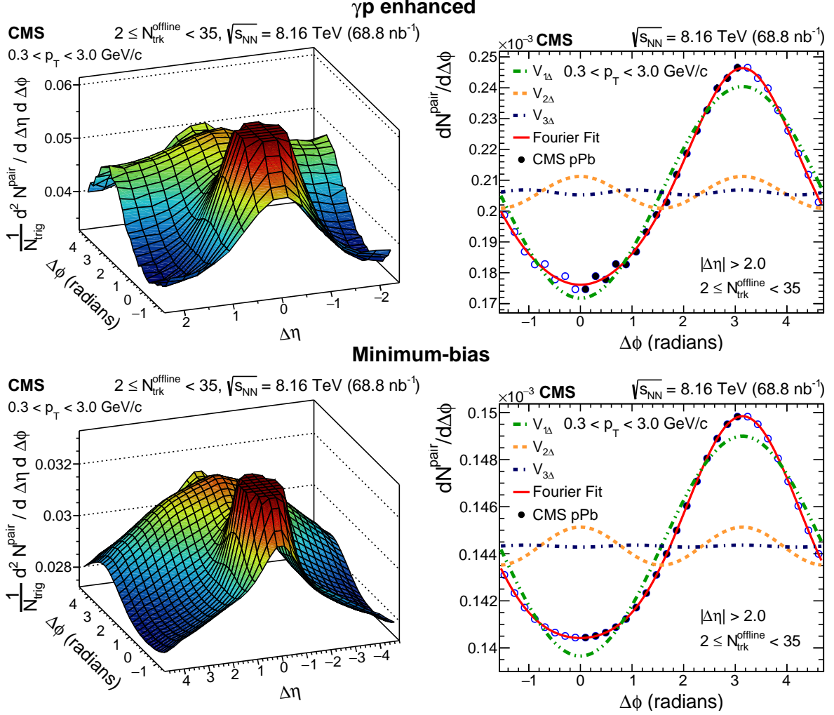
Figure 2: Two-dimensional (left) and one-dimensional (right) correlation plots for \gamma p -enhanced (upper) and MB (lower) events for 0.3 < p_{\text{T}} < 3.0 GeV/c and 2 \leq N_{\text{trk}}^{\text{offline}} < 35 . For the two-dimensional distributions, the jet peak centered at \Delta\eta = \Delta\phi = 0 is truncated to increase visibility. The rapidity gap requirement for the \gamma p -enhanced sample limits the |\Delta\eta| range to |\Delta\eta| < 2.5 . The one-dimensional \Delta\phi distributions are symmetrized by construction around \Delta\phi = 0 and \pi . The Fourier coefficients, V_{n\Delta} in the right column are fit over the \Delta\phi range [0, \pi] . Points outside this range are shown as open circles and are obtained by symmetrization of those in [0, \pi] . Statistical error bars are shown for both one-dimensional distributions.
