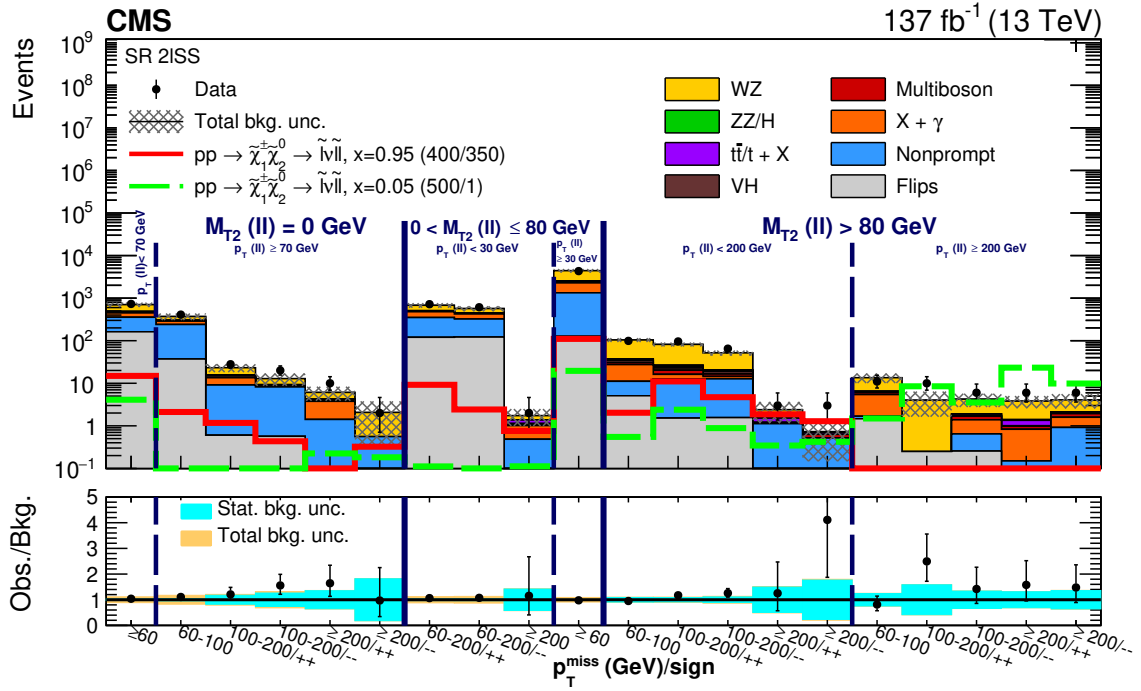
Figure 7. Observed and expected yields across the search regions in events with two same-sign light leptons ( 2\ell SS ). Several signal models are shown superimposed. They correspond to \tilde{\chi}_1^\pm \tilde{\chi}_2^0 production with slepton-mediated decays in the flavor-democratic hypothesis for a compressed \delta m = 50 GeV (red line) and uncompressed \delta m = 500 GeV (green dashed line) scenario. The legends specify the masses of \tilde{\chi}_2^0 and \tilde{\chi}_1^0 for the shown signal distributions as (m_{\tilde{\chi}_2^0}/m_{\tilde{\chi}_1^0}) .
