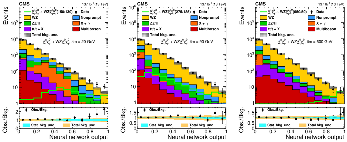
Figure 5. Observed and expected yields as functions of the output of the CMS neural network used to search for \tilde{\chi}_1^\pm \tilde{\chi}_2^0 production with WZ-mediated decays, evaluated at \delta m = 20 GeV (left), 90 GeV (center), and 600 GeV (right). The legends specify the masses of \tilde{\chi}_2^0 and \tilde{\chi}_1^0 for the shown signal distributions as (m_{\tilde{\chi}_2^0}/m_{\tilde{\chi}_1^0}) . The top panels show only the total uncertainty in the background prediction, while the lower panels show the total and statistical uncertainties separately. The following abbreviations are used in the legends of this and the following figures: “bkg.” stands for background, “unc.” for uncertainty and “obs.” for observed.
