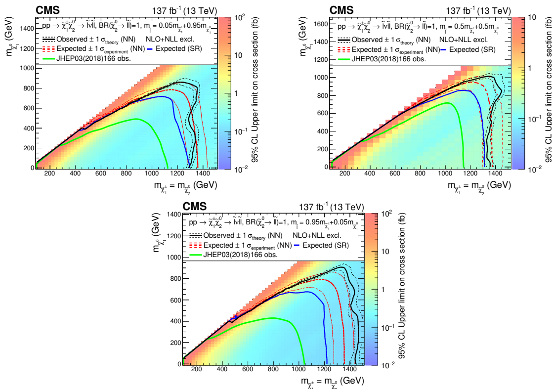
Figure 16. Interpretation of the results for \tilde{\chi}_1^{\pm} \tilde{\chi}_2^0 production with flavor-democratic slepton-mediated decays, and the parameter governing the mass splittings being x = 0.05 (upper left), x = 0.5 (upper right) and x = 0.95 (lower). The shading in the m_{\tilde{\chi}_1^0} versus m_{\tilde{\chi}_2^0} plane indicates the 95% CL upper limit on the \tilde{\chi}_1^{\pm} \tilde{\chi}_2^0 production cross sections. The contours delineate the mass regions excluded at 95% CL when assuming cross section computed at NLO plus NLL. All masses below the contours are excluded. The observed, observed \pm 1\sigma_{\text{theory}} ( \pm 1 standard deviation of the theoretical cross sections), median expected, and expected \pm 1\sigma_{\text{experiment}} bounds obtained with the neural network strategy are shown in black and red. The median expected bound obtained with the search region strategy is shown in blue. The observed limits obtained in the CMS analysis using 2016 data [20] are shown in green.
