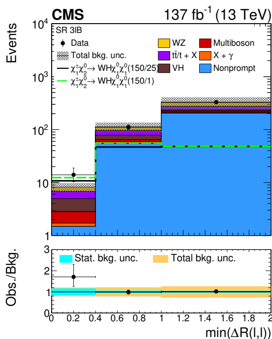
Figure 9. Observed and expected yields across the search regions in events with three light leptons, none of which form an OSSF pair (3lB). Several signal models are shown superimposed. They correspond to \tilde{\chi}_1^\pm \tilde{\chi}_2^0 production with WH-mediated decays for scenarios corresponding to a H boson like mass splitting \delta m = 125 GeV (black line) and a slightly less compressed \delta m = 150 GeV (green dashed line) scenario. The legends specify the masses of \tilde{\chi}_2^0 and \tilde{\chi}_1^0 for the shown signal distributions as (m_{\tilde{\chi}_2^0}/m_{\tilde{\chi}_1^0}) .
