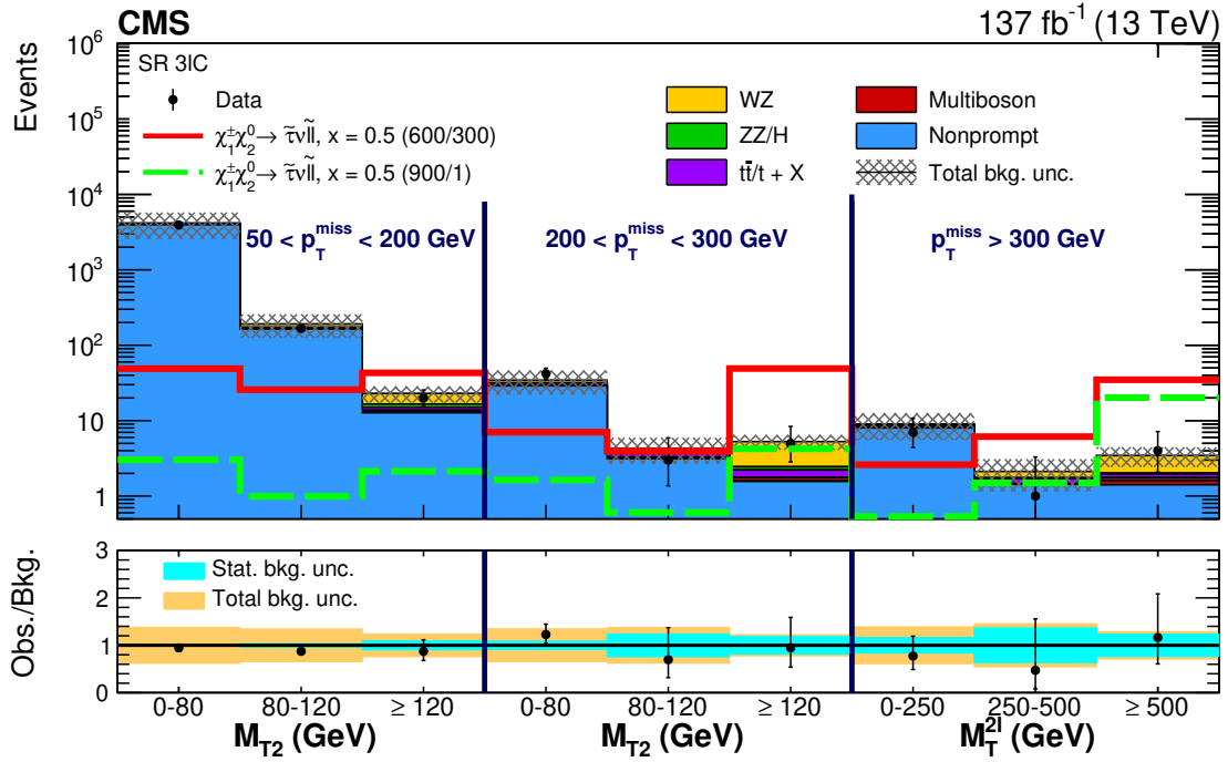
Figure 10. Observed and expected yields across the search regions in events with a \mu^+\mu^- or e^+e^- pair and an additional \tau_h candidate ( 3lC ). Several signal models are shown superimposed. They correspond to \tilde{\chi}_1^\pm\tilde{\chi}_2^0 production with slepton-mediated decays in the \tau lepton enriched hypothesis for a compressed \delta m = 300 GeV (red line) and uncompressed \delta m = 900 GeV (green dashed line) scenario. The legends specify the masses of \tilde{\chi}_2^0 and \tilde{\chi}_1^0 for the shown signal distributions as (\frac{m_{\tilde{\chi}_2^0}}{m_{\tilde{\chi}_1^0}}) .
