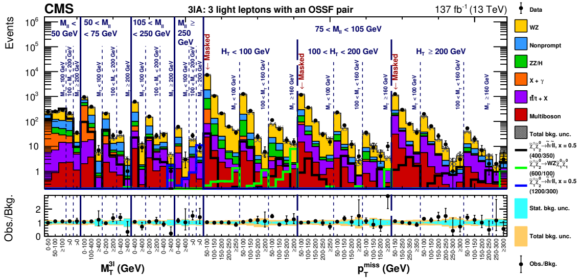
Figure 8. Observed and expected yields across the search regions in events with three light leptons, at least two of which form an OSSF pair ( 3lA ). Several signal models are shown superimposed. They correspond to \tilde{\chi}_1^{\pm}\tilde{\chi}_2^0 production with slepton-mediated decays in the flavor-democratic hypothesis for a compressed \delta m = 50 GeV (black line) and uncompressed \delta m = 900 GeV (blue line) scenario, and for WZ-mediated decays in an uncompressed \delta m = 500 GeV scenario (green line). Bins labeled as “Masked” are not considered in the interpretation of the results because of overlap with the WZ control region. The legends specify the masses of \tilde{\chi}_2^0 and \tilde{\chi}_1^0 for the shown signal distributions as (m_{\tilde{\chi}_2^0}/m_{\tilde{\chi}_1^0}) .
