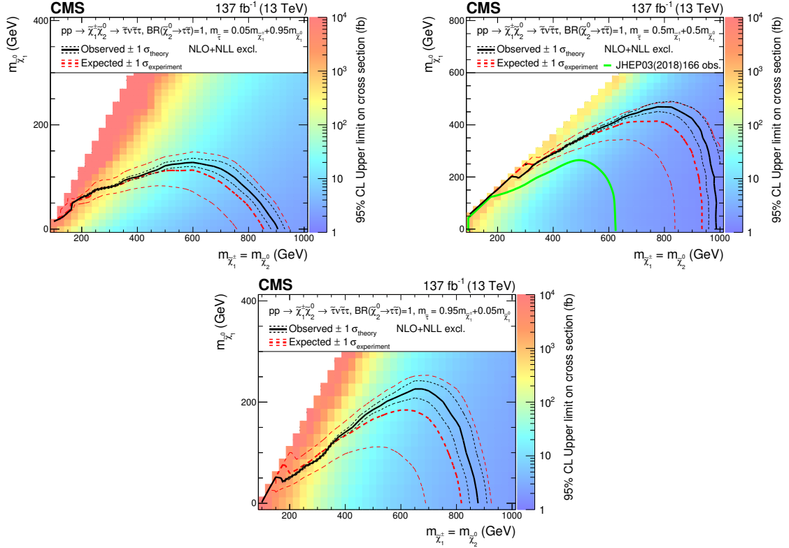
Figure 18. Interpretation of the results for \tilde{\chi}_1^{\pm} \tilde{\chi}_2^0 production with \tau -dominated slepton-mediated decays, and the parameter governing the mass splittings being x = 0.05 (upper left), x = 0.5 (upper right) and x = 0.95 (lower). The shading in the m_{\tilde{\chi}_1^0} versus m_{\tilde{\chi}_2^0} plane indicates the 95% CL upper limits on the \tilde{\chi}_1^{\pm} \tilde{\chi}_2^0 production cross sections. The contours delineate the mass regions excluded at 95% CL when assuming cross sections computed at NLO plus NLL. The observed, observed \pm 1\sigma_{\text{theory}} ( \pm 1 standard deviation of the theoretical cross sections), median expected, and expected \pm 1\sigma_{\text{experiment}} bounds are shown in black and red. The median expected bound obtained with the search region strategy is shown in blue. The observed limits obtained in the CMS analysis using 2016 data [20] are shown in green, which only included interpretations in the x = 0.5 case.
