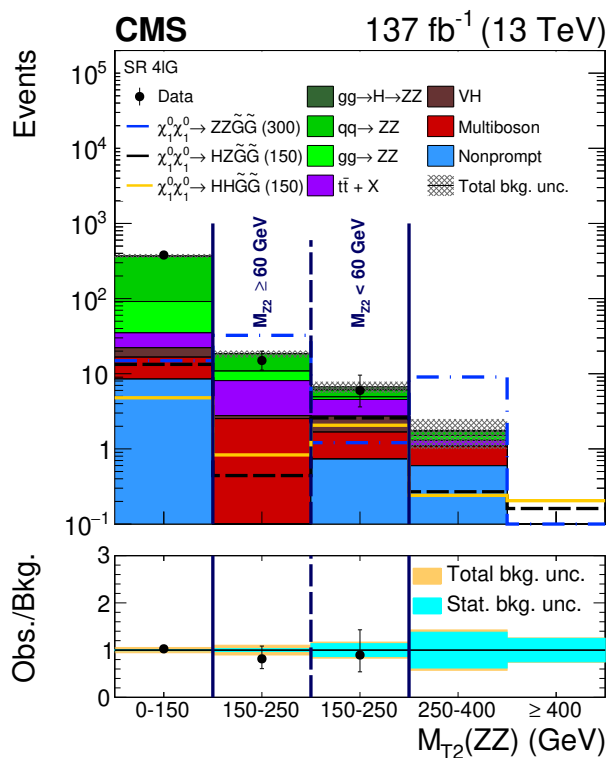
Figure 13. Observed and expected yields across the search regions in events with four light leptons, including 2 separate OSSF pairs ( 4lG ). Several signal models are shown superimposed. They correspond to Higgsino pair production with decays to ZZ (blue dotted line, Higgsino mass of 300 GeV), HZ (black dashed line, Higgsino mass of 150 GeV), and HH (dark yellow line, Higgsino mass of 150 GeV).
