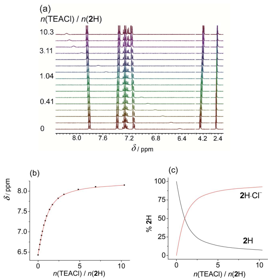
Fig. 1 (a) 1 H NMR titration of 2H ( c = 1.15 \times 10^{-3} \text{ mol dm}^{-3} ) with TEACl ( c = 2.10 \times 10^{-2} \text{ mol dm}^{-3} ) in MeCN- d_3 at (25.0 \pm 0.1)^\circ\text{C} , V_0 = 0.53 \text{ mL} . (b) Dependence of \text{NH}_b proton chemical shift on n(\text{TEACl})/n(2\text{H}) molar ratio. ■ Experimental, – calculated. (c) Distribution of species during the titration of 2H with TEACl.
