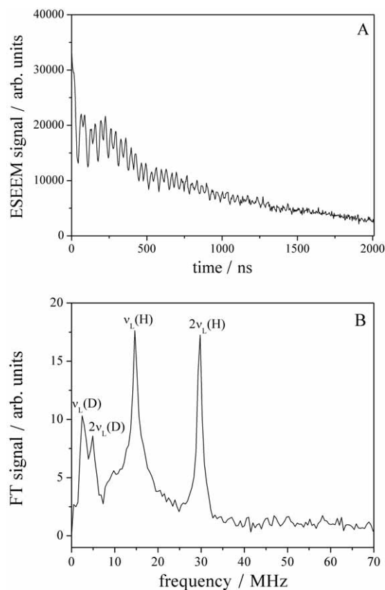
Figure 1. A – Time domain ESEEM, and B – FT-ESEEM spectra of 5-SASL incorporated in multi-lamellar liposomes (egg-PC : DHP = 7 : 1) in 0.1 \text{ mol dm}^{-3} phosphate buffer ( D_2O , pH = 7.1). Spectra were taken at 35 K.
