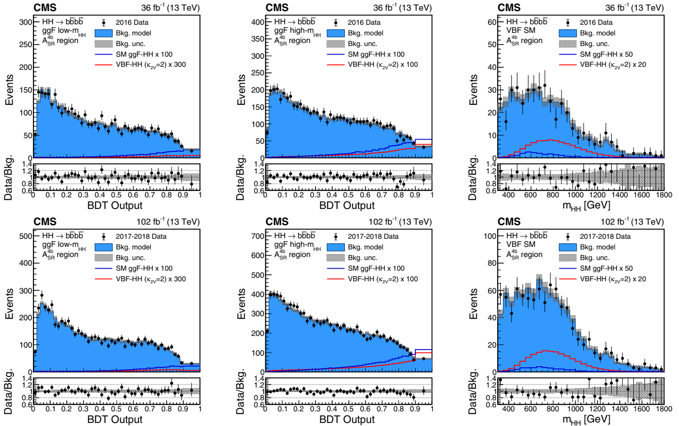
FIG. 1. Distributions of the events observed in the A_{SR}^{4b} signal region for 2016 (top) and 2017–2018 (bottom) data. The two leftmost columns show the BDT output in the low- and high-mass categories, and the rightmost column shows the m_{HH} distribution in the VBF SM-like category.
