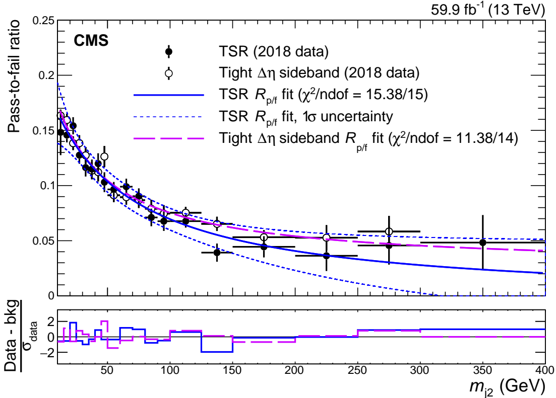
Figure 2: Distributions of the ratio of event passing and failing the D_{j_2}^{\text{bb}} > 0.6 requirement, as a function of the subleading jet groomed mass m_{j_2} , in 2018 data, for the TSR (filled markers) and the tight |\Delta\eta| sidebands (open markers). The arctangent R_{p/f} fit from which the background is estimated is shown by the solid line in the case of the TSR, and by the thick dashed line for the sideband, with the resulting \chi^2 and degrees of freedom indicated in the legend. The 1\sigma uncertainty band of the fit in the TSR, from which systematic uncertainties on the QCD background estimate are derived, is shown by the thin dashed lines. Similar results were obtained for 2016 and 2017 data and in the three LSRs. The lower panel shows the difference between the observed data and the fits, divided by the statistical uncertainty of the ratio of passing and failing events in the data for each bin.
