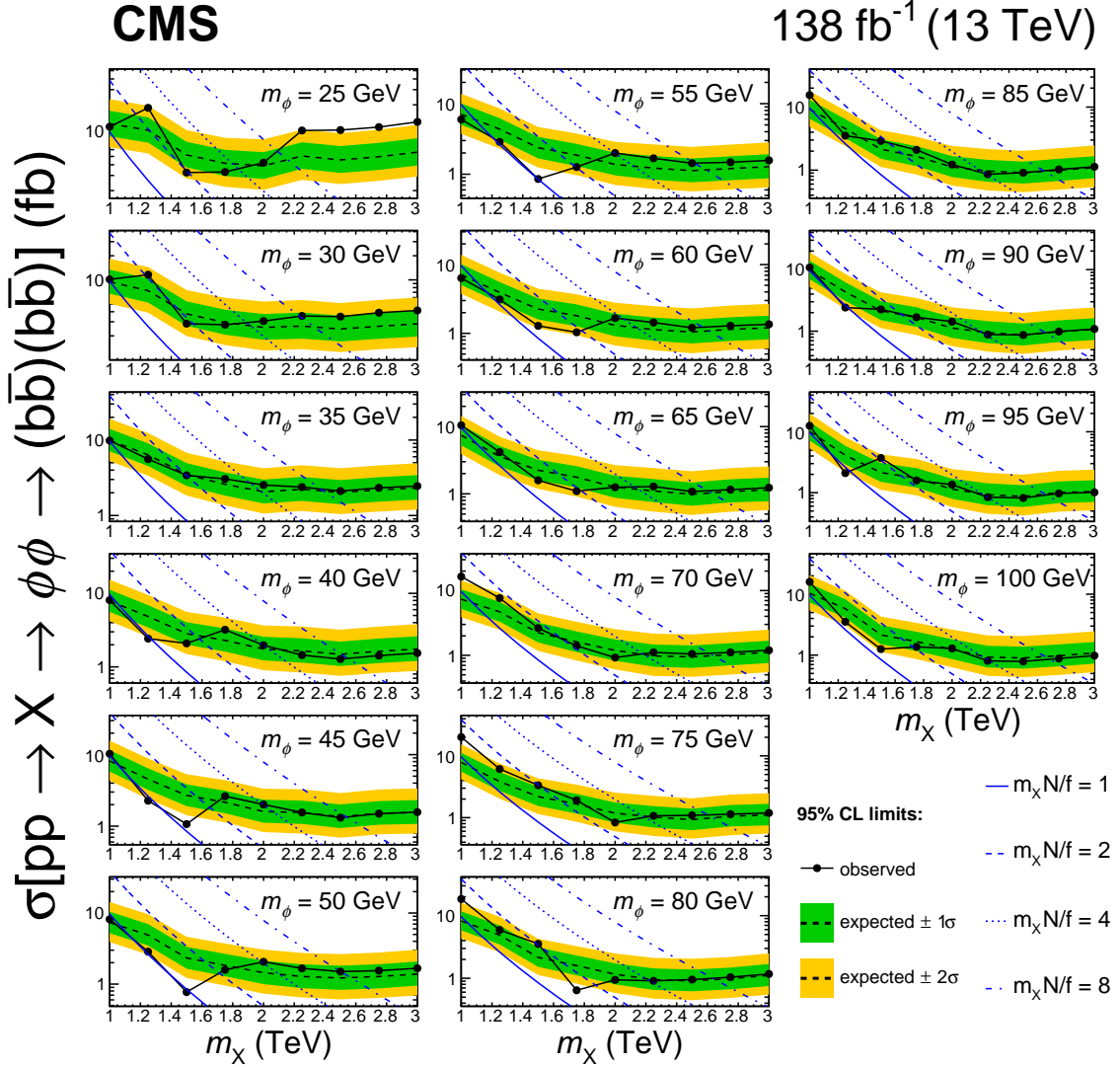
Figure 5: Upper limits at 95% CL on the cross section of the process pp \rightarrow X \rightarrow \phi\phi \rightarrow (b\bar{b})(b\bar{b}) , as a function of the mass of m_\chi , for different values of m_\phi . Both the X \rightarrow \phi\phi and \phi \rightarrow b\bar{b} branching fractions are assumed to be 100%. Each subpanel shows the limits for a fixed value of m_\phi . The observed limits are shown as solid black lines with markers, while the expected limits are dotted. The yellow (outer) and green (inner) bands represent one and two standard deviation intervals. The theoretical cross section for different values of the parameter m_\chi N/f are shown with dotted and dashed curves.
