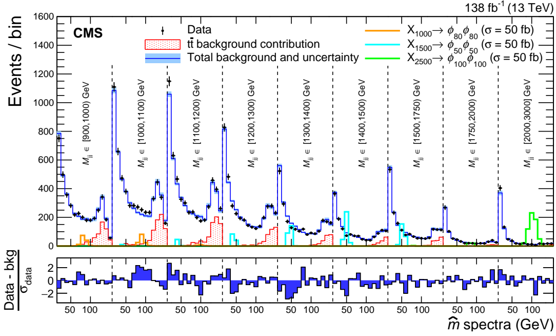
Figure 4: The average jet mass distributions in consecutive dijet mass intervals. The vertical dashed lines separate the average jet mass distributions in each bin of M_{jj} . The individual bins within such subdivisions correspond to the \hat{m} spectrum (from 15 to 200 GeV), as seen in Fig. 3 (left). Representative signal shapes are also shown; we note that they peak in the \hat{m} spectrum within subdivisions, and may appear in multiple M_{jj} bins. The blue (solid) line represents the sum of the estimated QCD and t\bar{t} backgrounds, and the red filled histogram shows the t\bar{t} contribution alone. The shaded areas around the background estimate in the upper panels represent the total uncertainty in the total background estimate in that bin. The shapes of three representative signals, each normalized to cross sections of 50 fb are indicated by solid colored lines. The lower panel shows the difference between the observed data and the background prediction, divided by \sigma_{\text{data}} , the statistical uncertainty of the data in each bin.
