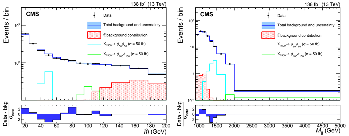
Figure 3: Distributions of average jet mass (left) and dijet mass (right), and background estimate of the combined search regions after the final fit is performed. The blue (solid) line represents the sum of the estimated QCD and t\bar{t} backgrounds, and the red filled histogram shows the t\bar{t} contribution alone. The shaded areas around the background estimate in the upper panels represent the total uncertainty in the total background estimate in that bin. The shapes of two representative signals, each normalized to cross sections of 50 fb, are indicated by solid colored lines. The lower panel shows the difference between the observed data and the background prediction, divided by \sigma_{\text{data}} , the statistical uncertainty of the data in each bin.
