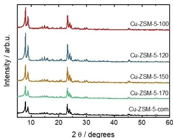
Figure 1. XRD patterns of Cu-containing ZSM-5 (sample labels as in Table 1).
