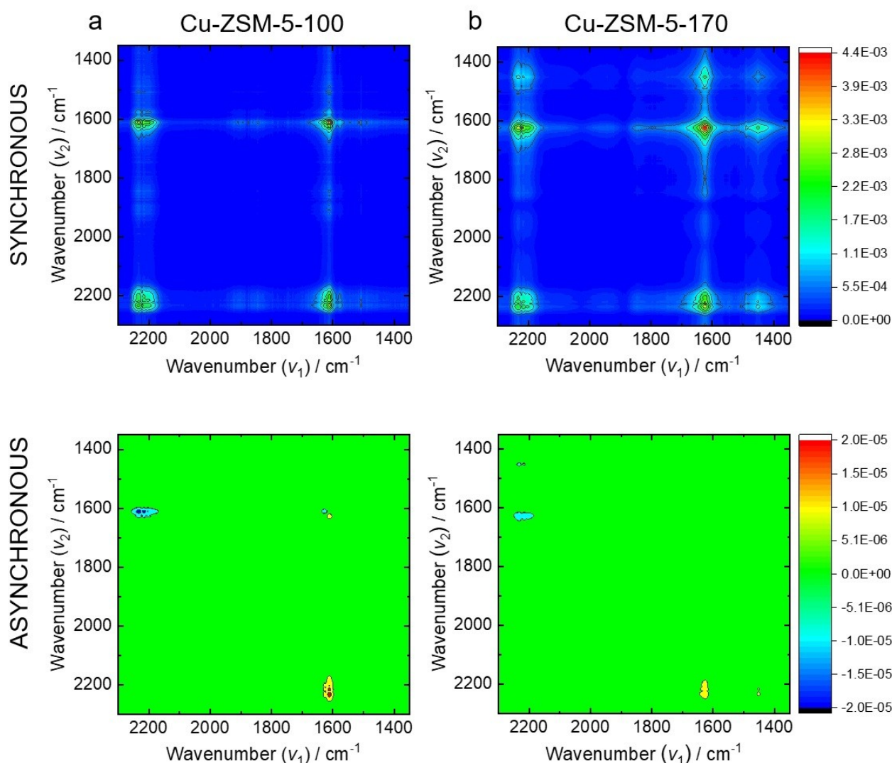
Figure 11. The 2D correlation IR spectra presenting N–O region collected upon the contact of the c(\text{NO}):c(\text{O}_2):c(\text{NH}_3):c(\text{H}_2\text{O}) = 4:1:4:8 mixture with a) Cu-ZSM-5-100 and b) Cu-ZSM-5-170 at 120 °C for 13 min.
