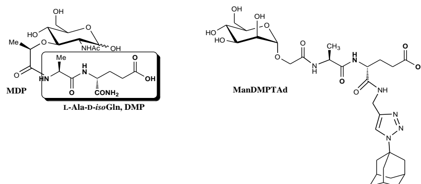
Figure 1. Structure of MDP, DMP and mannosylated adamantyl-triazole DMP derivative.
