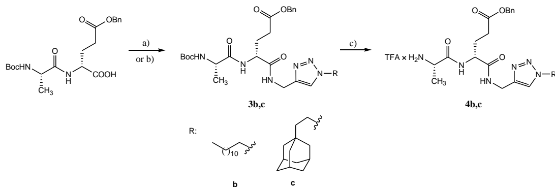
Scheme 3. Reagents and conditions: (a) 2b , HBTU, TEA, THF/dry \text{CH}_2\text{Cl}_2 , Ar (g), rt, 24 h, 53% ( 3b ); (b) (i) 2c , n -butyl chloroformate/ N -methylmorpholine, THF/dry \text{CH}_2\text{Cl}_2 , Ar (g), -10^\circ\text{C} to rt, 3 h; (ii) \text{NaHCO}_3 (aq), rt, 65% ( 3c ); (c) TFA, dry \text{CH}_2\text{Cl}_2 , rt, 4 h, yield: 82% ( 4b ), 89% ( 4c ).
