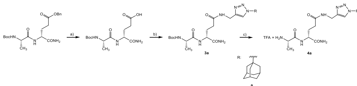
Scheme 2. Reagents and conditions: (a) \text{H}_2 , 10% Pd/C, MeOH, 34 psi, overnight, 95%; (b) 2a , EDC \times HCl, HOBT, TEA, 1,4-dioxane/ \text{CH}_2\text{Cl}_2 , 0^\circ\text{C} to rt, 48 h, 71%; (c) TFA, dry \text{CH}_2\text{Cl}_2 , rt, 2.5 h, 95%.
