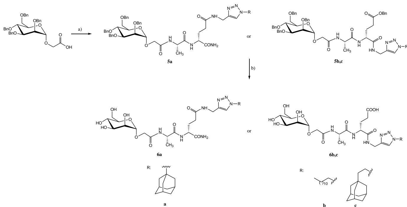
Scheme 4. Reagents and conditions: (a) 4a–c , EDC \times HCl, HOBt, TEA, 1,4-dioxane/ \text{CH}_2\text{Cl}_2 , 0^\circ\text{C} to rt, 48 h, yield: 60% ( 5a ), 69% ( 5b ), 57% ( 5c ); (b) \text{H}_2 , 10% Pd/C, 96% EtOH, 40 psi, rt, 24 h, yield: 60% ( 6a ), 76% ( 6b ), 67% ( 6c ).
