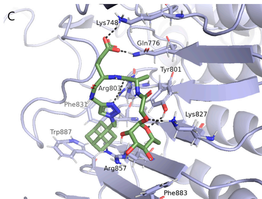
Figure 4. Molecular docking of ManDMPTAd (A), 6b (B) and 6c (C) in the proposed binding pocket on the concave surface of the LRR domain of NOD2. The stick model of different colors shows selected ligands, and the key amino acid residues of the NOD2 receptor around compounds have been displayed in the light blue stick model. Hydrogen bonds are shown as dark gray dashed lines.
