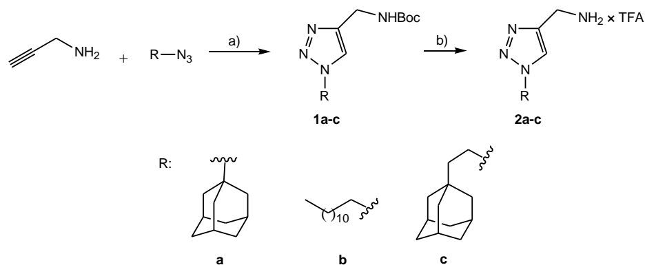
Scheme 1. Reagents and conditions: (a): (i) \text{Boc}_2\text{O} , TEA, 1,4-dioxane, \text{H}_2\text{O} , 0^\circ\text{C} to rt, 90 min; (ii) \text{R-N}_3 , Na ascorbate (aq), \text{CuSO}_4 \times 5 \text{H}_2\text{O} (aq), Ar, 35^\circ\text{C} , 24 h, yield: 97% ( 1a ), 58% ( 1b ), 53% ( 1c ); (b) TFA, dry \text{CH}_2\text{Cl}_2 , rt, 2–4 h; yield: 87% ( 2a ), 96% ( 2b ), 75% ( 2c ).
