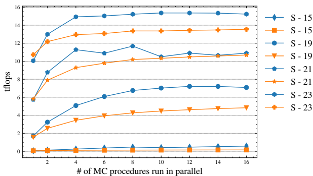
Fig. 4: The performance in TFLOPS/s of the entire simulation as a function of the number of MC procedures for batch (orange) and task (blue).
