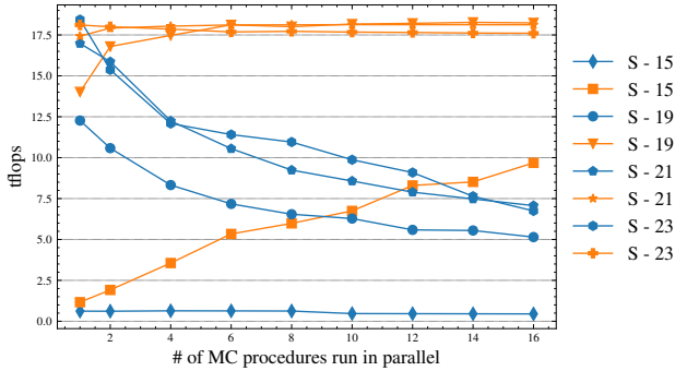
Fig. 3: Performance of the single GEMM operation as a function of the number of MC procedures for batch (orange) and task (blue) variants.
