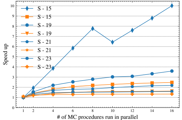
Fig. 2: Speedup of batched (orange) and tasked (blue) variants compared to the sequential execution for a given number of MC procedures on a single GPU.
