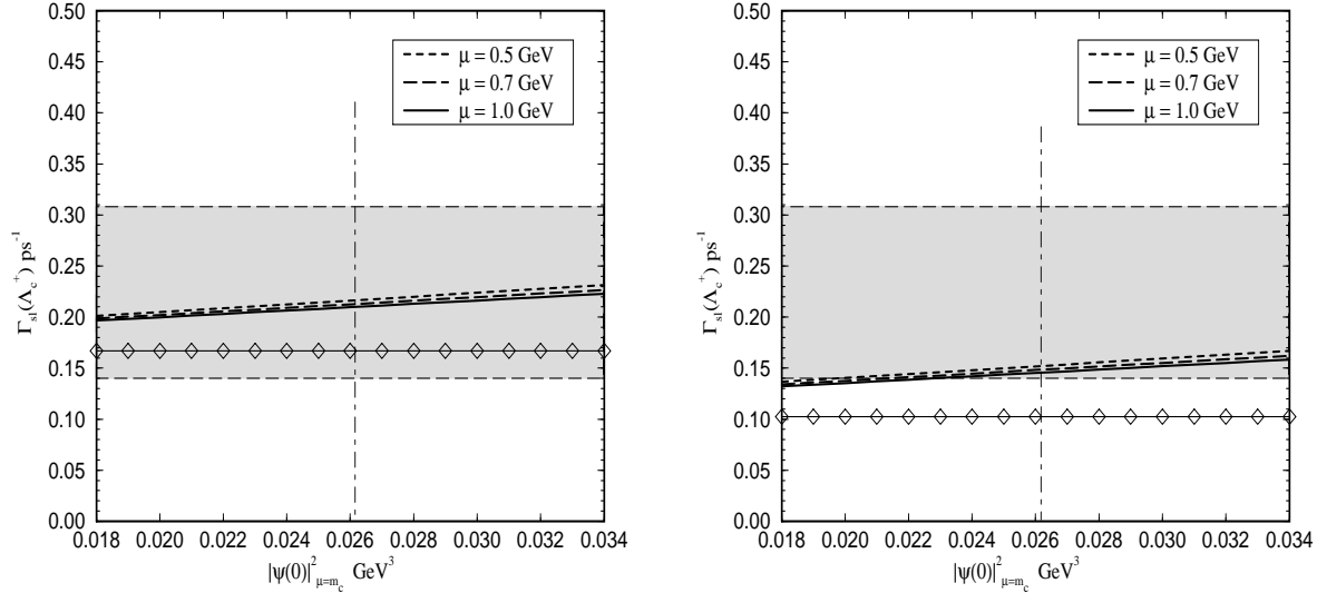
Figure 3: Semileptonic \Lambda_c^+ -decay rate for three values of the hybrid renormalization point \mu is given as a function of the square of the baryon wave function |\psi(0)|^2 . On the left picture finite \alpha_s -contributions are not included. The vertical dot-dashed line denotes the 'central' value in (17). The shaded area is the experimentally allowed region. \diamond denotes the semileptonic decay rate without Voloshin's contributions. The other parameter values used are m_c = 1.4 \text{ GeV} , \Lambda_{QCD} = 300 \text{ MeV} , \mu_\pi^2 = 0.1 \text{ GeV}^2 .
