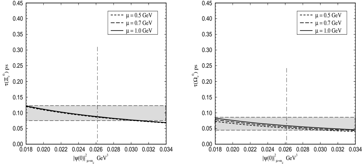
Figure 2: Lifetimes of \Xi_c^0 and \Omega_c^0 as a function of the square of the baryon wave function |\psi(0)|^2 given for three values of the hybrid renormalization point \mu . The shaded areas are the experimentally allowed regions. The dash-dotted vertical line is a value of |\psi(0)|^2 used in Tables 1 to 2. The results are obtained using m_c = 1.4 \text{ GeV} , \Lambda_{QCD} = 300 \text{ MeV} , \mu_\pi^2 = 0.1 \text{ GeV}^2 , \mu_G^2(\Omega_c^0) = 0.182 \text{ GeV}^2 .
