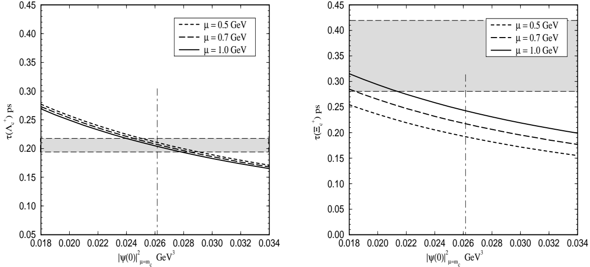
Figure 1: Lifetimes of \Lambda_c^+ and \Xi_c^+ as a function of the square of the baryon wave function |\psi(0)|^2 , given for three values of the hybrid renormalization point \mu . The shaded areas are the experimentally allowed regions. The dot-dashed vertical line is a value of |\psi(0)|^2 used in Tables 1 to 2. The results are obtained using m_c = 1.4 \text{ GeV} , \Lambda_{QCD} = 300 \text{ MeV} , \mu_\pi^2 = 0.1 \text{ GeV}^2 .
