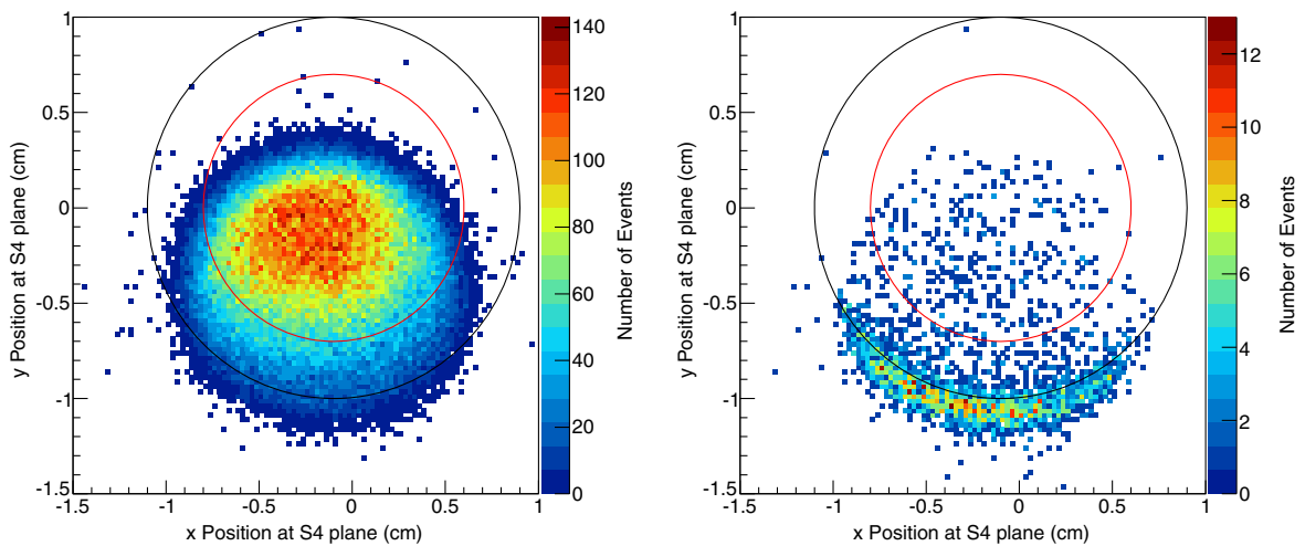
FIG. 3. Positions of BPD tracks extrapolated to the S4 plane in target removed data runs from the \pi^+ + C at 31 GeV/ c data set. The measured S4 position is shown as a black circle and the BPD radius cut is shown as a red circle in both figures. (Left) Events taken by the beam trigger. (Right) Events taken by the interaction trigger.
