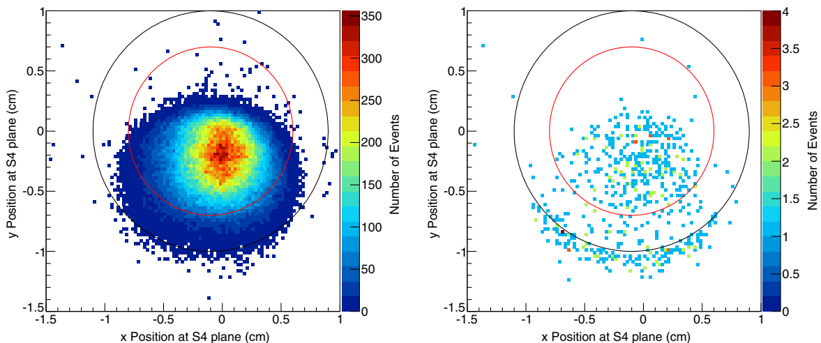
FIG. 4. Positions of BPD tracks extrapolated to the S4 plane in target removed data runs from the \pi^+ + C at 60 GeV/ c data set. The measured S4 position is shown as a black circle and the BPD radius cut is shown as a red circle in both figures. (Left) Events taken by the beam trigger. (Right) Events taken by the interaction trigger.
