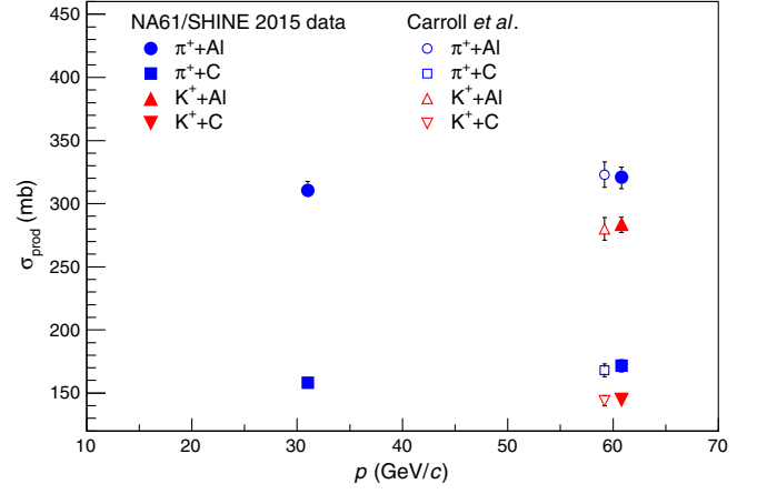
FIG. 7. Summary of production cross section measurements. The results are compared to previous results obtained with a beam momentum of 60 GeV/c by Carrol et al. [15].
