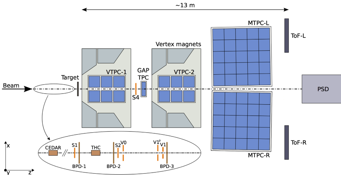
FIG. 1. The schematic top-view layout of the NA61/SHINE experiment in the configuration used during the 2015 data taking. The two superconducting vertex magnets were not operational during the data-taking period.
