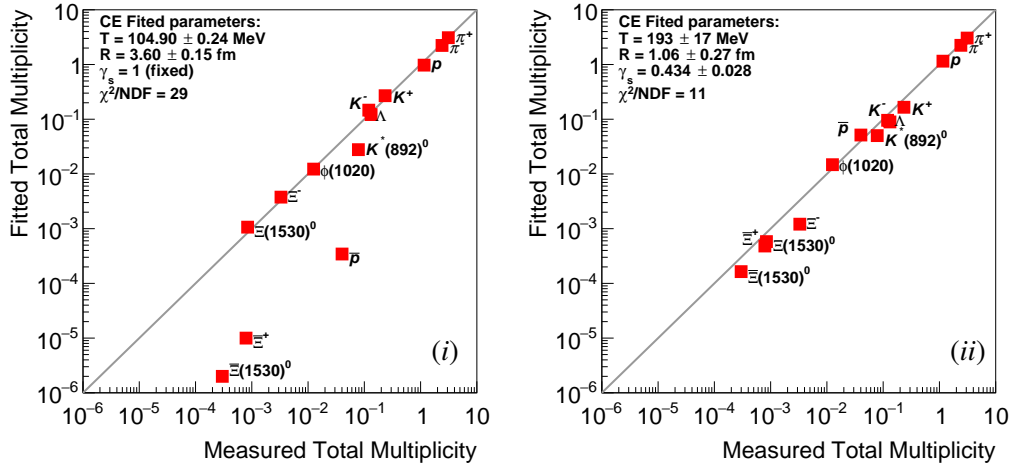
Figure 11: (Color online) Mean multiplicities of \pi^+ , \pi^- , K^+ , K^- , p , \bar{p} , K^*(892)^0 , \Lambda , \phi(1020) , \Xi^- , \Xi\bar{\Xi}^+ , \Xi(1530)^0 and \Xi\bar{\Xi}(1530)^0 produced in p+p interactions at 158 GeV/c [3, 4, 17, 18, 19, 20, 12] measured by NA61/SHINE are compared with mean multiplicities obtained from the HRG model based on the Canonical Ensemble with fixed \gamma_s = 1 (i) and fitted \gamma_s (ii). Uncertainties of the measurements are smaller than the size of the markers.
