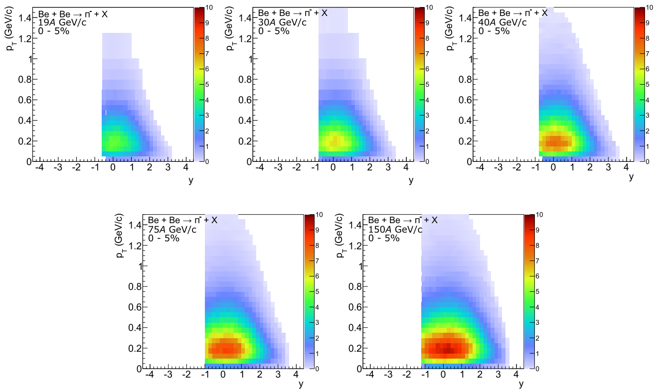
Fig. 10 Double-differential spectra \frac{d^2n}{dydp_T} of negatively charged pions produced in the 5% most central Be + Be collisions at beam momenta of 19A, 30A, 40A, 75A and 150A GeV/c
