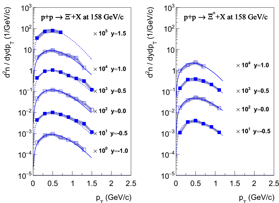
Fig. 4 Transverse momentum spectra in rapidity slices of \Xi^- (left) and \Xi^+ (right) produced in inelastic p+p interactions at 158 GeV/c. Rapidity values given in the legends correspond to the middle of the corresponding interval. Statistical uncertainties are smaller than the marker size, shaded bands show systematic uncertainties. Spectra are scaled by the given factors for better separation
