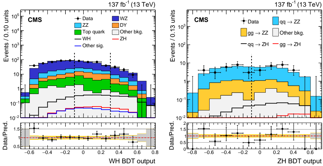
Figure 8: The observed BDT output distribution in the WH (left) and ZH (right) categories compared to the prediction from the simulation of various SM background processes. Signal distributions expected from different production modes of the Higgs boson with m_H = 125 GeV are overlaid. The description of the ratio panel is the same as in Fig. 4. The dashed vertical lines indicate the boundaries of the optimized event categories.
