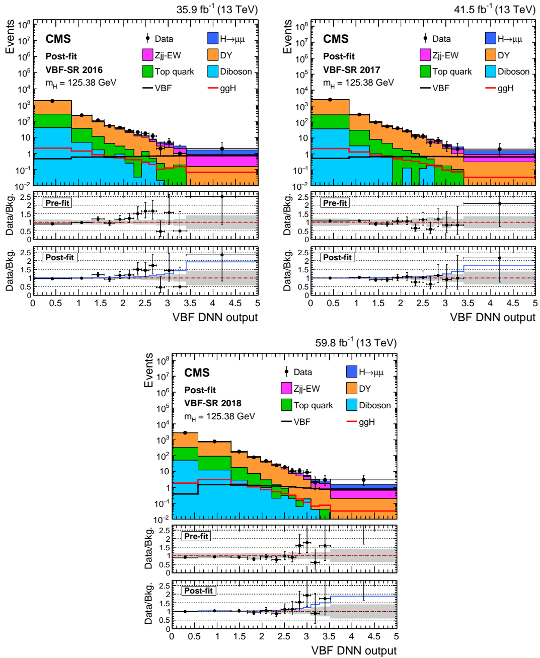
Figure 1: The observed DNN output distribution in the VBF-SR region for data collected in 2016 (first row, left), 2017 (first row, right), and 2018 (second row) compared to the post-fit background estimate for the contributing SM processes. The post-fit distributions for the Higgs boson signal produced via ggH (solid red) and VBF (solid black) modes with m_H = 125.38 GeV are overlaid. The predicted backgrounds are obtained from a S+B fit performed across analysis regions and years. In the middle panel, the ratio between data and the pre-fit background prediction is shown. The grey band indicates the total pre-fit uncertainty obtained from the systematic sources previously described. The lower panel shows the ratio between data and the post-fit background prediction from the S+B fit. The grey band indicates the total background uncertainty after performing the fit. The blue histogram (upper panel) and solid line (lower panel) indicate the total signal extracted from the fit with m_H = 125.38 GeV.
