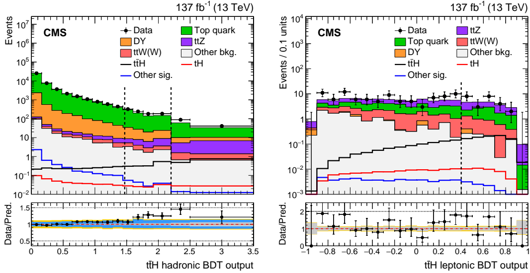
Figure 6: The observed BDT output distribution in the t\bar{t}H hadronic (left) and leptonic (right) categories compared to the prediction from the simulation of various SM background processes. Signal distributions expected from different production modes of the Higgs boson with m_H = 125 GeV are overlaid. The dashed vertical lines indicate the boundaries of the optimized event categories. The description of the ratio panels is the same as in Fig. 4.
