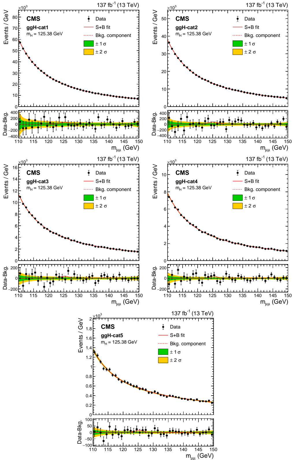
Figure 5: Comparison between the data and the total background extracted from a S+B fit performed across the various ggH subcategories. The one (green) and two (yellow) standard deviation bands include the uncertainties in the background component of the fit. The lower panel shows the residuals after background subtraction and the red line indicates the signal with m_H = 125.38 \text{ GeV} extracted from the fit.
