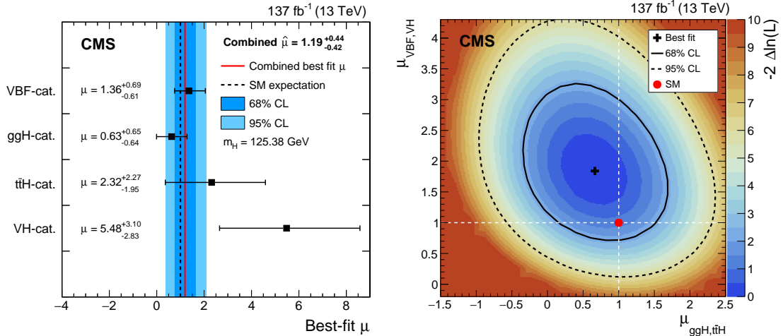
Figure 11: Left: signal strength modifiers measured for m_H = 125.38\text{ GeV} in each production category (black points) are compared to the result of the combined fit (solid red line) and the SM expectation (dashed grey line). Right: scan of the profiled likelihood ratio as a function of \mu_{\text{ggH},t\bar{t}H} and \mu_{\text{VBF},\text{VH}} with the corresponding 1\sigma and 2\sigma uncertainty contours. The black cross indicates the best fit values (\hat{\mu}_{\text{ggH},t\bar{t}H}, \hat{\mu}_{\text{VBF},\text{VH}}) = (0.66, 1.84) , while the red circle represents the SM expectation.
