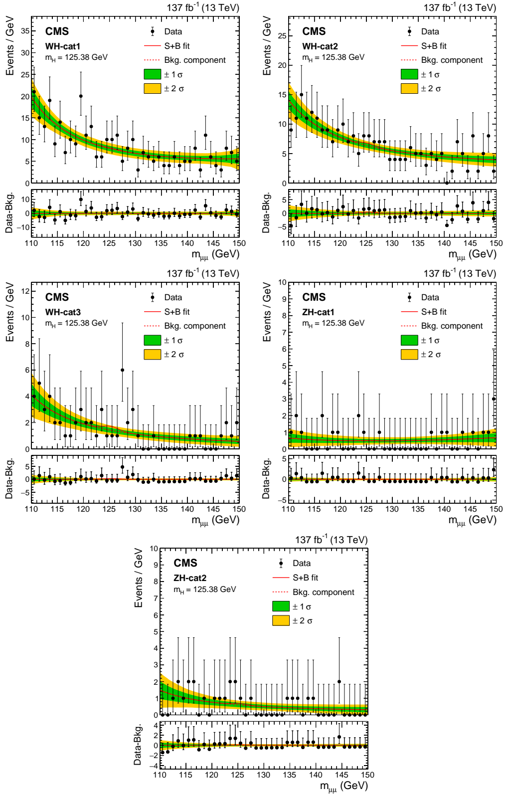
Figure 9: Comparison between the data and the total background extracted from a S+B fit performed across the various WH and ZH event subcategories. The one (green) and two (yellow) standard deviation bands include the uncertainties in the background component of the fit. The lower panel shows the residuals after the background subtraction, where the red line indicates the signal with m_H = 125.38 GeV extracted from the fit.
