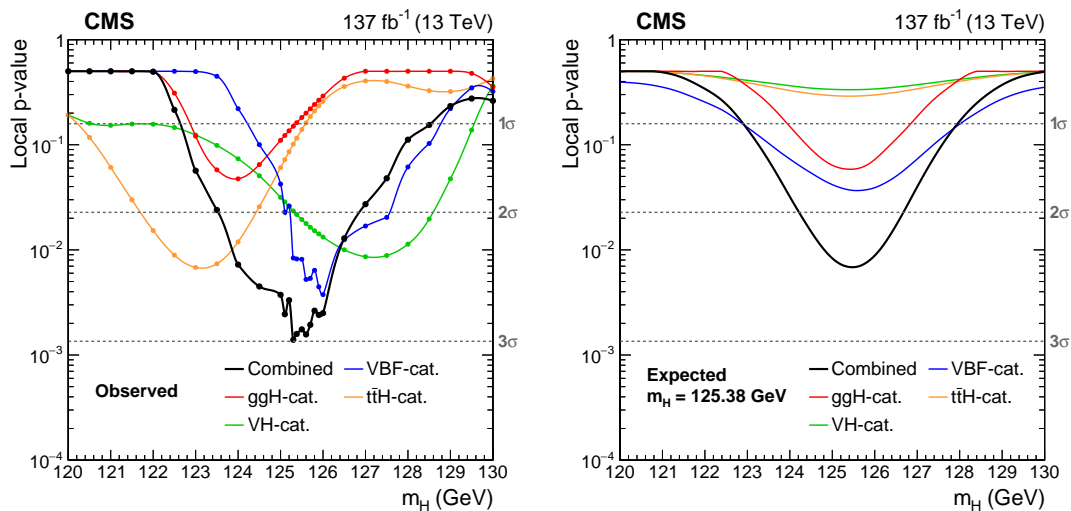
Figure 10: Left: observed local p -values as a function of m_H , extracted from the combined fit as well as from each individual production category, are shown. The solid markers indicate the mass points for which the observed p -values are computed. Right: the expected p -values are calculated using the background expectation obtained from the S+B fit and injecting a signal with m_H = 125.38 GeV and \mu = 1 .
