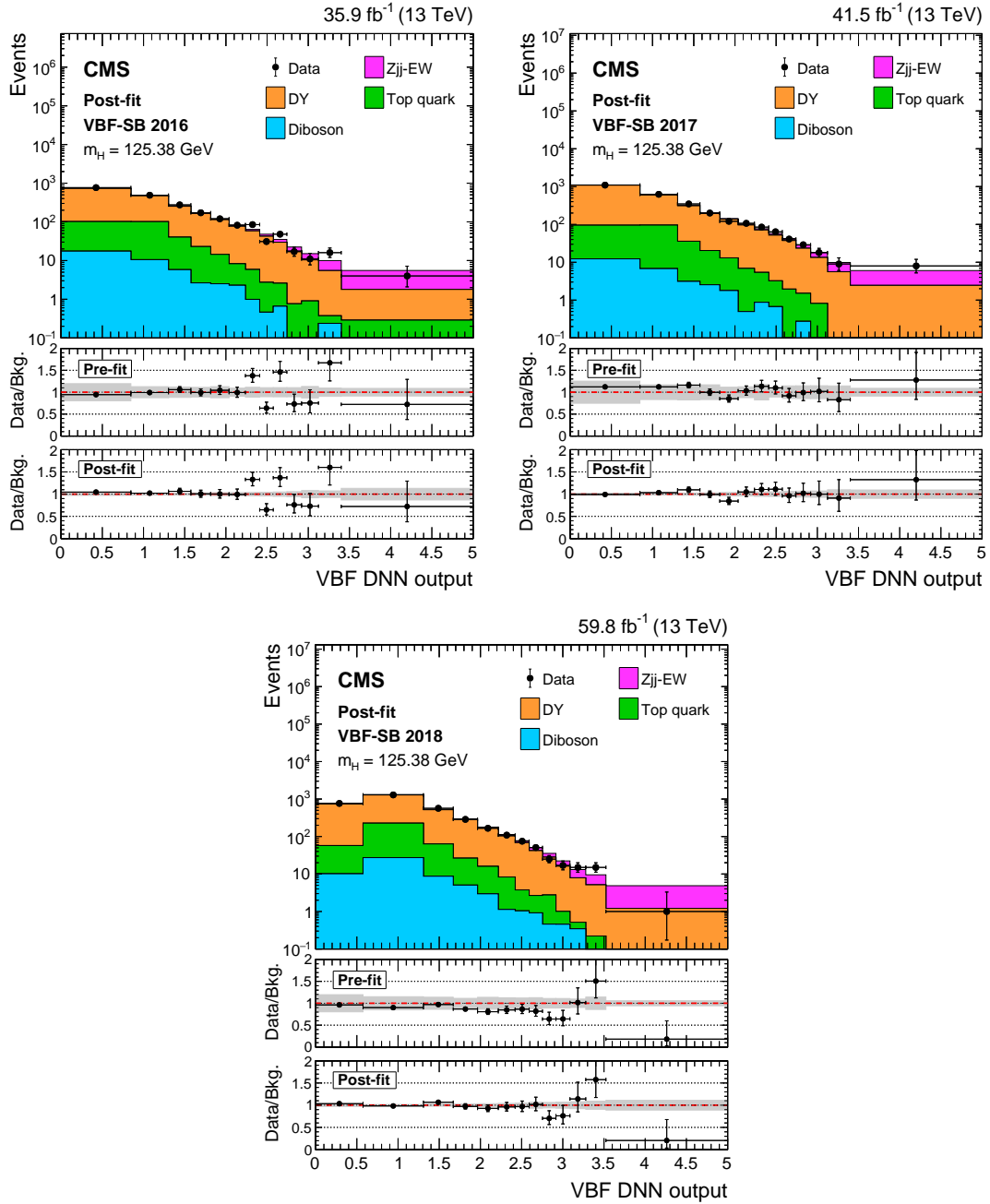
Figure 2: The observed DNN output distribution for data collected in 2016 (first row, left), 2017 (first row, right), and 2018 (second row) in the VBF-SB region compared to the post-fit background estimate from SM processes. The predicted backgrounds are obtained from a S+B fit performed across analysis regions and years. The description of the three panels is the same as in Fig. 1.
