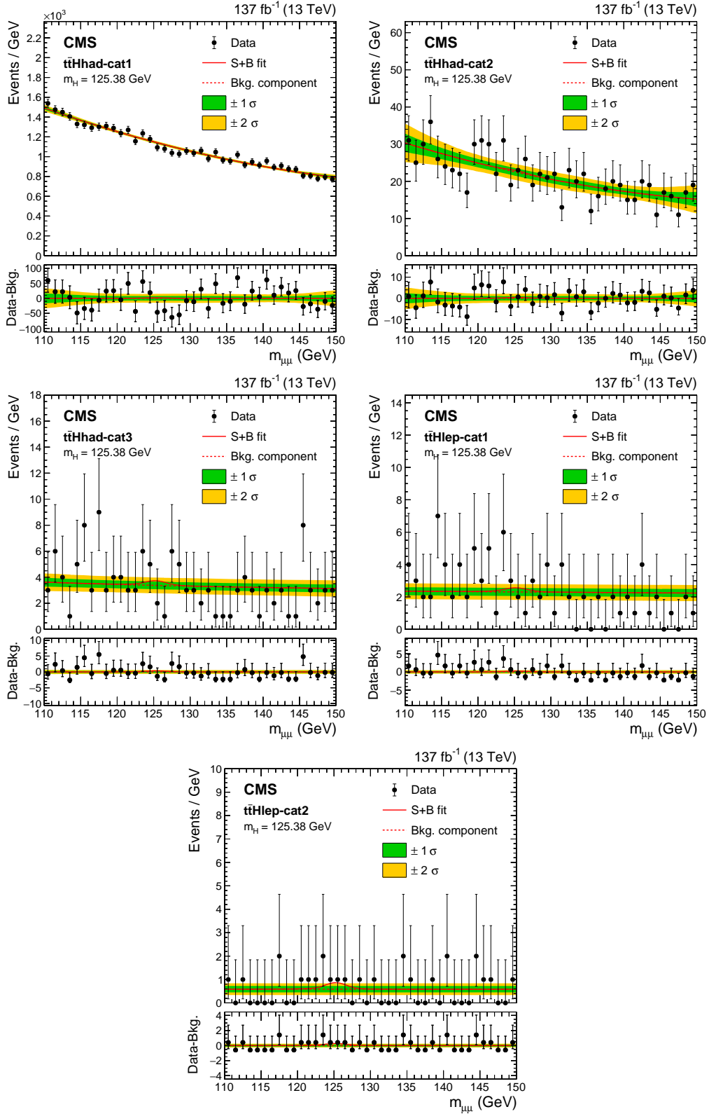
Figure 7: Comparison between the data and the total background extracted from a S+B fit performed across the various t\bar{t}H hadronic and leptonic event subcategories. The one (green) and two (yellow) standard deviation bands include the uncertainties in the background component of the fit. The lower panel shows the residuals after the background subtraction, where the red line indicates the signal with m_H = 125.38 GeV extracted from the fit.
