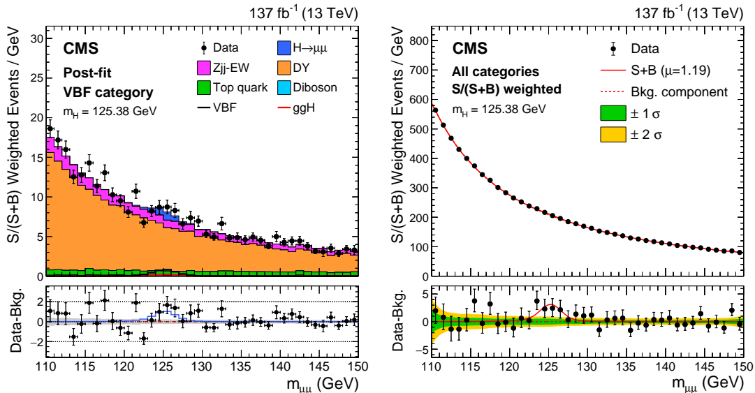
Figure 12: Left: the m_{\mu\mu} distribution for the weighted combination of VBF-SB and VBF-SR events. Each event is weighted proportionally to the S/(S+B) ratio, calculated as a function of the mass-decorrelated DNN output. The lower panel shows the residuals after subtracting the background prediction from the S+B fit. The best fit H \rightarrow \mu^+\mu^- signal contribution is indicated by the blue line and histogram, while the grey band indicates the total background uncertainty from the background-only fit. Right: the m_{\mu\mu} distribution for the weighted combination of all event categories. The lower panel shows the residuals after background subtraction, with the best fit SM H \rightarrow \mu^+\mu^- signal contribution for m_H = 125.38 GeV indicated by the red line.
