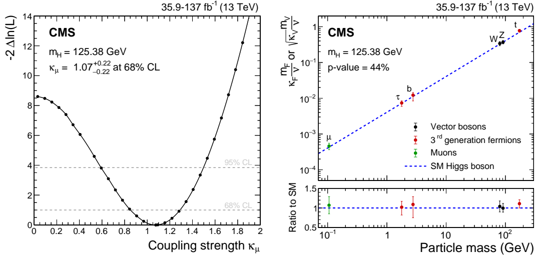
Figure 14: Left: the observed profile likelihood ratio as a function of \kappa_\mu for m_H = 125.38 GeV, obtained from a combined fit with Ref. [10] in the \kappa -framework. The best fit value for \kappa_\mu is 1.07 and the corresponding observed 68% CL interval is 0.85 < \kappa_\mu < 1.29 . Right: the best fit estimates for the reduced coupling modifiers extracted for fermions and weak bosons from the resolved \kappa -framework compared to their corresponding prediction from the SM. The error bars represent 68% CL intervals for the measured parameters. In the lower panel, the ratios of the measured coupling modifiers values to their SM predictions are shown.
