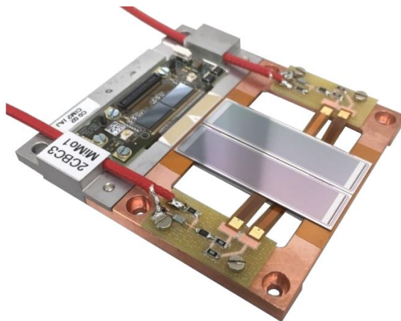
Figure 8. One of the three mini-modules assembled for the DESY beam test.
