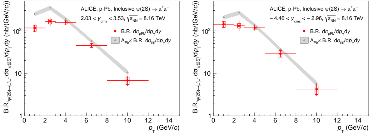
Figure 3: The differential cross sections \text{B.R.}_{\psi(2S) \rightarrow \mu^+ \mu^-} \cdot d^2\sigma^{\psi(2S)}/dy dp_T for p–Pb collisions at \sqrt{s_{\text{NN}}} = 8.16 TeV, shown separately for the forward and backward y_{\text{cms}} samples. The error bars represent the statistical uncertainties, while the boxes correspond to total systematic uncertainties. The latter are uncorrelated among the points, except for a very small correlated uncertainty (0.5% and 0.7% for the forward and backward y_{\text{cms}} samples, respectively). The grey bands correspond to the reference pp cross section scaled by A_{\text{Pb}} .
