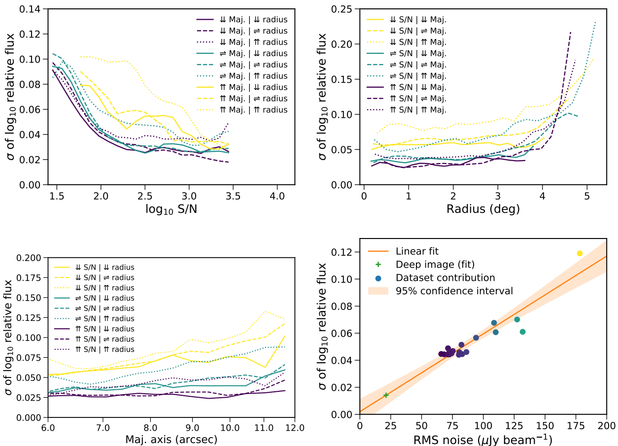
Fig. 12. Standard deviation ( \sigma ) of the logarithmic relative flux density with respect to several parameters. The upper left panel shows the relation of \sigma with respect to the signal-to-noise level for sub-samples separated in tertiles of distance from the pointing centre and major axis. The different tertiles are marked with arrow symbols in the legend: up arrows for the higher tertile, left-right arrows for the middle tertile, and down arrows for the lower one. The upper right panel shows the relation of \sigma with respect to the distance to the centre for tertiles of major axis and S/N. The lower left panel shows the relation of \sigma with respect to the major axis of the sources for tertiles of distance to the centre and S/N. The lower right panel shows the contribution of the calibration effects of the dataset ( \sigma_{dataset} , as explained in the text) with respect to the RMS noise at 2 square degrees for the individual datasets (coloured circles). The linear fit to the relation is shown as a orange line and its 95 per cent confidence interval as a shaded orange band. The extrapolated location of the final deep image is also marked in the diagram as a green cross.
