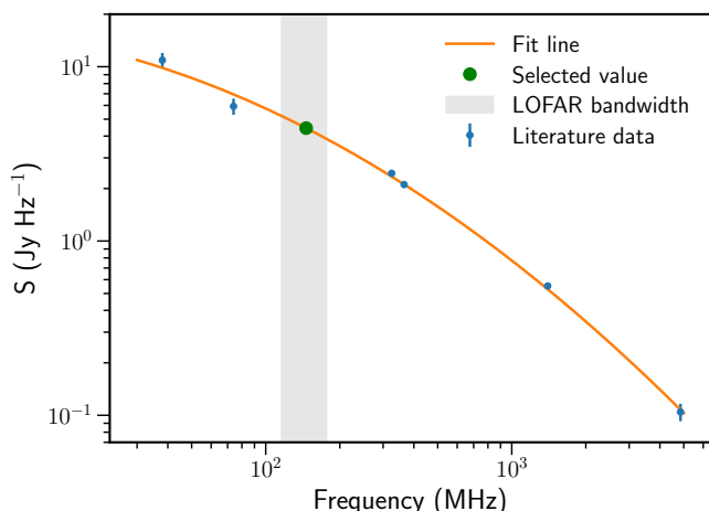
Fig. A.1. Determination of the flux density of the calibrator 87GB 160333.2+573543 in the LOFAR band using literature data. The measurements from the literature and their respective errors are shown as blue dots. The vertical grey band represents the LOFAR bandwidth of the ELAIS-N1 data. The green dot marks the value of the flux density adopted at a frequency of 146 MHz.
