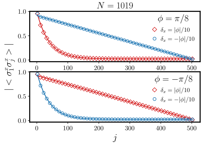
FIG. 5: (Color online) Spin correlation |\langle \sigma_1^x \sigma_j^x \rangle| as a function of the site j , for a chain made of N = 1019 spins. The defect is along the x direction. The exponential decay found for a FTD defect underlines the standard AFM order. On the other hand the linear decay for the AFTD case is a typical signature of the frustrated nature of the incommensurate AFM phase.
