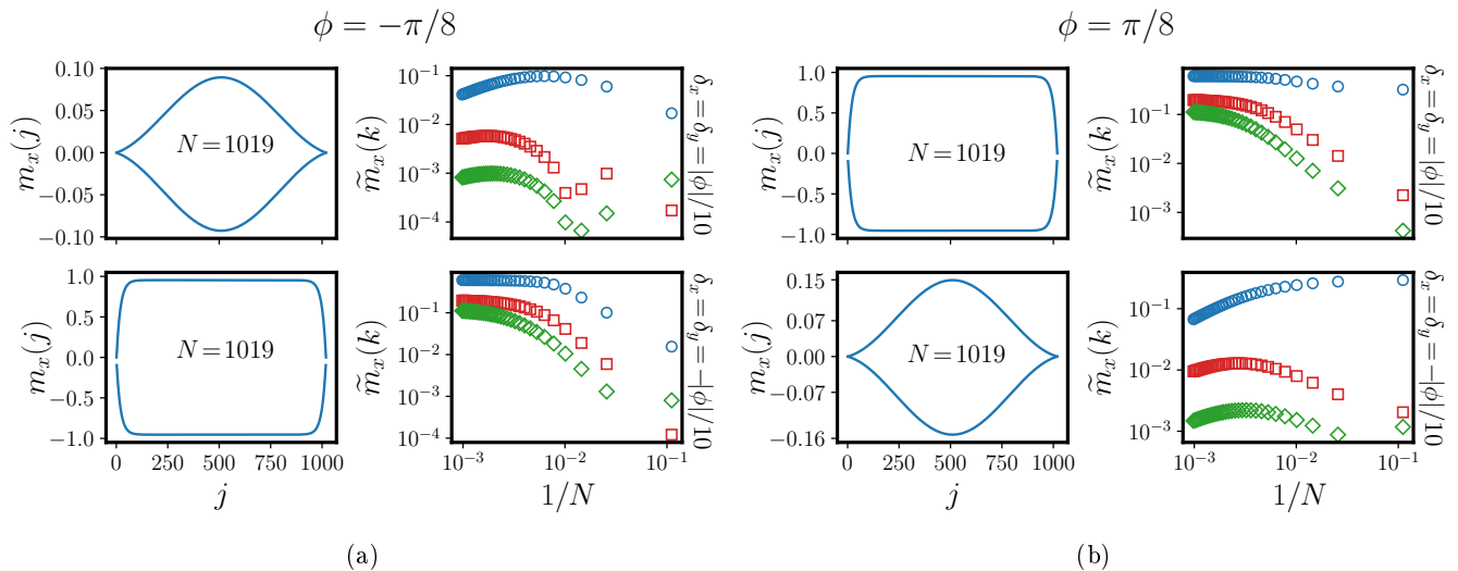
FIG. 7: (Color online) Magnetization m_x(j) = \langle \sigma_j^x \rangle as a function of the site j for a chain made of N = 1019 spins (left), and the absolute value of its Discrete Fourier Transform (DFT) in eq. (4) as a function of the inverse chain length (right), while keeping fixed the “momentum”: green diamonds |\tilde{m}_x(\frac{N+1}{2})| , red squares |\tilde{m}_x(\frac{N-1}{2})| , and blue circles |\tilde{m}_x(\frac{N+1}{2})| . The defect is along both the x and y directions. An antiferromagnetic one yields mesoscopic magnetization that varies in space with an incommensurate pattern, while a ferromagnetic defect gives standard AFM order in the bulk (see text for discussion).
