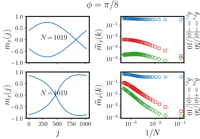
FIG. 3: (Color online). Magnetization with two bond defects, one between the first and the last spins of the chain ( \delta_{x_1} ) and the second between the \frac{N-1}{2} and the \frac{N+1}{2} spins ( \delta_{x_2} ). On the left, the magnetization m_x(j) = \langle \sigma_j^x \rangle as a function of the site j for N = 1019 and on the right the absolute value of its Discrete Fourier transform (DFT) in eq. (4) as a function of the inverse chain length, up to N = 2001 , for different momenta: green diamonds |\tilde{m}_x(\frac{N+5}{2})| , red squares |\tilde{m}_x(\frac{N+3}{2})| , and blue circles |\tilde{m}_x(\frac{N+1}{2})| . The results are obtained considering the defects only along the x direction ( \delta_{y_1} = \delta_{y_2} = 0 ). While in the case of both defect being AFTD (upper row) the DFT clearly signals the rising of a macroscopic incommensurate staggerization in which the magnetization on the j -th spin is proportional to \sin[\pi(1 - \frac{1}{N})j] , when the smaller defect is FTD the system sizes considered are not sufficient to clearly characterize the emerging order. It seems clear that at least one Fourier component remains finite as N \rightarrow \infty , indicating that the order survives in the thermodynamic limit, but the determination of the faith of the other components requires larger N 's.
