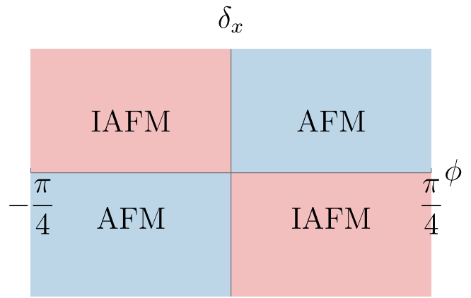
FIG. 1: (Color online) Schematic representation of the different phases as function of the system parameters. The interval (-\pi/4, \pi/4) corresponds to a dominating antiferromagnetic interaction along the x axis. When a defect of the form (\delta_x \neq 0, \delta_y = 0) favours a ferromagnetic alignment, namely when a FTD defect is considered, the effect of the defect is localized in a small region and outside of them the standard AFM order is restored. On the other hand when it tends to strengthen the antiferromagnetic interaction (AFTD) the incommensurate AFM order (IAFM) is realized.
