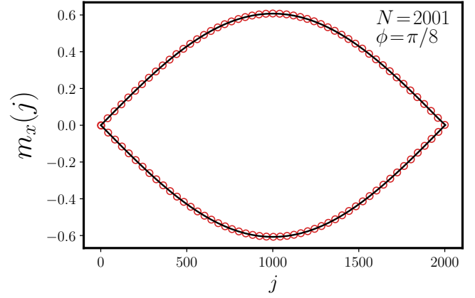
FIG. 6: (Color online) Comparison with the expression of the magnetization in eq. (10) obtained with the perturbative approach (solid black line) and the data obtained with the exact calculation (red dots) for a system made by N = 2001 spins and \phi = \frac{\pi}{8} , \delta_x = \frac{\pi}{80} .
