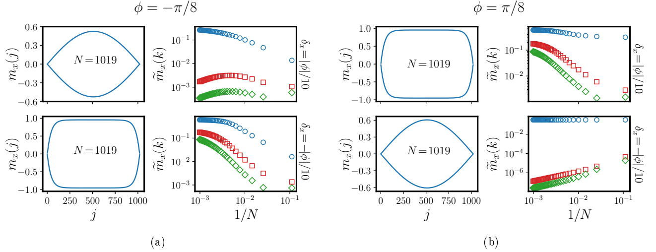
FIG. 2: (Color online) Magnetization m_x(j) = \langle \sigma_j^x \rangle as a function of the site j for a chain made of N = 1019 spins (left), and the absolute value of its Discrete Fourier transform (DFT) eq. (4) as a function of the inverse chain length, for chain lengths up to N = 2001 , (right) for different momenta: green diamonds |\tilde{m}_x(\frac{N \pm 3}{2})| , red squares |\tilde{m}_x(\frac{N \pm 5}{2})| , and blue circles |\tilde{m}_x(\frac{N \pm 1}{2})| . The results are obtained considering the defect only along the x direction ( \delta_y = 0 ). An antiferromagnetic defect yields an incommensurate AFM order, while a ferromagnetic one gives standard AFM order in the bulk (see text for discussion).
