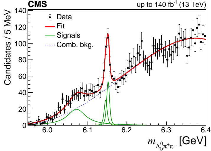
Figure 2: Invariant mass distribution of the selected \Lambda_b^0\pi^+\pi^- candidates in the high-mass region. The vertical bars on the data points represent the statistical uncertainties in the data. The overall fit result is shown by the thick solid line. The thin lines present the contributions from the two signal peaks and the broad enhancement. The dashed line displays the combinatorial background.
