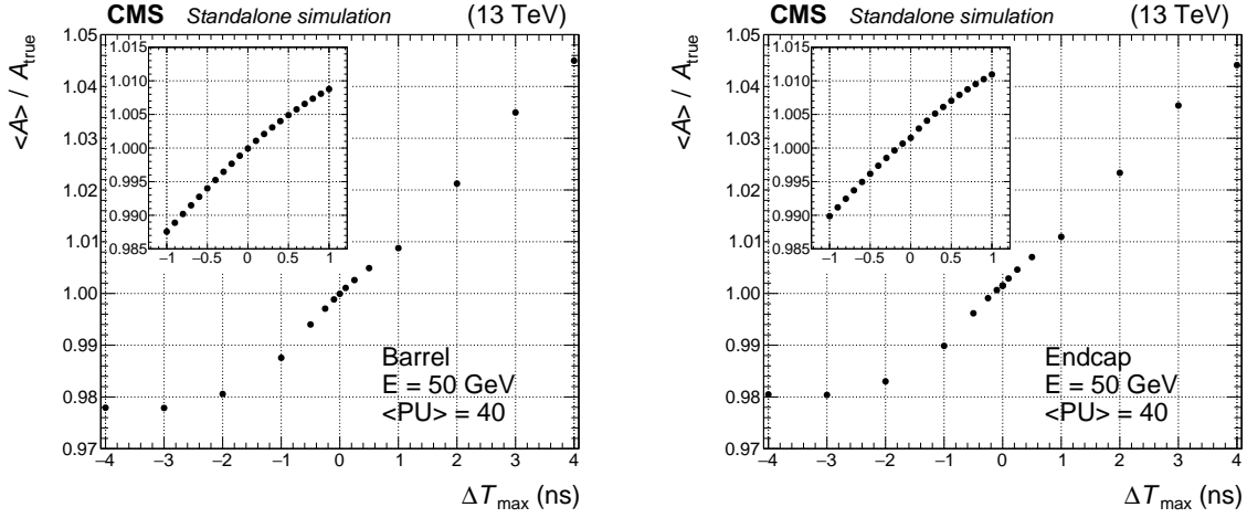
Figure 7: Reconstructed amplitude over true amplitude, \langle A \rangle / A_{\text{true}} , as a function of the timing shift of the pulse template, \Delta T_{\text{max}} , for a single-crystal pulse of E = 50 \text{ GeV} in the EB (left) and EE (right). The insets show an enlargement in the \pm 1 \text{ ns} range with a finer \Delta T_{\text{max}} granularity.
