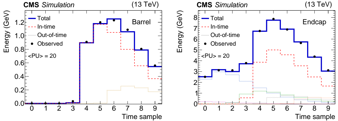
Figure 1: Two examples of fitted pulses for simulated events with 20 average pileup interactions and 25 ns bunch spacing. Signals from individual crystals are shown. They arise from a p_T = 10 GeV photon shower in the barrel (left) and in an endcap (right). In the left panel, one OOT pulse, in addition to the IT pulse, is fitted. In the right panel, six OOT pulses, in addition to the IT pulse, are fitted. Filled circles with error bars represent the 10 digitized samples, the red dashed distributions (dotted multicolored distributions) represent the fitted in-time (out-of-time) pulses with positive amplitudes. The solid dark blue histograms represent the sum of all the fitted contributions. Within the dotted distributions, the color distinguishes the fitted out-of-time pulses with different BX, while the legend represent them as a generic gray dotted line.
