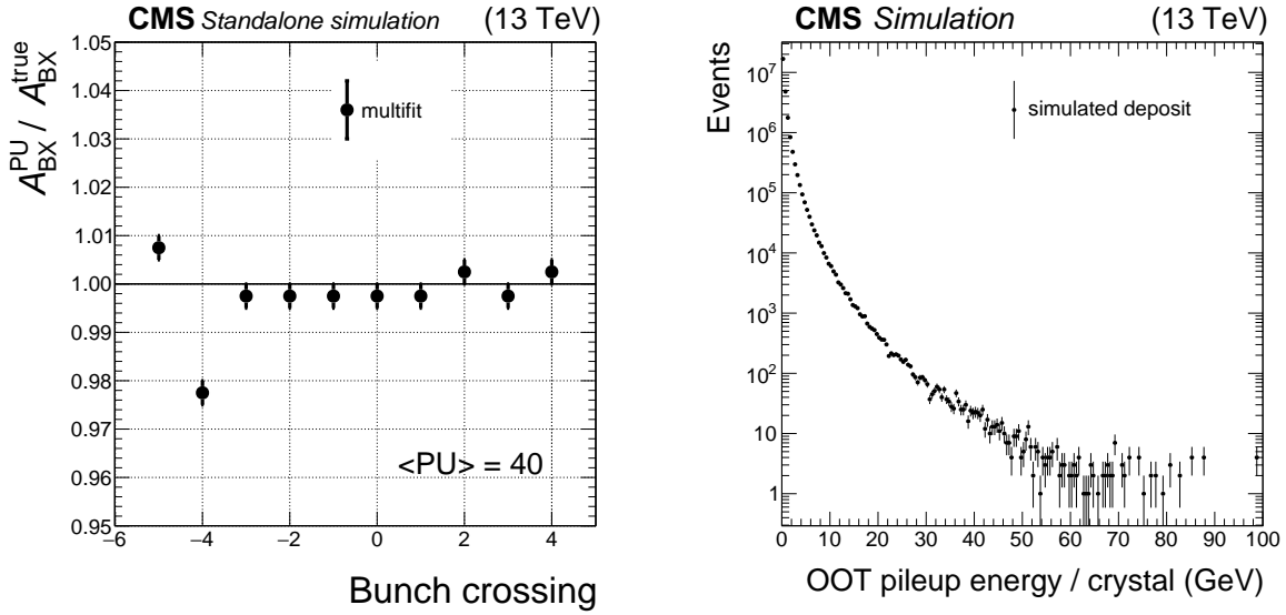
Figure 10: Left: bias in the out-of-time amplitude estimated by the multifit algorithm as a function of BX, for the bunch crossings -5 \leq \text{BX} \leq +4 . The in-time interaction corresponds to \text{BX} = 0 in the figure. The bias is estimated as the mode of the distribution of the ratio between the measured and the true energy. Only statistical uncertainties are shown. Right: energy spectrum in an ECAL barrel crystal, at \eta \approx 0 .
