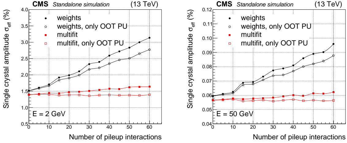
Figure 9: Measured amplitude resolution for two generated energy deposits ( E = 2 GeV or E = 50 GeV) in a single ECAL barrel crystal, at \eta = 0 , reconstructed with either the multifit or the weights algorithm. Filled points show the effective resolution expressed as the difference between the reconstructed energy and the true energy, divided by the true energy. Open points show the percent resolution estimated when the true energy is replaced with the sum of the true energy and the in-time pileup energy.
