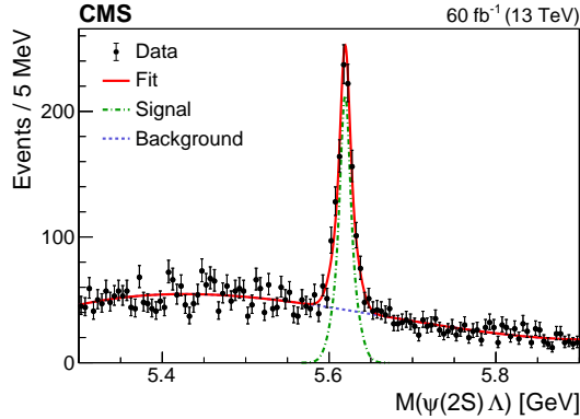
Figure 2: The invariant mass distribution of \Lambda_b^0 \rightarrow \psi(2S)\Lambda candidates. The points are the data and the lines give the result of the fit described in the text.
