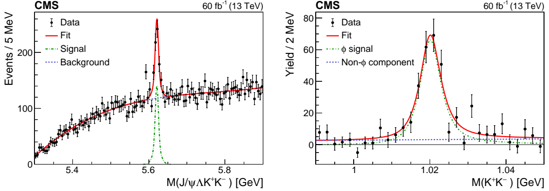
Figure 1: The invariant mass distributions of (left) J/\psi\Lambda K^+K^- and (right) background-subtracted K^+K^- . The points are the data, with the vertical bars giving the statistical uncertainties, and the lines show the results of the fits described in the text.
