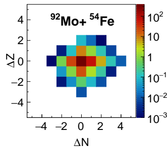
Figure 3. GRAZING calculated cross section for the target-like products in the ^{92}\text{Mo}+^{54}\text{Fe} collision at 370 MeV.
