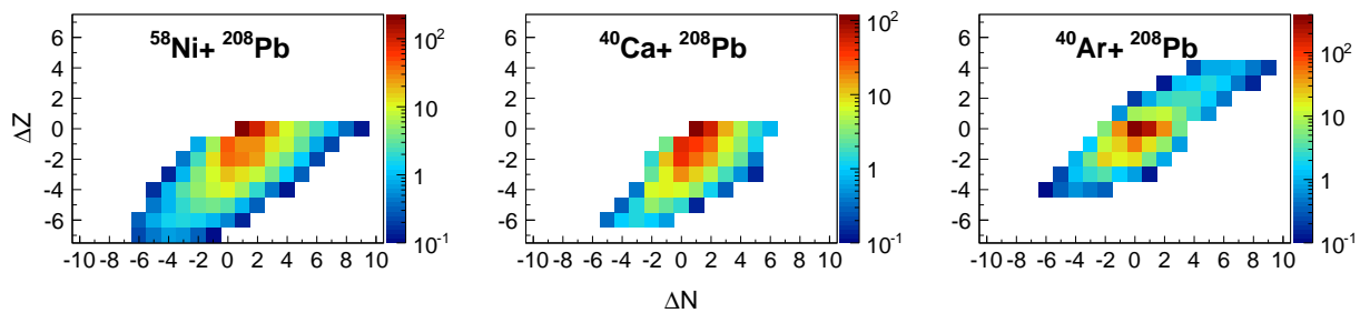
Figure 1. Angle and energy integrated total cross section for ^{40}\text{Ar} , ^{40}\text{Ca} , and ^{58}\text{Ni} projectiles on the ^{208}\text{Pb} target, at energies E_{\text{lab}} = 6.4, 6.2, and 6 MeV/A, respectively. The cross section values of the elastic (+inelastic) channel have been scaled down by a factor 100 to better display the behavior of the transfer channels [3].
