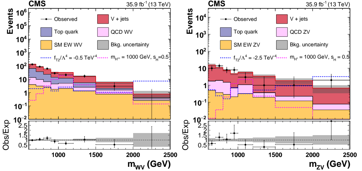
Figure 4: Distributions of m_{WV} (left) and m_{ZV} (right) in the signal region. The gray bands include uncertainties from the predicted yields. The histograms for other backgrounds include the contributions from QCD VV, top quark, W+jets, and Drell–Yan processes. The predicted yields are shown with their best-fit normalizations from the background-only fit. The dashed lines show the signal predictions for two aQGC parameters, and charged Higgs bosons in the GM model. The overflow is included in the last bin. The bottom panel in each figure shows the ratio of the number of events observed in data to that of the total background prediction.
