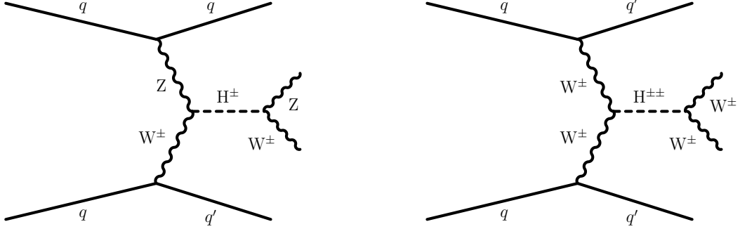
Figure 2: Examples of Feynman diagrams showing the production of singly (left) and doubly (right) charged Higgs bosons via VBF.
