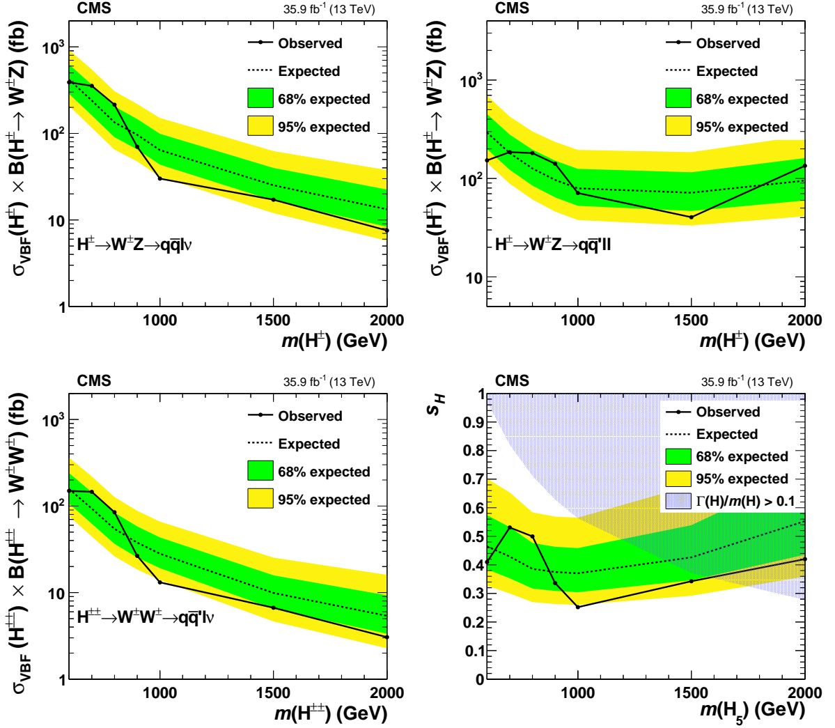
Figure 5: Expected and observed exclusion limits at the 95% CL as a function of m(H^\pm) for \sigma_{\text{VBF}}(H^\pm) \mathcal{B}(H^\pm \rightarrow W^\pm Z) in the WV (upper left) and ZV (upper right) final states, for \sigma_{\text{VBF}}(H^{\pm\pm}) \mathcal{B}(H^{\pm\pm} \rightarrow W^\pm W^\pm) , as a function of m(H^{\pm\pm}) (lower left), and for s_H in the GM model (lower right). The blue shaded area covers the theoretically disallowed parameter space [76].
