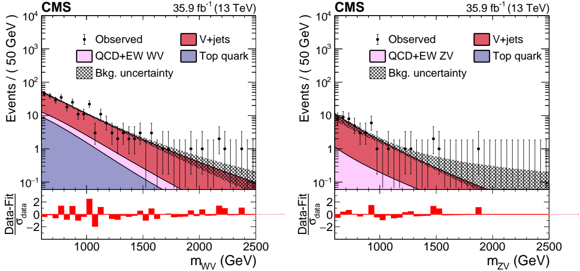
Figure 3: Comparison between the fit results for the V+jets background processes and the data distributions of the m_{WV} (left) and m_{ZV} (right), respectively, in the sideband region with 40 < m_V < 65 GeV or 105 < m_V < 150 GeV. The fit uncertainty is shown as a shaded band.
