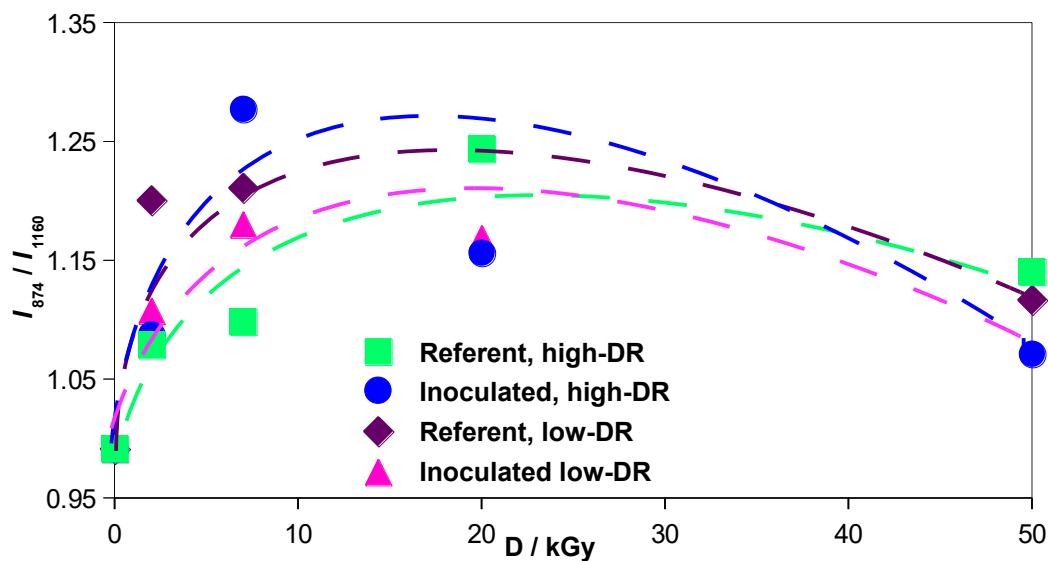
Fig. 6. Absorbed dose dependence of FTIR intensity ratio of carbonate anion absorption at 874\text{ cm}^{-1} to pyranose ring absorption at 1160\text{ cm}^{-1} for irradiated inoculated and referent paper samples.
