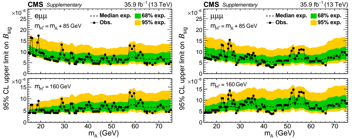
Figure A.3: Upper limits at 95% CL on B_{\text{sig}} for the 95 m_A values, with an assumption of m_{H^+} = m_A + 85 \text{ GeV} (upper) or m_{H^+} = 160 \text{ GeV} (lower), for individual final states (left: e\mu\mu and right: \mu\mu\mu final states). In the calculation, the same value of \sigma(t\bar{t}) as in Fig. A.2 is assumed.
