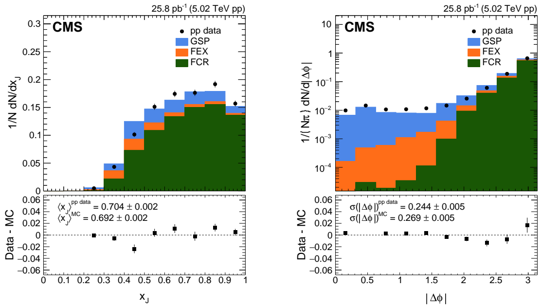
Figure 8: The distributions of x_J (left) and \Delta\phi (right) in pp collisions after flavor process reweighting. Data are shown in solid points, while the stacked histograms show the contributions of different processes in PYTHIA 6 (see text for details). The bottom set of panels show the difference between data and simulation (MC).
