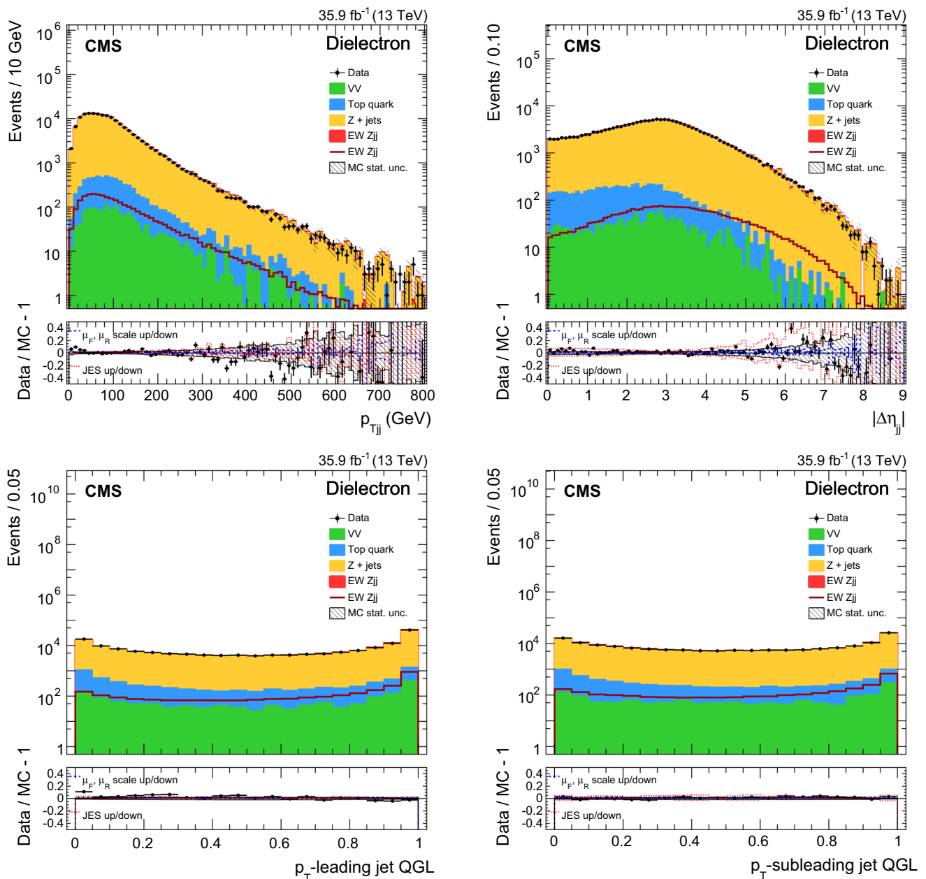
Fig. 5 Data and simulated event distributions for the dielectron event selection: dijet system transverse momentum (top left), dijet pseudorapidity opening (top right), p_{T\text{-leading jet QGL}} (bottom left), and p_{T\text{-subleading jet QGL}} (bottom right). The contributions from the different background sources and the signal are shown stacked, with data points
