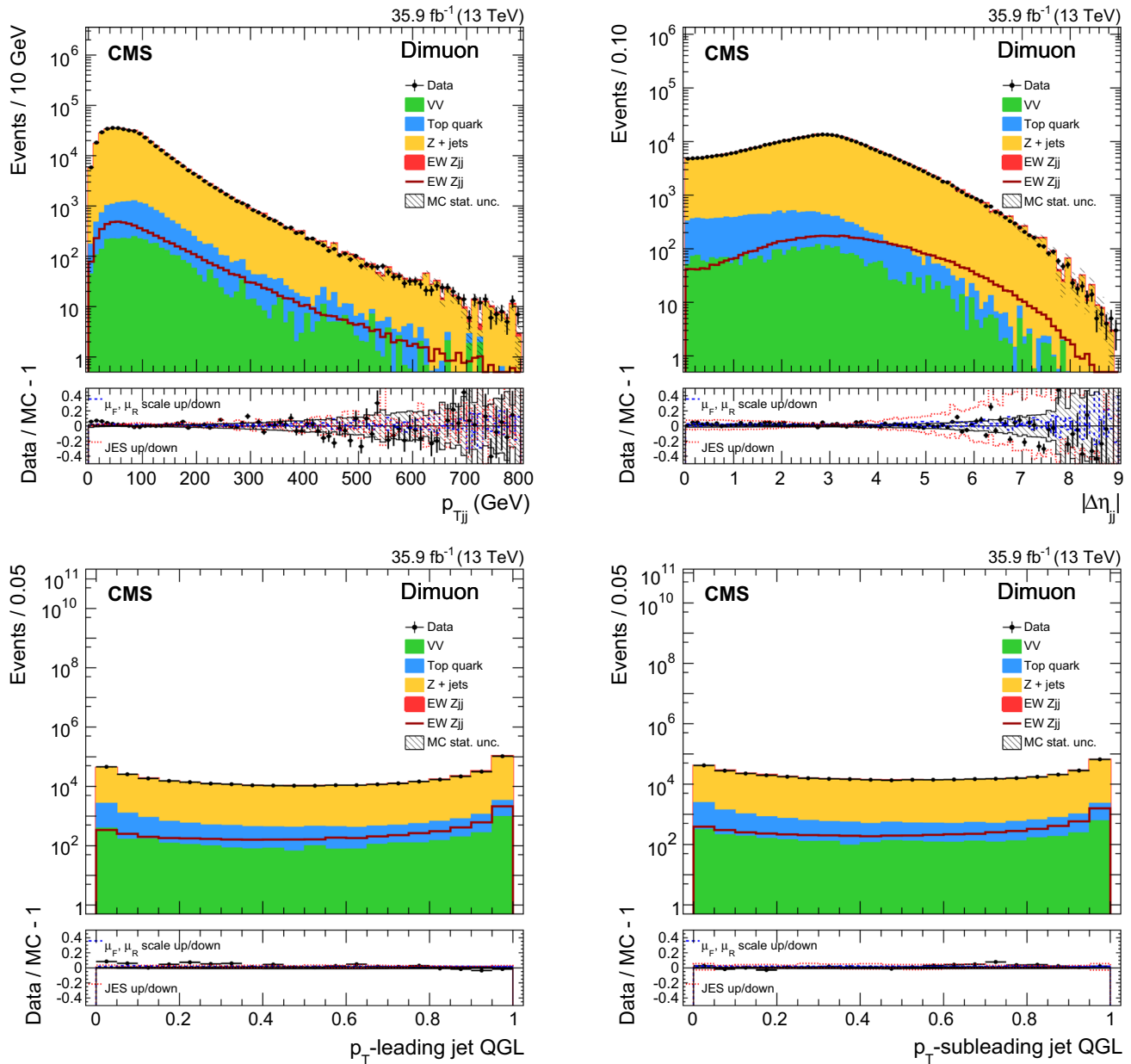
Fig. 6 Data and simulated event distributions for the dimuon event selection: dijet system transverse momentum (top left), dijet pseudorapidity opening (top right), p_{T\text{-leading jet QGL}} (bottom left), and p_{T\text{-subleading jet QGL}} (bottom right). The contributions from the different background sources and the signal are shown stacked, with data points
